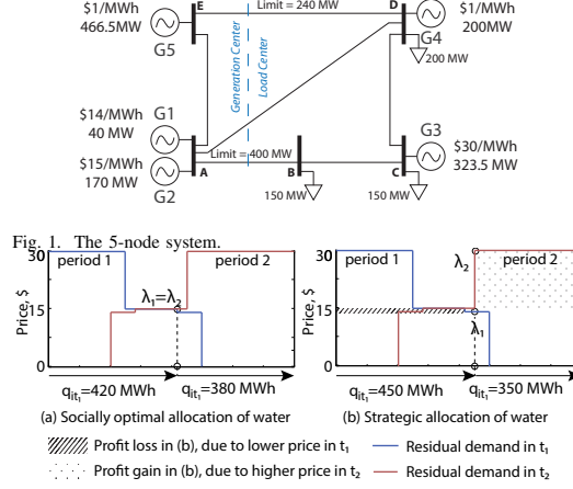
Fig. 2. The effect of relocation of water in time by hydropower producer.
