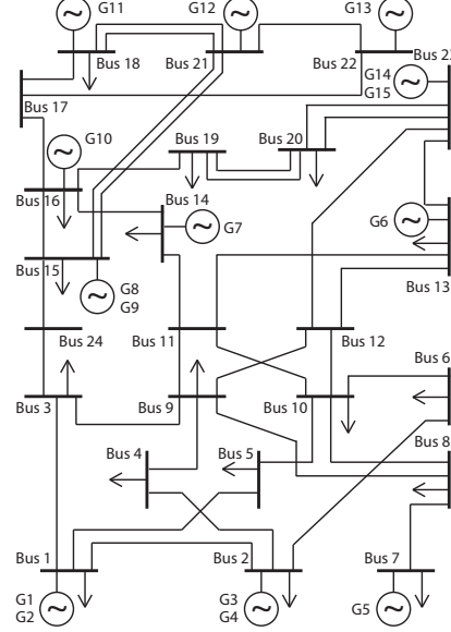
Fig. 4. The IEEE 24-nodes example system.
