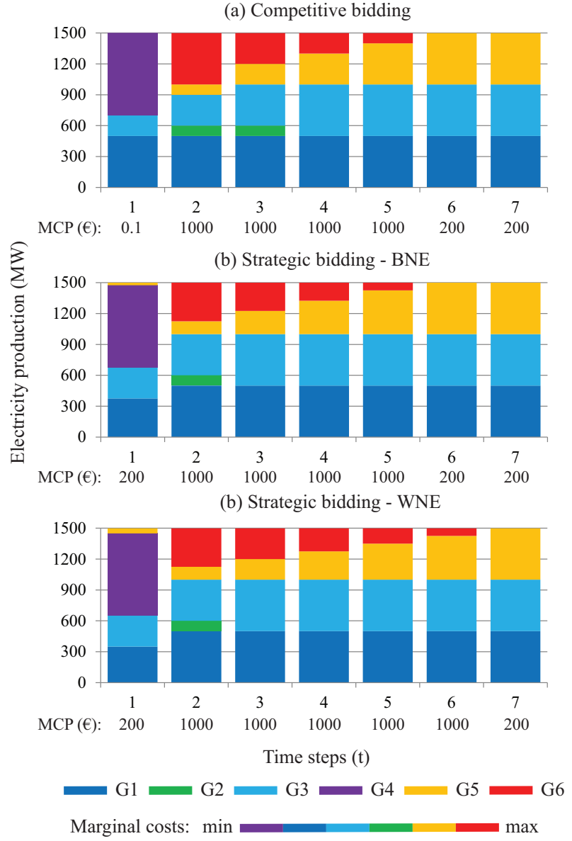
Figure 4.1: Short-run economic dispatch and market clearing prices (MCPs) for the cases of (a) competitive and (b) strategic bidding. BNW: best-Nash equilibrium case, WNE: worst-Nash equilibrium case.
