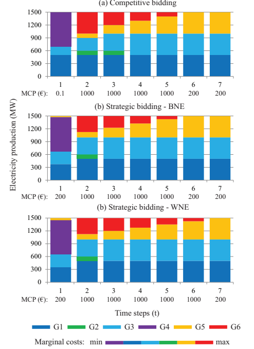
Fig. 2. Short-run economic dispatch and market clearing prices (MCPs) for the cases of (a) competitive and (b) strategic bidding. BNE: best-Nash equilibrium case, WNE: worst-Nash equilibrium case.
