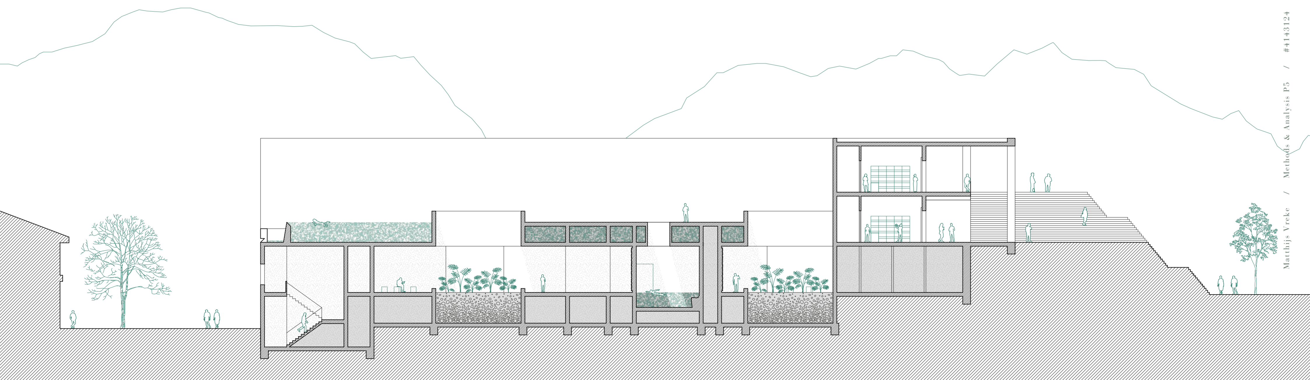
Section / 1:200
