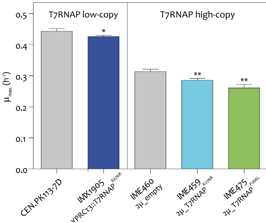
Figure 2.3. Physiological characterization of S. cerevisiae strains expressing T7RNAP. Maximum specific growth rates ( \mu_{max} ) of S. cerevisiae constitutively expressing T7RNAP K276R , Spycas9 , and Fncas12a (IMX1905) and the control strain (CENPK.113-7D), or S. cerevisiae strains overexpressing T7RNAP K276R (IME459) or T7RNAP P266L (IME475) and the control strain carrying a 2 \mu m multi-copy empty vector (IME460). All strains were cultivated on a 96-well plate containing chemically defined medium supplemented with glucose as the sole carbon source (SMD for CENPK.113-7D or IMX1905; SMD-urea with hygromycin B for IME459, IME475, or IME460; the slower growth rate measured for strains with plasmids compared to strains with genomic integration is explained by the difference in medium composition). Data points represent average and mean deviations of four biological replicates. * p < 0.025 ; ** p < 0.001 . Student's t-test was calculated compared to respective control strains CENPK.113-7D or IME460.
