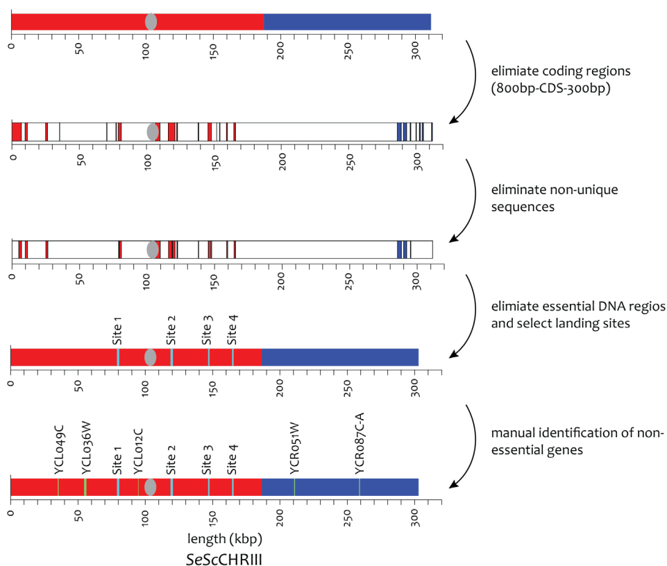
Figure 4.3. Strategy to identify non-coding unique DNA sequences in S. pastorianus CBS 1483 SeScCHRIII. In the first step, non-coding regions were obtained by subtracting the coding sequences plus 800 bp upstream and 300 bp downstream covering for promoter and terminator regions. In the second step, the unique regions were obtained by selecting unique k -mers when aligning to the CBS 1483 genome and the non-unique sequences were eliminated. In the next step, the non-coding unique sequences were checked for the presence of essential DNA regions. Additionally, potential landing sites identified by manual screening of non-essential genes were selected, resulting in a total of nine landing sites.
