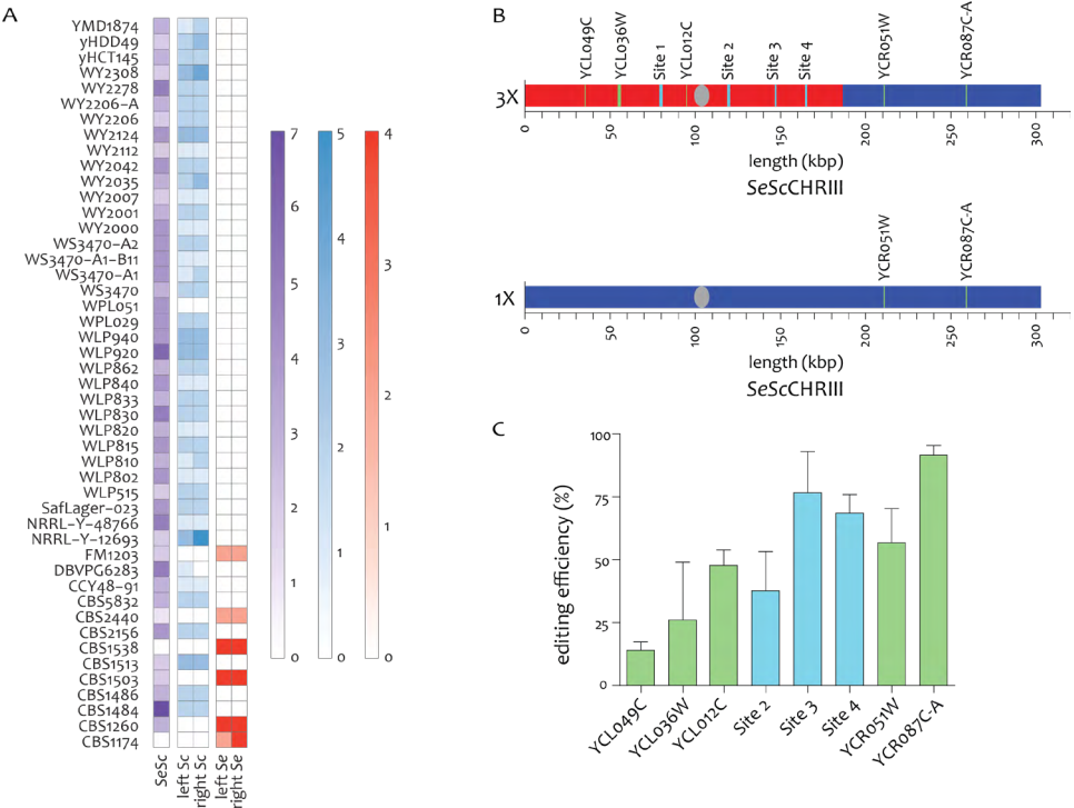
Figure 4.5. A) Overview of CHRIII genetic configurations in 47 different S. pastorianus strains. B) Chromosome III configurations in S. pastorianus WS 34/70. In comparison to CBS 1483, WS 34/70 has an additional ScCHRIII and one less hybrid SeScCHRIII. C) Genome editing efficiencies in S. pastorianus WS 34/70 targeting the identified landing sites thereby aiming for ymNeongreen integration. Editing efficiencies were calculated based on number of green fluorescent colonies over the total number of colonies on the transformation plates. Values are derived from three individual transformations.
