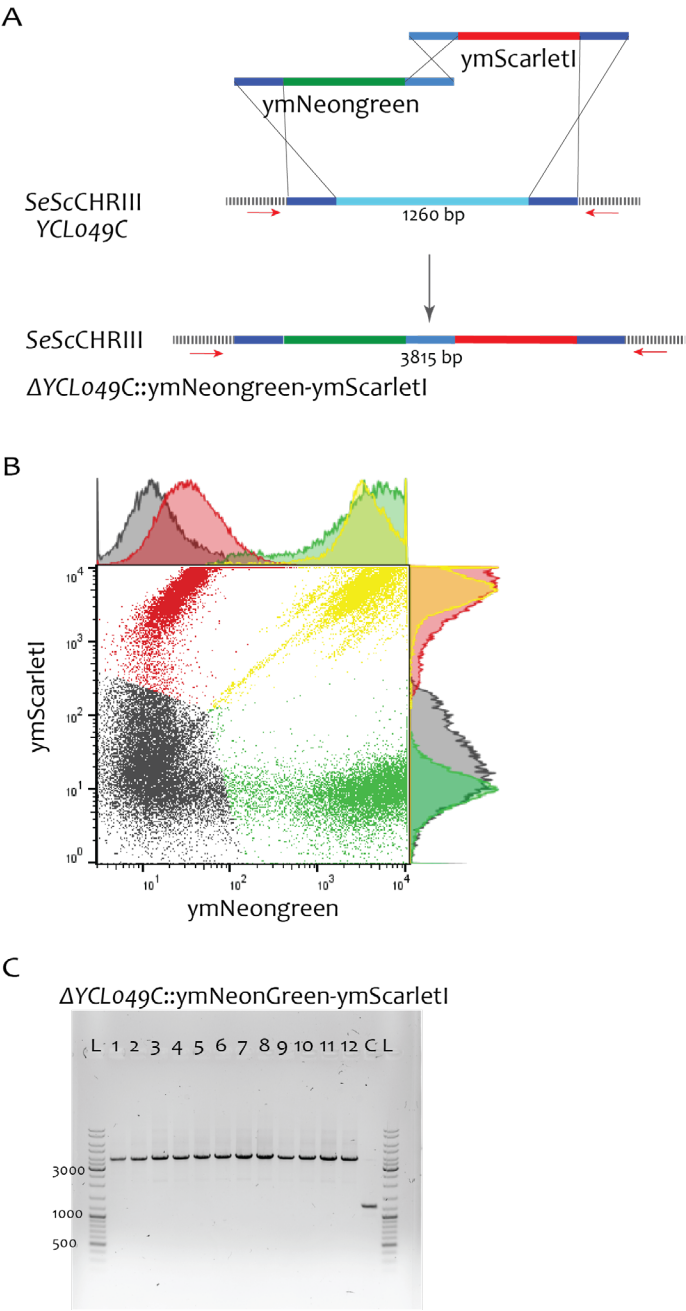
Figure 4.8. Genomic integration into landing site SeYCL049C of two in vivo assembled DNA fragments expressing ymNeongreen and ymScarletI. A) Schematic overview of the genomic integration strategy for in vivo assembly of ymNeongreen and ymScarletI DNA fragments. B) Fluorescent profile of the transformed population when aiming for integration of two fluorescent expression cassettes. The fluorescence corresponding to ymNeongreen and ymScarletI is plotted for 100.000 events. Flow cytometry was performed for three biological replicates; one representative replicate is shown. C) Genotyping of the sorted ymNeongreen + ymScarletI + single colony isolates.
