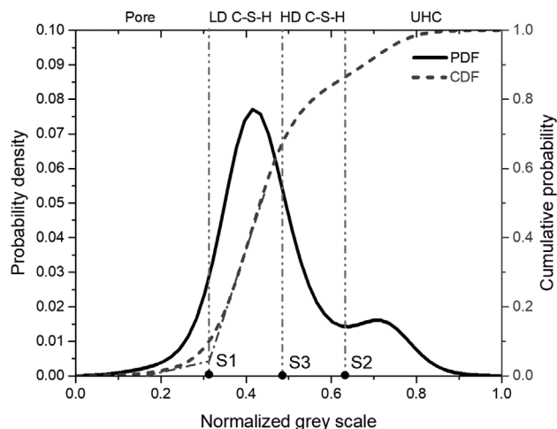
FIGURE 3 Image segmentation through gray scale histogram of CT images
