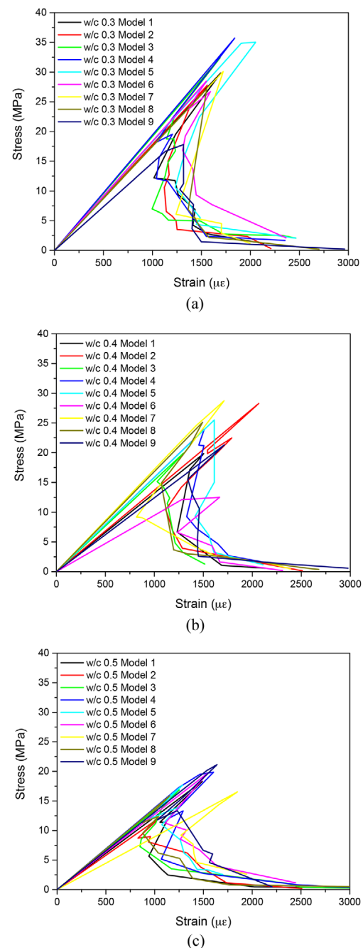
FIGURE 9 The simulated stress–strain responses for (a) w/c 0.3, (b) w/c 0.4, and (c) w/c 0.5
