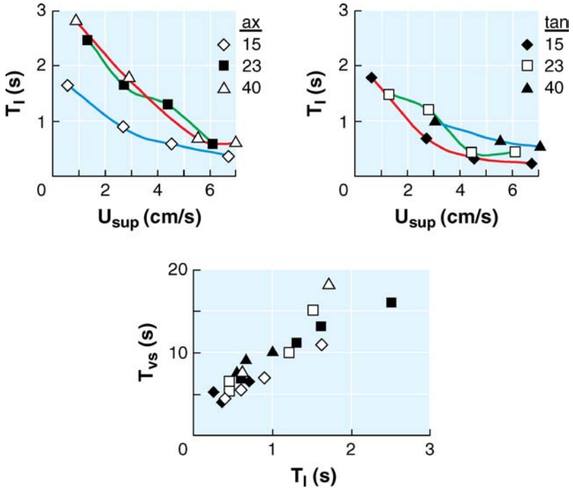
Figure 12 Dependence on the superficial gas velocity of integral timescale, T_I , and of the vortical structures, T_{vs} (from Groen 2004).
