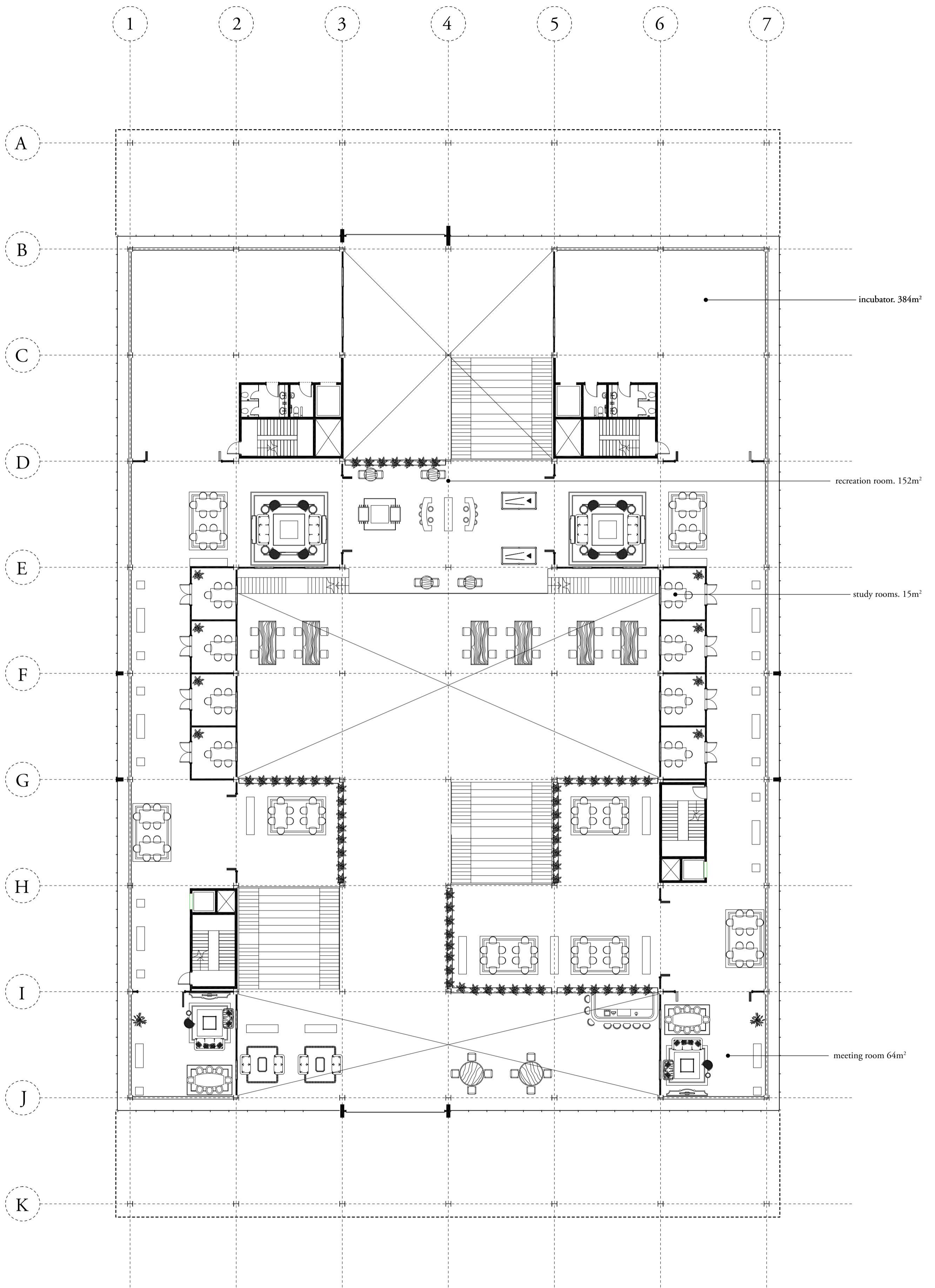
collaboration. first floor. 1:200
