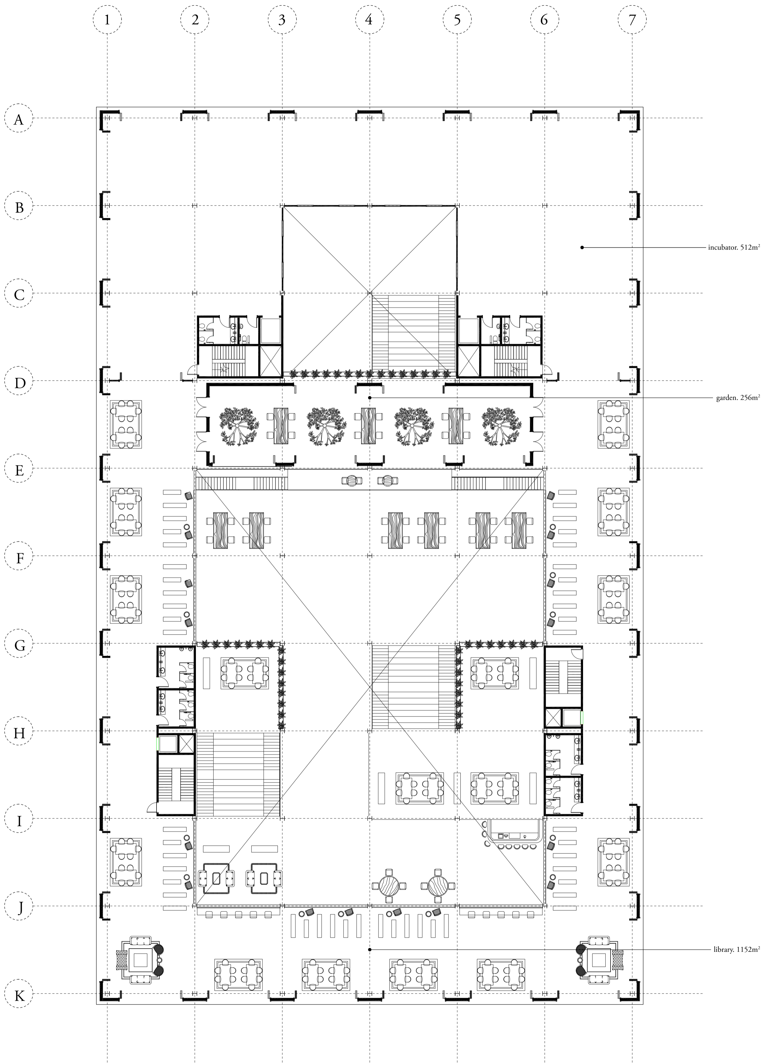
consumption. second floor. 1:200
