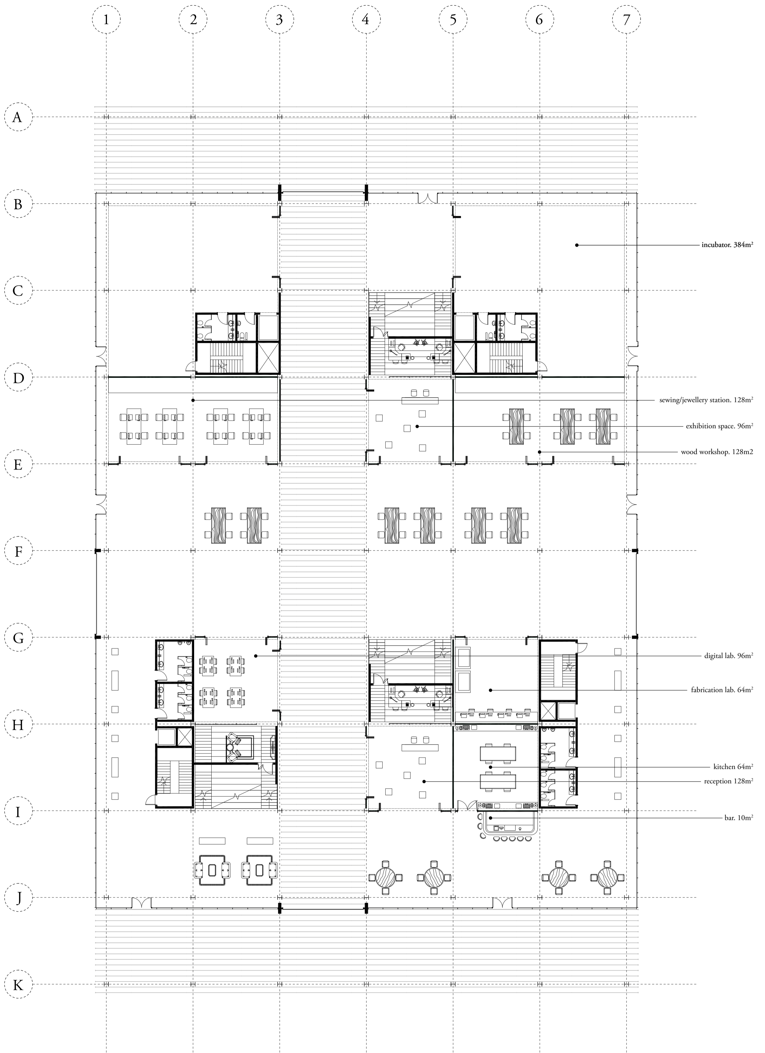
creation. ground floor. 1:200
