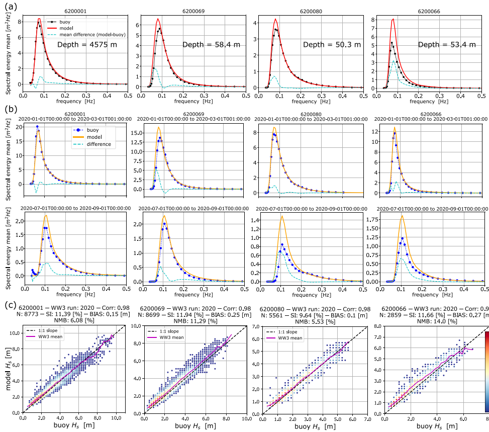
Fig. 10. (a) Spectral energy mean comparison for 2020 at buoys 6200001, 6200069, 6200080 and 6200066. (b) Same as (a) but for January–February (top panel) and July–August (bottom panel). (c) Scatter plot and performance parameters of H_s . Colorbar in (c) indicates normalized occurrences in % (N is the total amount of model-buoy time-matched data).
