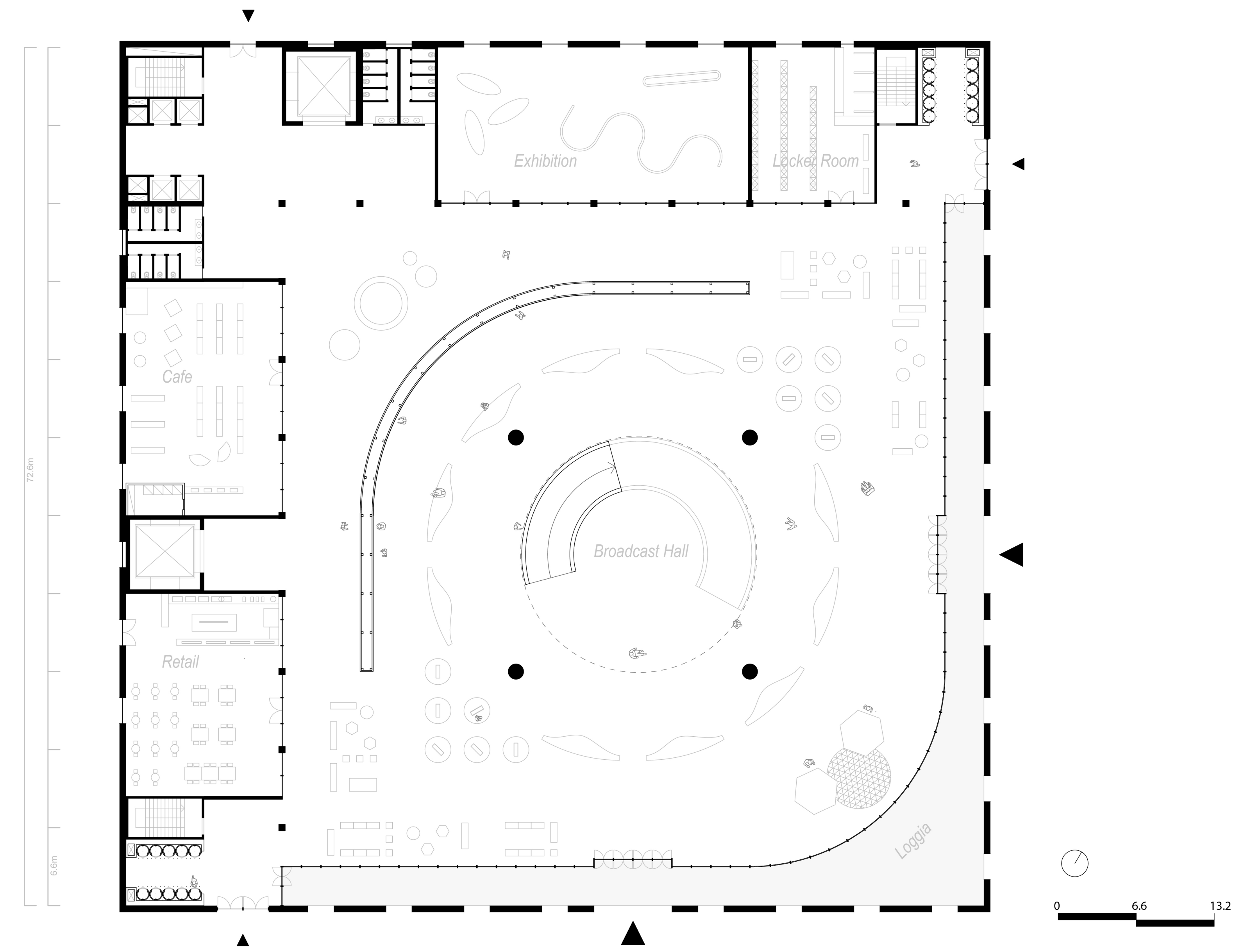
1-250 Ground Floor
