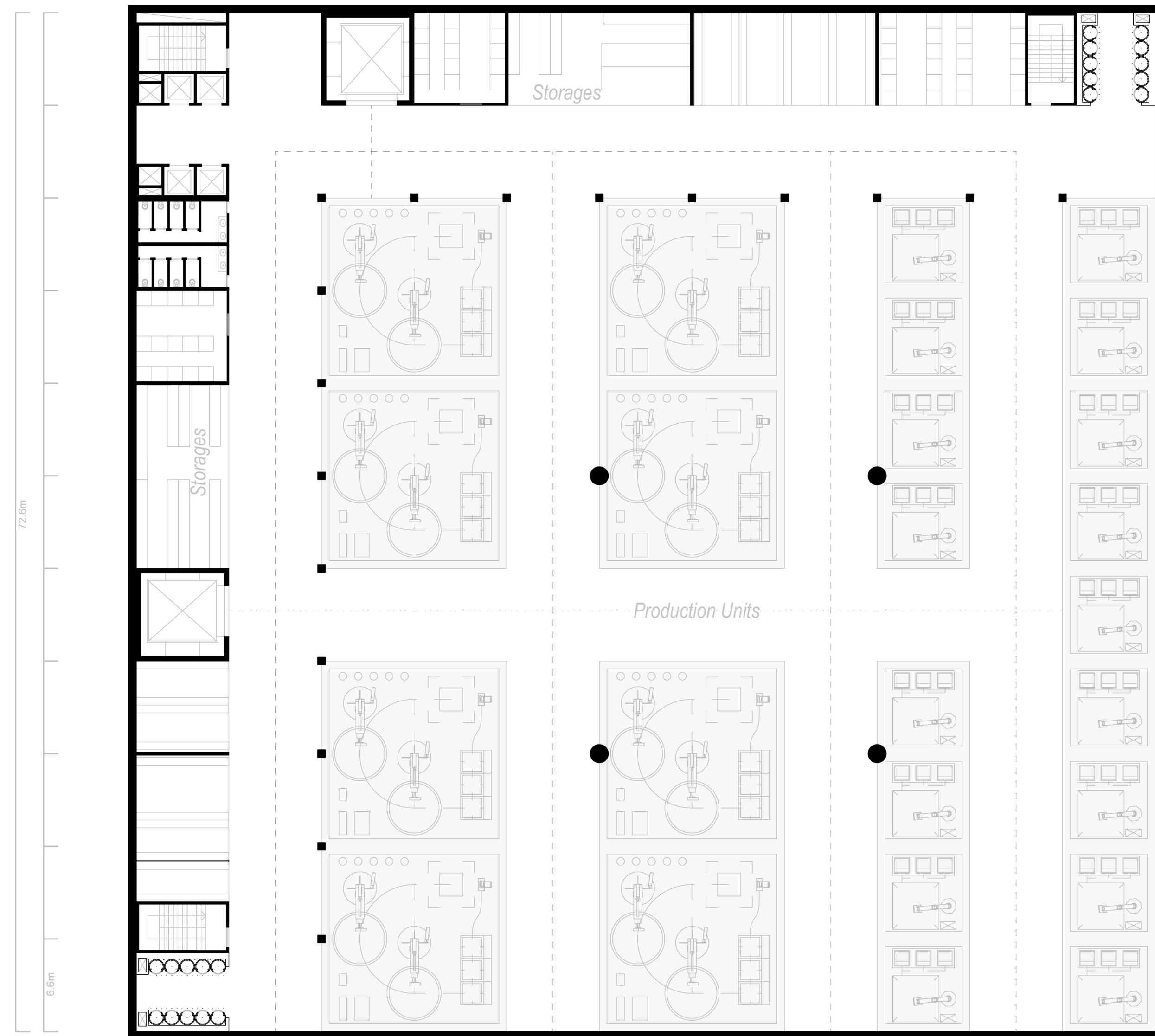
1-250 Underground
