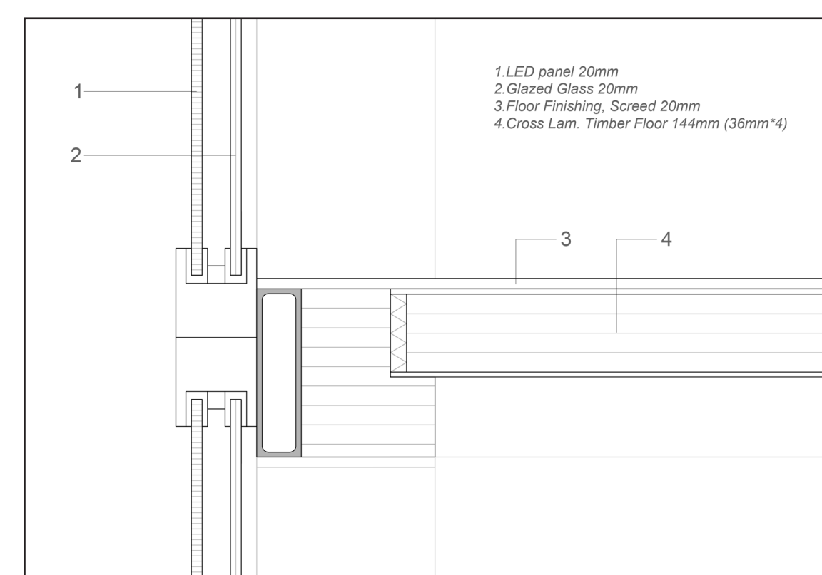
D-06 Internal Led Panels 1:10
