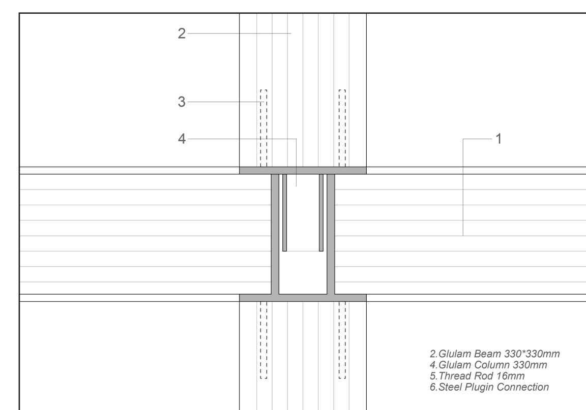
D-07 Joint between Column and Beam 1:10
