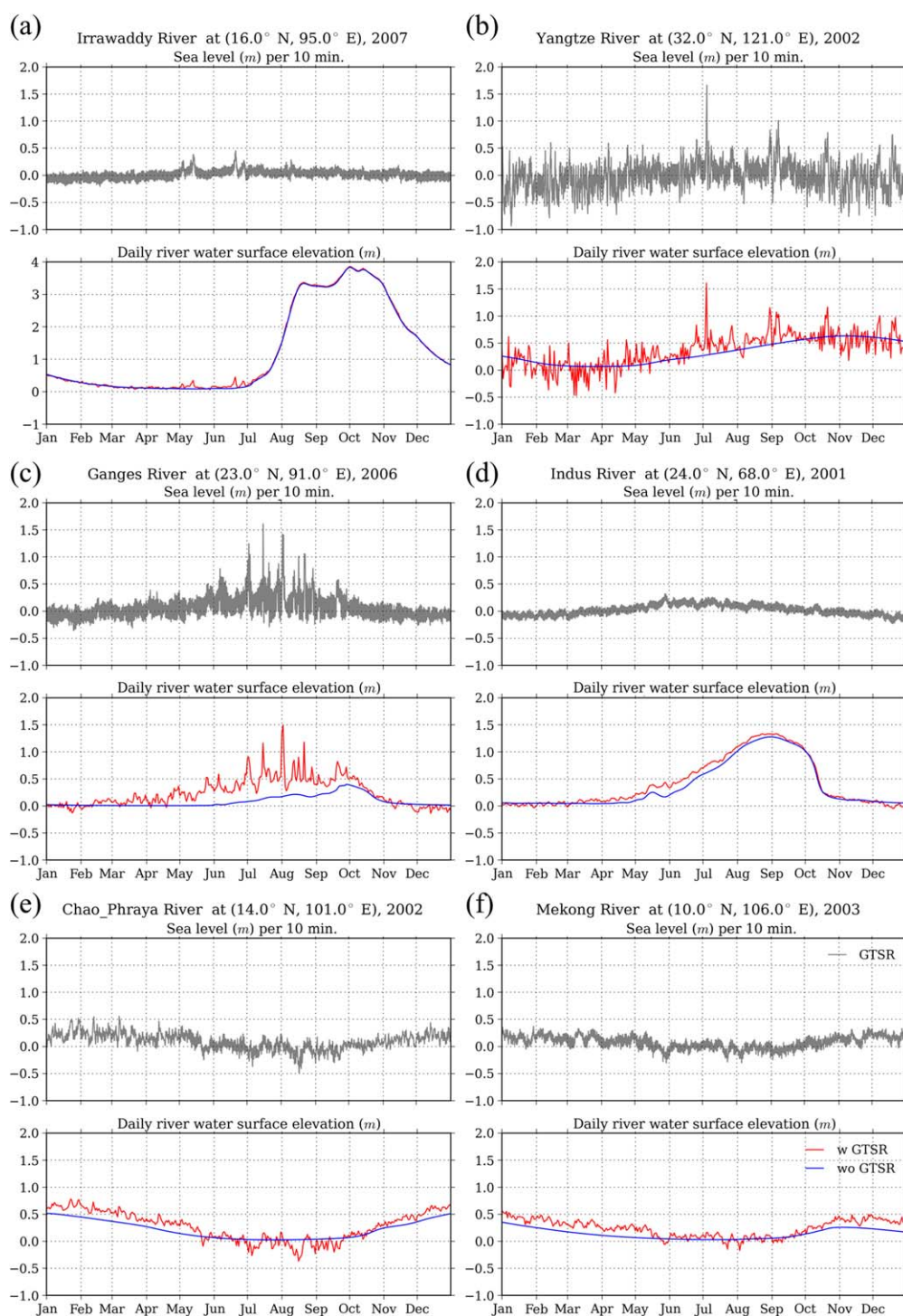
Figure 2. Input water levels (m) per 10 min at river mouths (gray lines in upper parts) and water surface elevation (m) modeled by CaMa-Flood with and without GTSR (red and blue lines in lower parts) in six Asian rivers: (a) Irrawaddy River, (b) Yangtze River, (c) Ganges River, (d) Indus River, (e) Chao Phraya River, and (f) Mekong River. Each plot shows water levels in different years, which are indicated in the respective titles.
