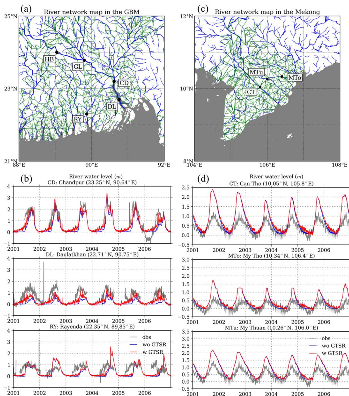
Figure 3. (a) The river network map in CaMa-Flood and gauging stations (CD, DL, and RY) used for validation in the GBM Delta. Blue and green lines indicate main river channels and bifurcation river channels, respectively. Names and locations for each station are denoted in Figure 3b. Two other stations (HB and GL) are indicated in Figure 7. (b) Validation of water levels (m) simulated by the CaMa-Flood coupled with GTSR at three stations in the GBM Delta. Gray, blue, and red lines indicate observations, CaMa-Flood simulations without GTSR, and with GTSR, respectively. Gaps in gray lines indicate missing values. (c) Same as Figure 3a but for the Mekong Delta. (d) Same as Figure 3b but for the Mekong Delta.
