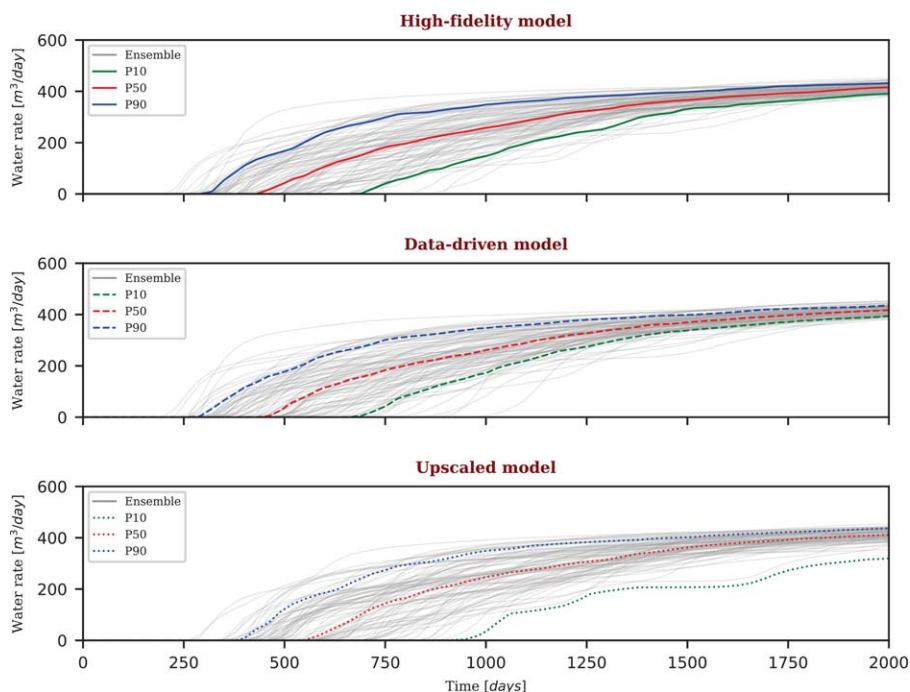
Fig. 3—Total water rate for the high-fidelity (reference) model with the size of the 100 \times 100 gridblock for the hundred Flumy realizations, together with the responses of data-driven and upscaled models ( 10 \times 10 ). Gray lines indicate the rates from a single-model realization, whereas the red, blue, and green lines indicate the quantile response of the ensemble (i.e., the P10, P50, and P90).
