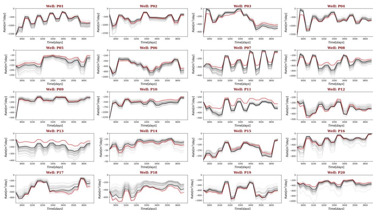
Fig. 10—Oil production rates obtained with the history-matched data-driven proxy model. Gray lines are oil production rates from multiple prior realizations of the proxy model, the black line is a true response, and the red line is the history-matched estimated data-driven proxy response.
