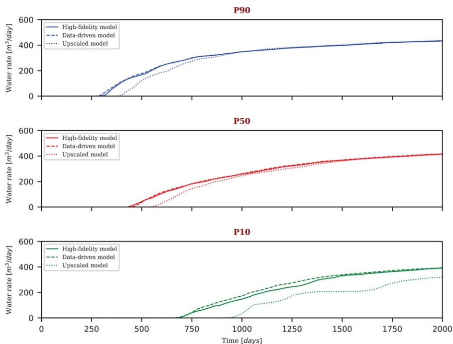
Fig. 4—P10, P50, and P90 quantile response of the high-fidelity (reference), data-driven, and upscaled models for 100 Flumy realizations.
