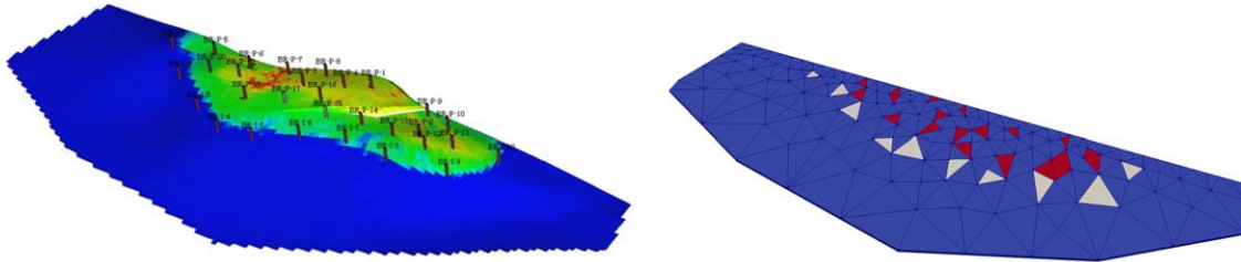
Fig. 7—(a) High-fidelity Brugge model used to generate the true model response ( 139 \times 48 \times 9 gridblocks). (b) Unstructured proxy model mesh with 283 elements: Red cells indicate a producing well, and white cells indicate an injection well.
