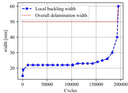
(b) Long fatigue life (specimen s3)
