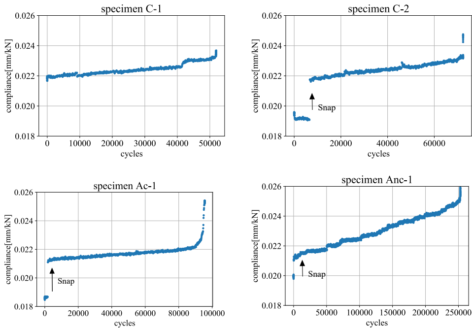
Figure 3.2: Stiffness degradation illustrated through compliance increase in different specimens
