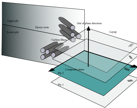
Figure 1.1: A simplified scheme of CFRP, showing plies having different fiber orientations stacked one on top of each other to form a layup
