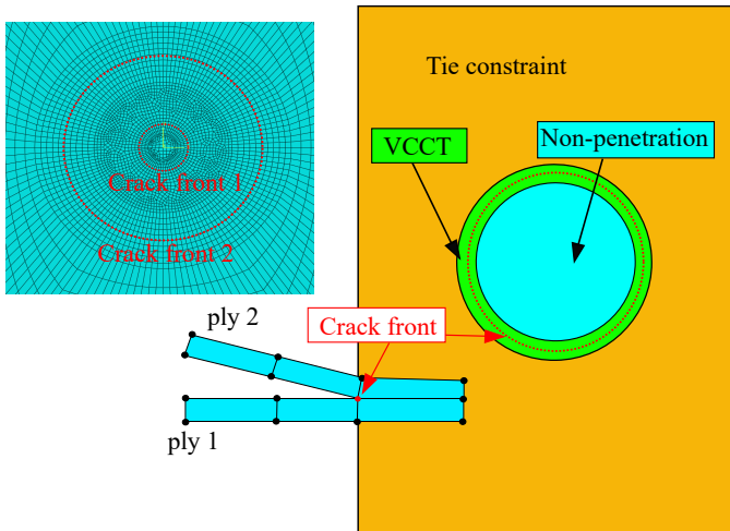
Figure 4.3: Scheme of the modeling approach adopted for the interfaces between plies and mesh in case of circular and annular delamination
