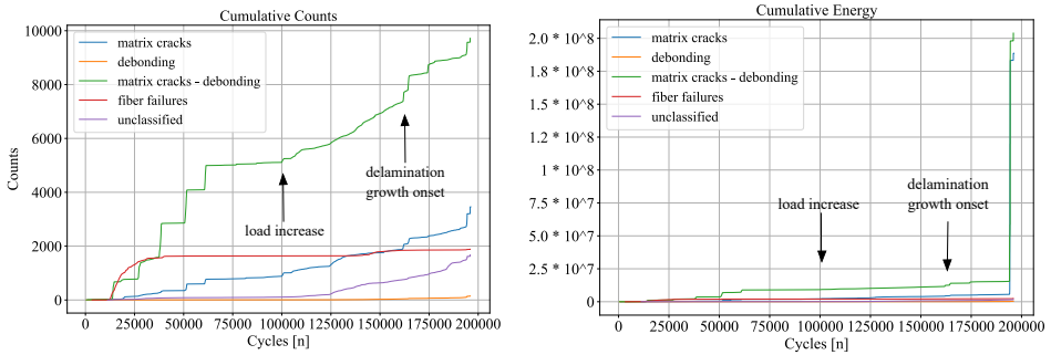
Figure 7.7: Damage modes repartition plots in specimen s3 (long life). In the left plot, the progression of cumulative count in fatigue life is shown for every damage mode. On the right the cumulative signal energy (defined in Table 5.2) is shown for every damage mode.
