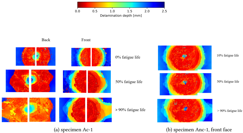
Figure 3.6: Ultrasound scan at different stages of fatigue life in specimen Ac-1 and Anc-1. The results show the propagation of several delaminations at multiple depth locations in the case of specimen Ac-1 and the propagation of delaminations close to the back face in specimen Anc-1. Growth happened in the perpendicular to the loading direction.
