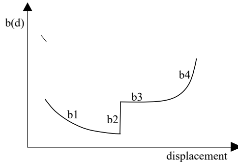
Figure 6.2: b-value/displacement plot. The possible trends that can be found in actual tests are shown
