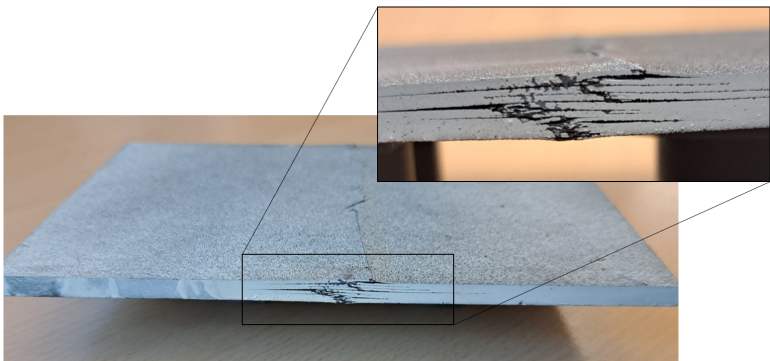
Figure 2.7: Failed specimen in compression fatigue after impact test showing signs of delamination, sublaminates buckling and fiber kinking
