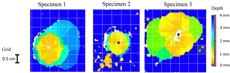
Figure 6.3: Close-up C-scan images of the impacted specimens, showing multiple delaminations at different depths. The images are cropped to show the full delamination; the impact contact point was always in the center of the specimen
