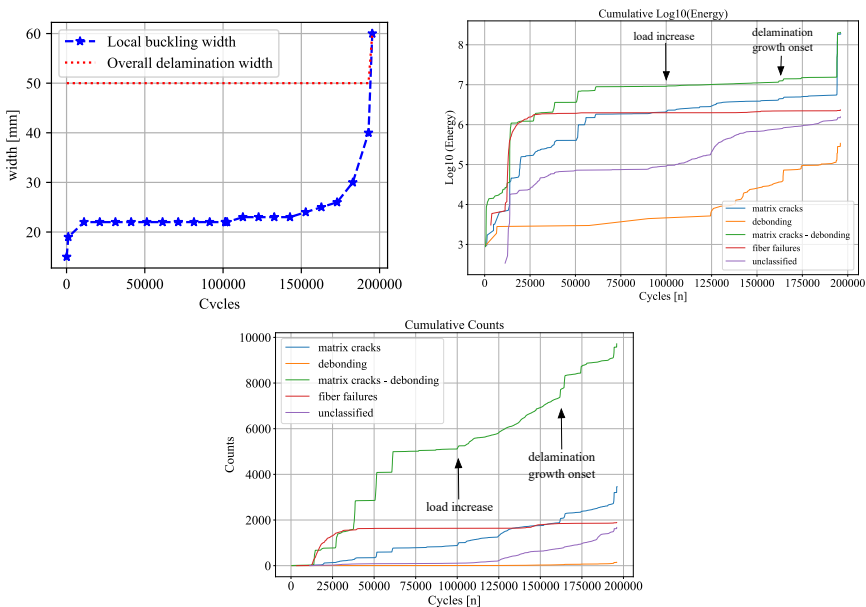
Figure 7.9: Specimen s3 delamination propagation evaluated indirectly with DIC buckle size on the left (Chapter 2), the logarithmic plot of the acoustic signal energy released by the different damage modes, and the cumulative sum of events associated to the different damage modes
