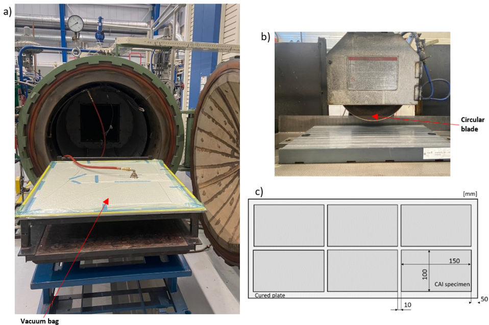
Figure 2.1: Images from the manufacturing of the laminate showing a) the autoclave and the vacuum bag containing CFRP plates, b) the diamond saw used to cut the specimens, c) the scheme of the cuts.
