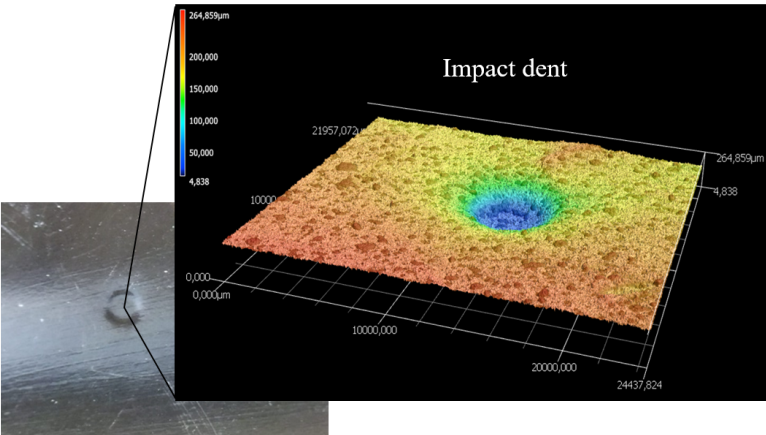
Figure 2.5: Impact dent photo and profile of the dent obtained with optical microscopy showing a dent depth < 0.3 mm
