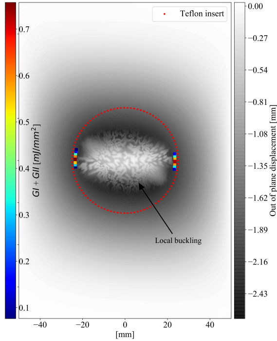
Figure 4.6: Buckling area matching SERR profiles. In color, the maximum SERR G_{max} values in the penultimate interface (where the higher values were observed). In the gray scale, the magnitude of out of plane displacement of the upper ply to this specific interface shows an elliptical local buckle.
