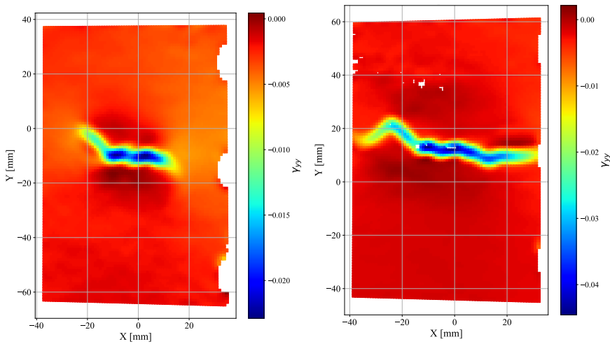
(a) sp 1 at 0% and 90% of fatigue life. Initial projected delamination width (x-direction) = 50 mm
