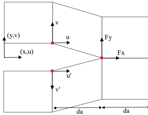
Figure 4.2: The VCCT technique schematic
