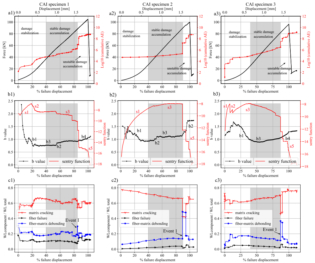
Figure 6.4: damage accumulation study in the three CAI quasi-static tests, each column of plots representing one specimen. In the first row of plots, the force-displacement and the acoustic emission cumulative signal energy (Table 5.2) are plotted. The three phases of damage accumulation are also labeled in the first row of plots. In the second row, the b value and sentry function are shown, pointing out the different trends in the b value (as described in Section 6.3.2 and Figure 6.2) and in the Sentry function (as described in Section 6.3.1 and Figure 6.1). In the third row the wavelet components ratio representing the different damage modes are plotted, and 'event 1' determining the inset of the final propagation phase, is labelled.
