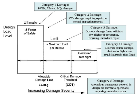
Figure 1.2: Damage tolerance guidelines for CFRP dictated by the EASA [8] the FAA [7]
