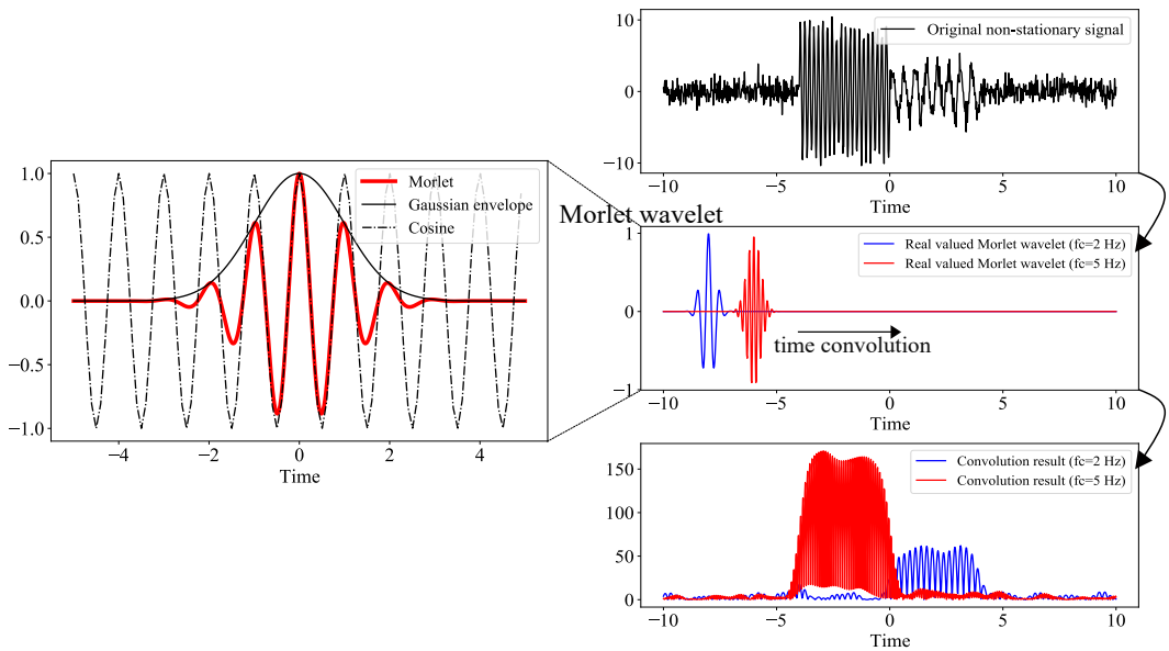
Figure 5.2: Morlet wavelets convolution visually explained
