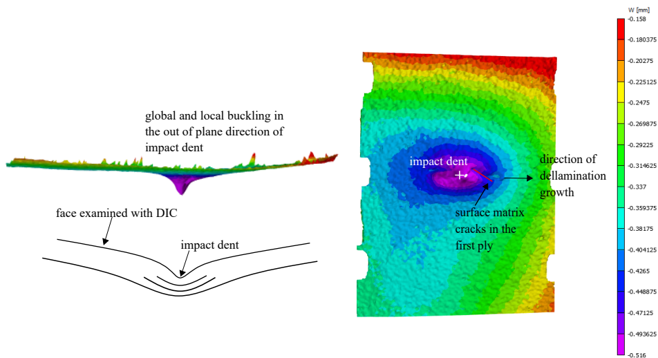
Figure 2.14: Out of plane displacement of loaded specimen s4 derived with DIC analysis. The plot shows the direction of buckling compared to the impact dent. The delamination growth direction and the position of surface cracks is also shown
