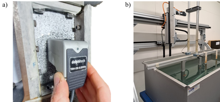
Figure 2.4: Images of the ultrasonic inspections performed showing a) pulse-echo system scanning probe, b) through thickness attenuation water tank
