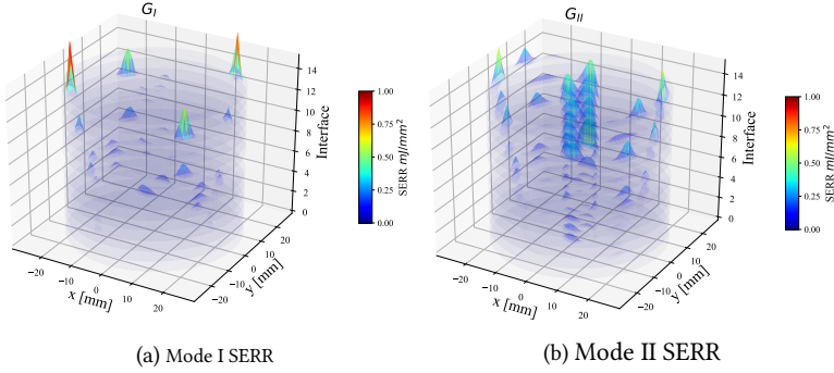
Figure 4.11: G_{max} profile in case internal non-delaminated area radius = 5 mm. Each circular surface in transparent blue represents a VCCT interaction zone (Figure 4.3) modeling one interface. The x and y coordinates of the plot align with the specimen axis, where x = 0 and y = 0 represent the central coordinates of the specimen, and the y-axis indicates the loading direction. The side with larger delamination is placed on top for enhanced visibility.
