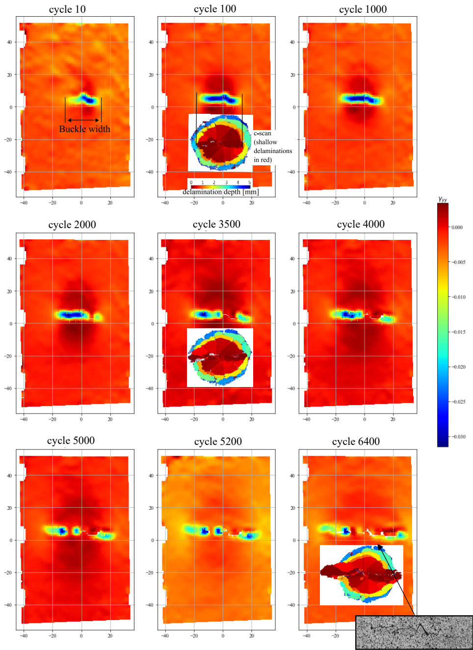
Figure 2.11: DIC results of fatigue propagation showing the \gamma_{yy} engineering strain in specimen s4. The image on top-center shows how the local buckling width in the perpendicular to the loading direction matches the shallow delamination (red colors in the ultrasounds) and not the larger delaminations
