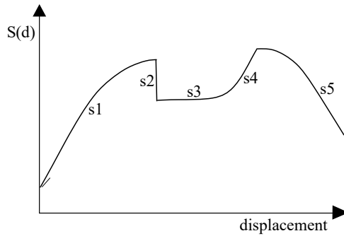
Figure 6.1: Sentry function/displacement plot. The possible trends that can be found in actual tests are shown
