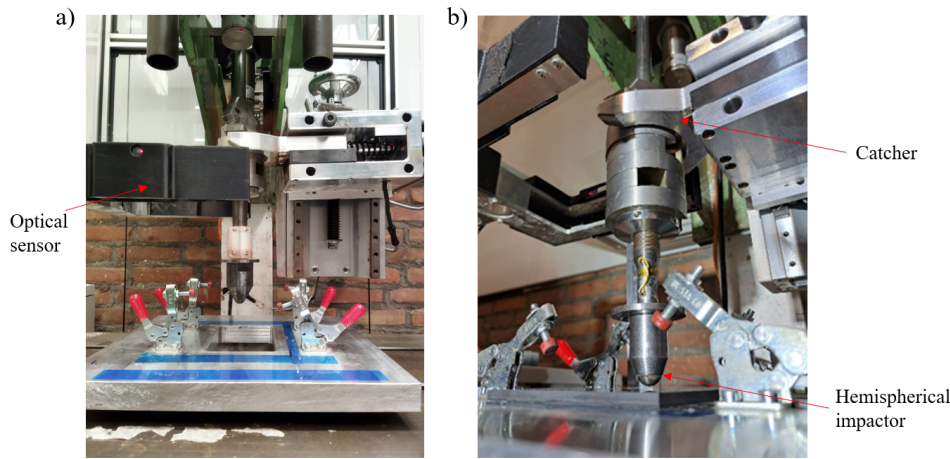
Figure 2.2: Fixture of LVI test showing the hemispherical impactor, the catcher to avoid bounce back triggered by optical sensor
