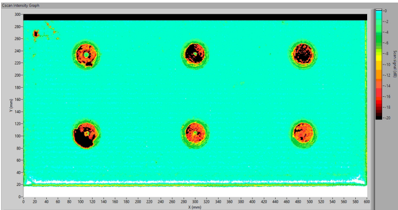
(c) Ultrasound scan of the manufactured plate
