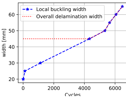
(a) Short fatigue life (specimen s4)
