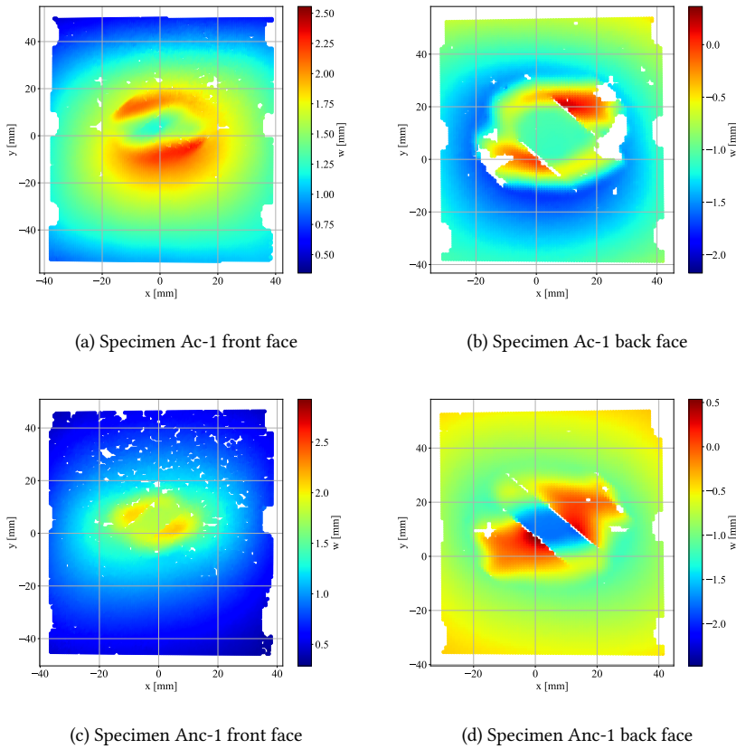
Figure 3.4: Out of plane displacement in specimens Ac-1 and Anc-1 derived with DIC. In the back face (right side figures) a positive out-of-plane displacement (in red) area surrounded by a negative displacement area (in blue) denotes the presence of local buckling having opposite out-of-plane displacement compared to the global buckling. A double/shape local buckling can be seen in both cases, caused by the presence of a central non-delaminated zone.
