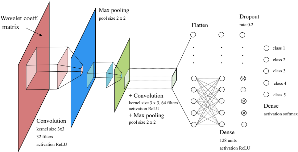
Figure 7.3: Structure of the CNN algorithm. The original images pass through a series of convolution and max pooling layers. Then a dense layer and a dropout are present. Finally dense layer with soft-max activation allows to compute the probability of each class
