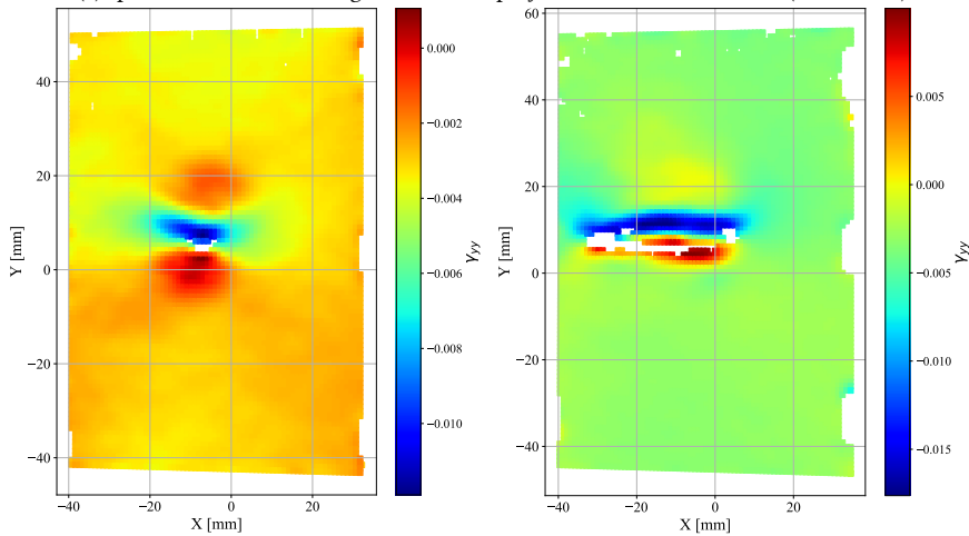
(b) sp 2 at 0% and 90% of fatigue life. Initial projected delamination width (x-direction) = 50 mm
