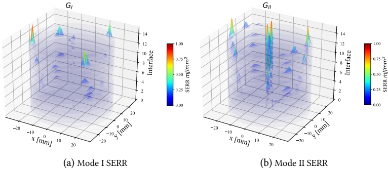
Figure 4.12: G_{max} profile in case internal non-delaminated area radius = 2 mm. Each circular surface in transparent blue represents a VCCT interaction zone (Figure 4.3) modeling one interface. The x and y coordinates of the plot align with the specimen axis, where x = 0 and y = 0 represent the central coordinates of the specimen, and the y-axis indicates the loading direction. The side with larger delamination is placed on top for enhanced visibility.
