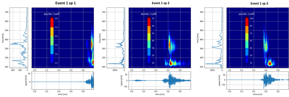
Figure 6.5: Acoustic event preceding the onset of unstable damage propagation in the three tests. The continuum Morlet wavelet scalogram is reported in the three events.
