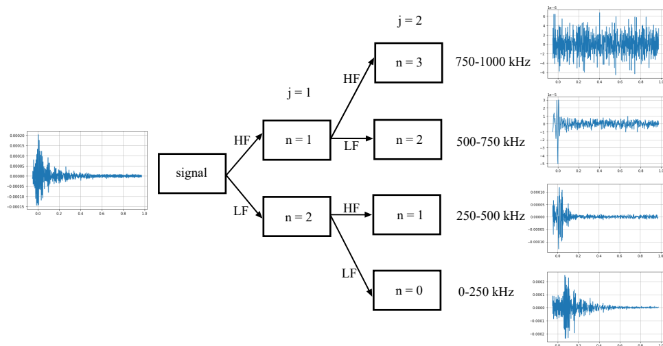
Figure 5.3: Wavelet packet level 2 decomposition tree of an acoustic emission waveform.
