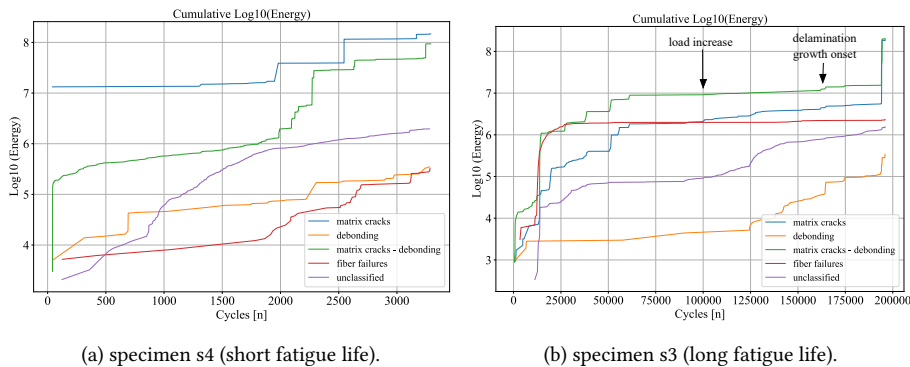
Figure 7.8: Cumulative signal energy plot in logarithmic scale
