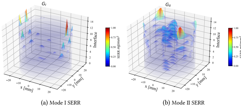
Figure 4.10: G_{max} profile in case internal non-delaminated area radius = 7 mm. Each circular surface in transparent blue represents a VCCT interaction zone (Figure 4.3) modeling one interface. The x and y coordinates of the plot align with the specimen axis, where x = 0 and y = 0 represent the central coordinates of the specimen, and the y-axis indicates the loading direction. The side with larger delamination is placed on top for enhanced visibility.
