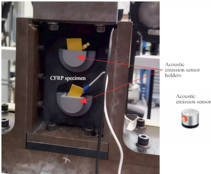
Figure 5.4: CAI fatigue setup showing the AE sensors located inside the 3d printed sensor holders, which are glued to the surface of the CFRP rectangular specimen
