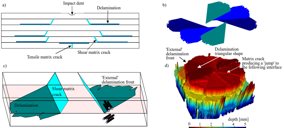
Figure 1.4: BVID in a quasi-isotropic laminate with 45deg angle mismatch between plies a) side view representation b) representation of delaminations (top view) in different interfaces showing the double-triangular shape c) representation of a single interface between two plies showing delamination originating from shear matrix crack d) ultrasound scan of actual impact damage showing the 3d delamination envelope
