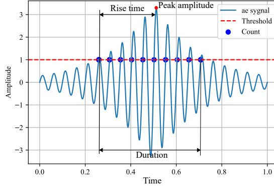
Figure 5.1: Schematic of acoustic emission waveform and some time-domain descriptors
