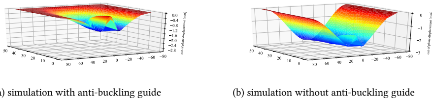
Figure 4.9: FE out of plane displacement with and without restrained buckling
