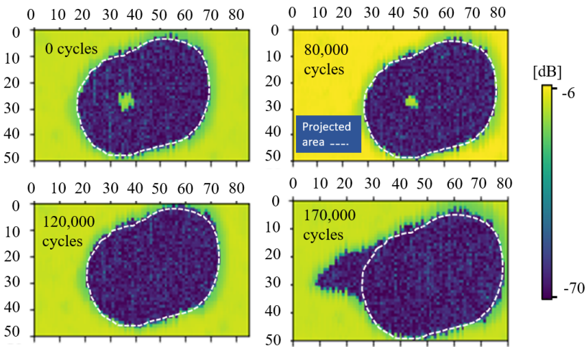
Figure 2.8: through transmission scan monitoring showing growth in the central impact area happening before delamination growth outside of the projected area
