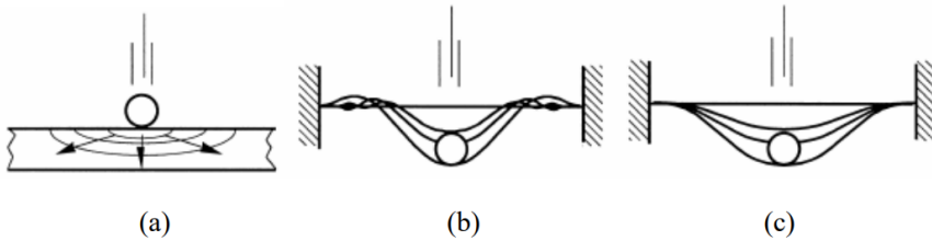
Figure 1.3: Impact response classification: a) short b) medium c) long impact time [11]
