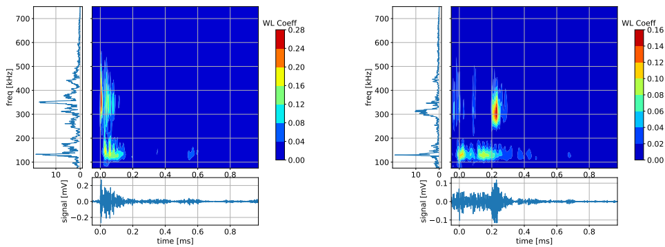
Figure 5.7: The scalogram derived with Morlet wavelets is plotted in two signals located in the proximity of the same cluster centroid with the clustering based on frequency-domain descriptors. Although the frequency spectrum is similar (vertical plots on the left), the wavelet plot reveals that in the second signal, a higher frequency event reaches the sensor after low frequency.
