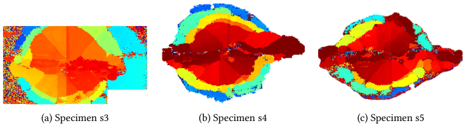
Figure 2.10: Comparison of pulse-echo scans prior to failure (> 90 % of fatigue life) in different specimens with different loads applied and different fatigue lives. Image shows a similar damage envelope before failure, with the extensive growth of delamination of small depths (red colors) in the perpendicular to the loading direction
