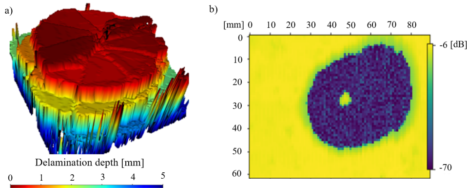
Figure 2.6: Impact damage ultrasound scan obtained with a) pulse-echo and b) through thickness attenuation system
