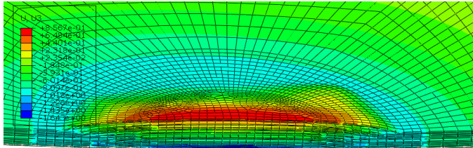
Figure 4.7: A cut section of the deformed laminate is shown. The section is cut in the x direction (perpendicular to loading) from the center point. It shows the sub laminates opening in the out of plane direction. The back face is placed on top in the figure to better show the larger delaminations.
