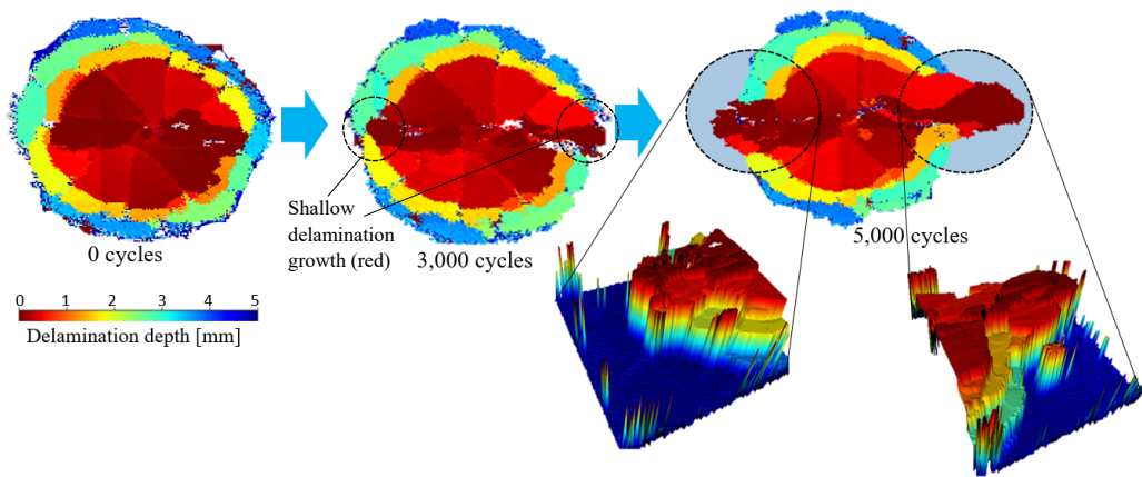
Figure 2.9: Pulse-echo scan monitoring of specimen s4 showing the preferential growth of shorter delamination (in width) happening before the onset of growth outside of the projected area. Initial growth affects mostly shallow delaminations i.e. situated at small depth with respect to the impacted face
