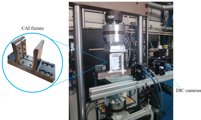
Figure 2.3: CAI fixture with DIC cameras
