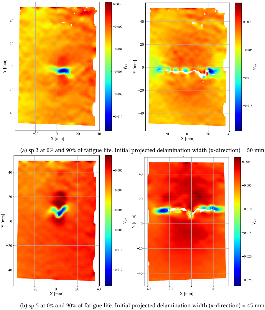
Figure 2.13: Comparison of strain fields at different specimens at the beginning and close to the end of fatigue life. The results show growth of local buckling in the perpendicular to width directions, starting from an initial size smaller than the overall projected width of delamination (in the x-axis direction).
