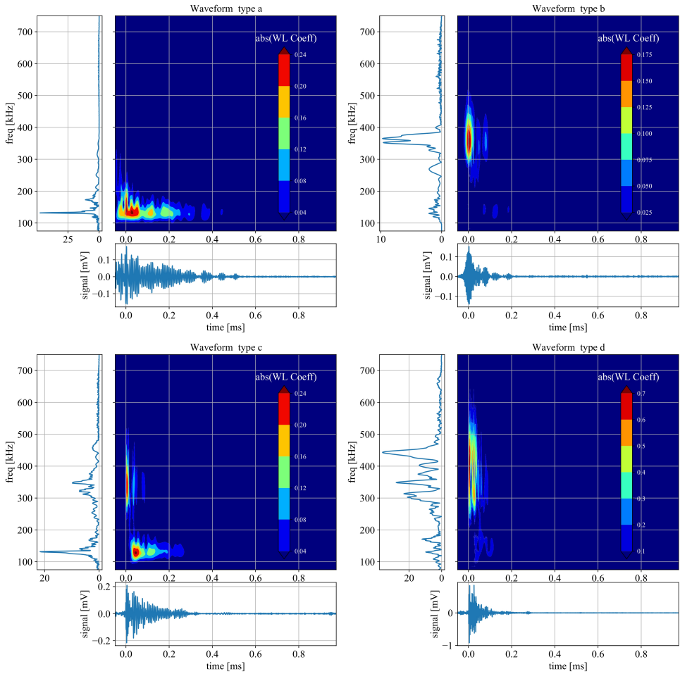
Figure 5.5: Wavelet transform of the different types of waveforms. The color plot represents the coefficient derived from the Morlet wavelet transform. The vertical subplots show the frequency spectrum derived from the Fourier transform. The horizontal subplots show the original signal
