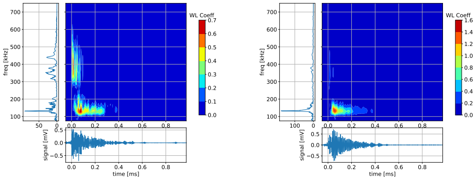
Figure 5.6: The scalogram derived with Morlet wavelets is plotted in two signals located in the proximity of the same cluster centroid with the clustering based on time-domain descriptors. Although the signals in the time domain appear similar (horizontal subplots) large differences can be found in The frequency domain (vertical subplots) and in the wavelet coefficient.
