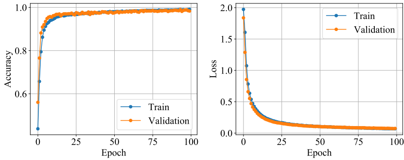
Figure 7.4: Performance of the training. The accuracy and the loss progression in the training and validation set are shown over the epochs. A good convergence is reached at 100 epochs.
