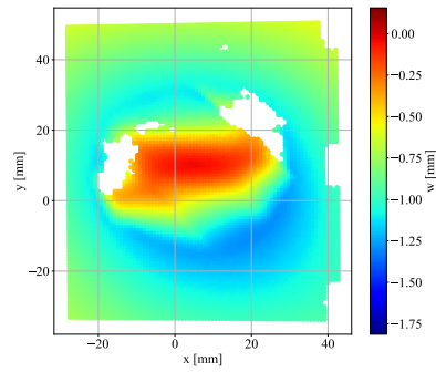
(b) Specimen C-1 back face
