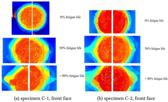
Figure 3.5: Ultrasound scan at different stages of fatigue life in specimen C-1 and C-2. The results show the propagation of several delaminations at multiple depth locations, all in the perpendicular to the loading direction
