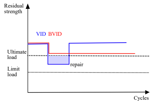
Figure 1.6: No growth procedure for BVID and VID
