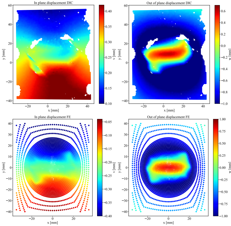
Figure 4.4: Comparison of DIC surface displacement in specimen c-2 (top images) and FE simulations (bottom images). Left side of the figure compares in-plane displacement while right side of the image compares out of plane displacements.
