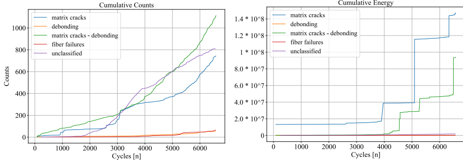
Figure 7.6: Damage modes repartition plots in specimen s4 (short life). In the left plot, the progression of cumulative count in fatigue life is shown for every damage mode. On the right, the cumulative ae signal energy is shown (defined in Table 5.2).
