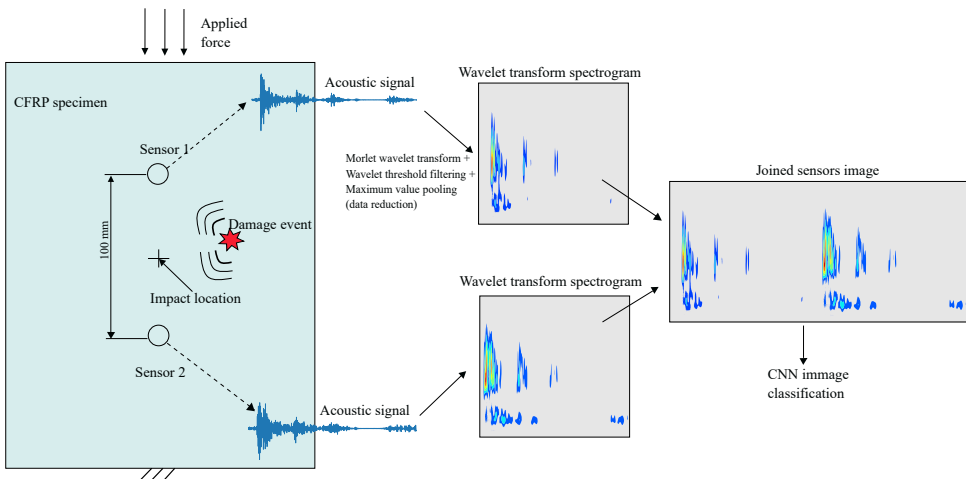
Figure 7.2: Data processing from sensor data to input of the CNN. Continuum Morlet waveform transform is applied to the acoustic signal in the two sensors. Then the two scalograms are joined to form a single image.
