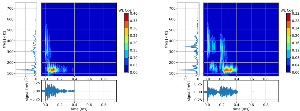
Figure 5.8: The scalogram derived with Morlet wavelets is plotted in two signals located in the proximity of the same cluster centroid with the clustering based on time-frequency domain descriptors. The frequency spectrum is similar (vertical subplots), and descriptors in the time domain (horizontal subplots) like rise time, peak amplitude, and duration are similar. However, wavelet plots show largely different scalograms.
