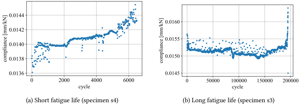
Figure 2.16: Degradation of stiffness in (a) short and (b) long fatigue lives
