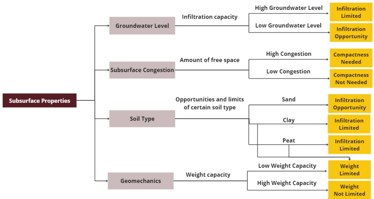
Figure 1. Decision tree for design interventions based on subsurface properties
