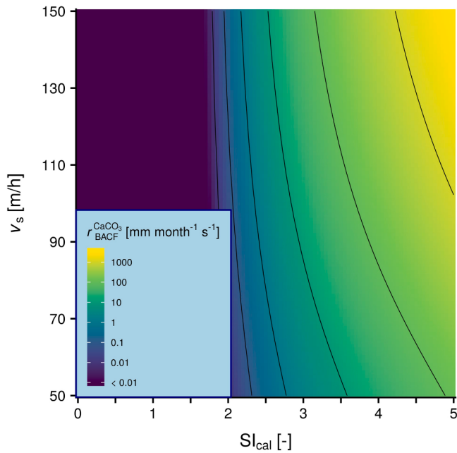
Fig. 4. r_{\text{CaCO}_3}^{\text{BACF}} versus v_s and SI_{\text{cal}} . The black contour lines are a guide for the eye and are drawn at every order of magnitude between 0.01 – 1000 \text{mm month}^{-1} \text{s}^{-1} . Simulated data of r_{\text{CaCO}_3}^{\text{BACF}} at other T -values is found as Figure S36 in SI-X.
