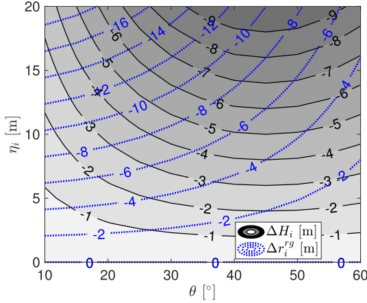
Fig. 5. Height error \Delta H_i and ground range error \Delta r_i^{\text{rg}} as function of range sub-pixel position \eta_i and incidence angle \theta , in the case of Radarsat-2 data.
