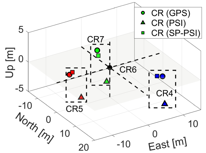
Fig. 16. Location of CR4, CR5, and CR7 relative to CR6. The circles indicate the position of CR4, CR5, CR7 estimated by GPS. The squares indicate the estimated position of the reflectors by SP-PSI with TerraSAR-X. The triangles indicate the estimated position of the reflectors by PSI.
