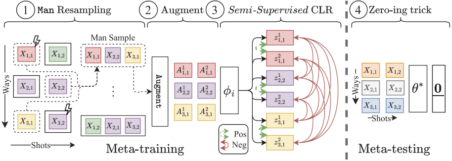
Fig. 1. Illustration of meta-learning with BatMan on a noisy 3-way 2-shot few-shot learning task, i.e., a (3, 2)-FSL. The task is provided to the learner as containing three classes (ways): red, purple, and yellow, with two supporting samples (shots) each. Colors indicate the true underlying class (ground-truth), while lightning bolts indicate shots provided with a mismatched label (i.e., noisy) (way 1 shot 1, and way 3 shot 2). Steps: ① Man sampling (Algorithm 2) creates a batch of (3, 1)-FSL manifold samples; ② Augment creates semi-supervised (3, 2)-FSL sub-tasks via independent random augmentations; ③ a contrastive loss jointly optimizes all sub-tasks via (Pos)itive and (Neg)ative pairs; ④ trained meta-model \theta^* is meta-tested in a supervised way by appending a zero-ed out linear layer. (Color figure online)
