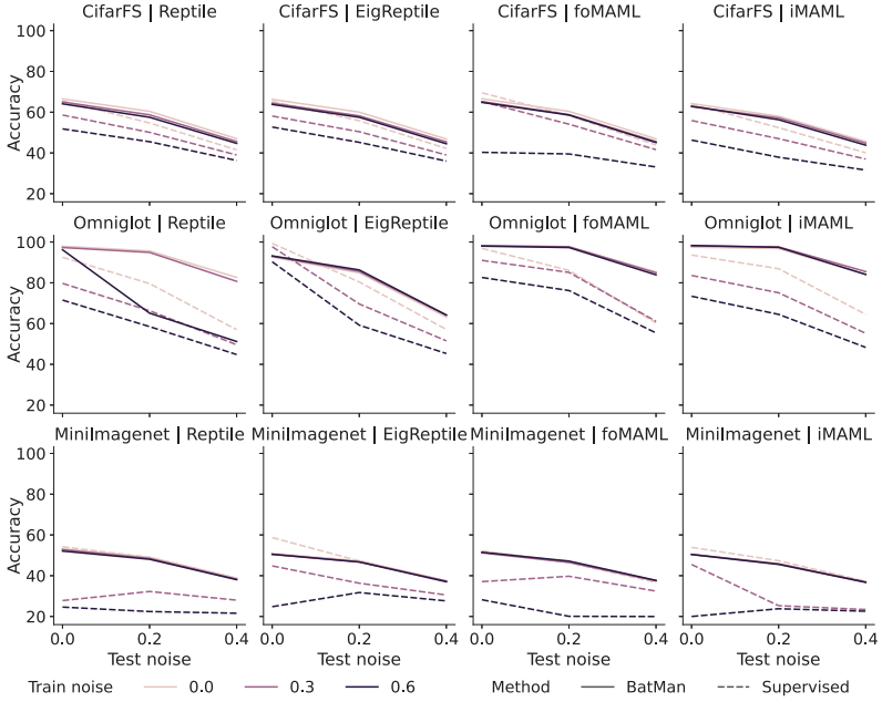
Fig. 2. Meta-test accuracy of supervised and BatMan-CLR meta-trained models with different meta-learners, training, and testing noise levels. Results shown meta-trained with dataset-level label noise ( \epsilon \in \{0.0, 0.3, 0.6\} ) and meta-testing label noise ( \epsilon \in \{0.0, 0.2, 0.4\} ) at task-level.
