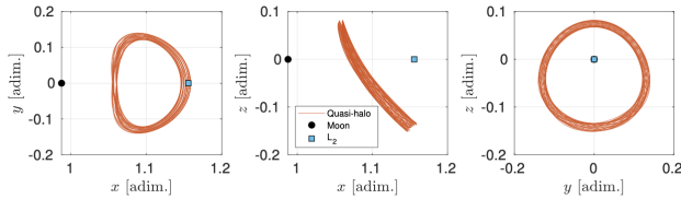
Figure 3. Projection of the selected operative Earth-Moon L_2 quasi-halo in the Roto-Pulsating Frame. Dimensions are provided relative to the average Earth-Moon distance.
