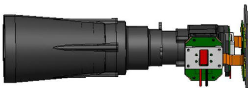
Figure 8. The LUMIO-CAM [7].
