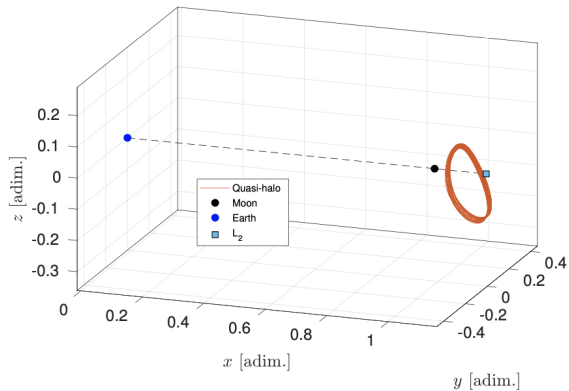
Figure 4. Selected operative Earth-Moon L_2 quasi-halo orbit in the Earth-Moon synodic frame. Dimensions are provided relative to the average Earth-Moon distance.
