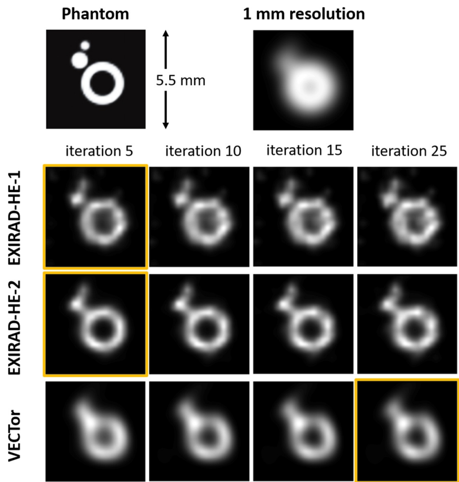
Figure 9. Simulation of a mouse tumour xenograft phantom with the optimal collimators (table 5) in comparison with the HE-UHR-M collimator in VECTor and the 1 mm blurred image of the phantom. Images are shown at several iteration numbers, and the images with the lowest NMSE are enclosed in boxes. The optimal NMSE is 0.05, 0.03, and 0.12 for EXIRAD-HE-1, EXIRAD-HE-2, and VECTor, respectively. Slice thickness was 0.5 mm.
