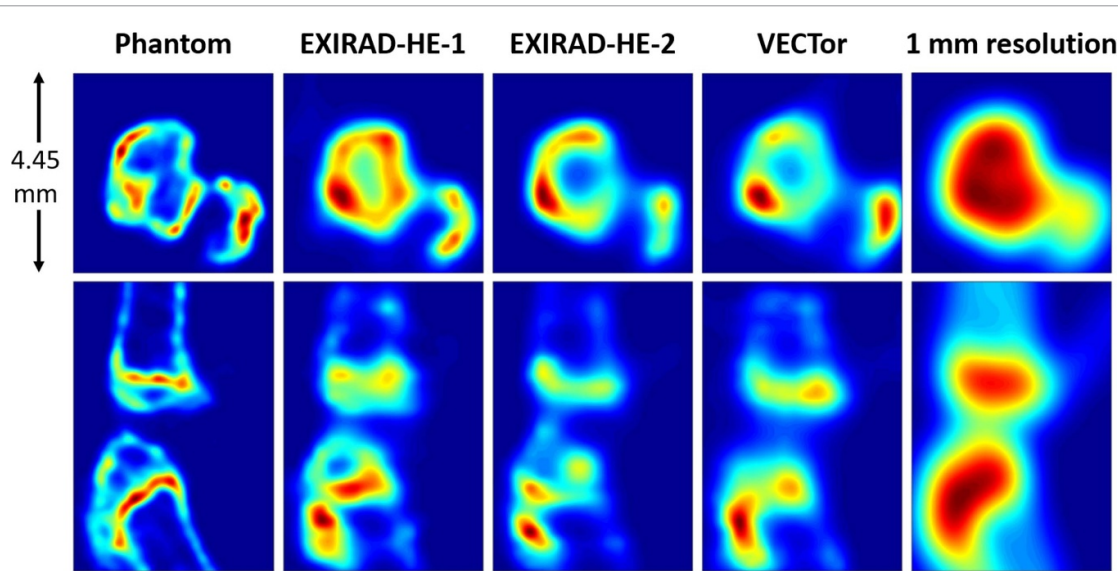
Figure 8. Simulation of a mouse knee joint phantom with the optimal collimators (table 5) in comparison with the HE-UHR-M collimator in VECTor and the 1 mm blurred image of the phantom. The images are shown at the iteration number that gives the lowest NMSE. The optimal NMSE is 0.17, 0.18, and 0.25 for EXIRAD-HE-1, EXIRAD-HE-2, and VECTor, respectively. Slice thickness was 0.5 mm.
