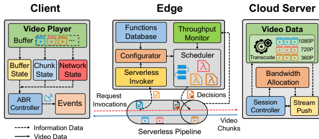
Fig. 5. An overview of our serverless video streaming system.
