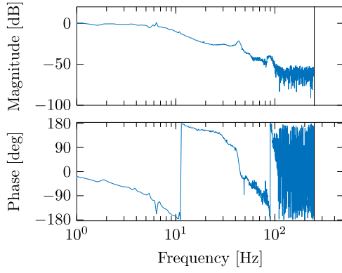
Fig. 2. Bode diagram of the measured frequency response of the closed loop T = (1 + PC)^{-1} PC (—).
