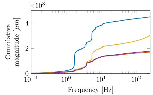
Fig. 15. Cumulative error spectrum without compensation (—) and with compensation of the disturbances originating from both drive belts. Multirate RC (—) is able to match the performance of traditional RC (—), while low-rate RC (—) cannot attenuate the disturbance at 5.4 Hz due to the period mismatch.
