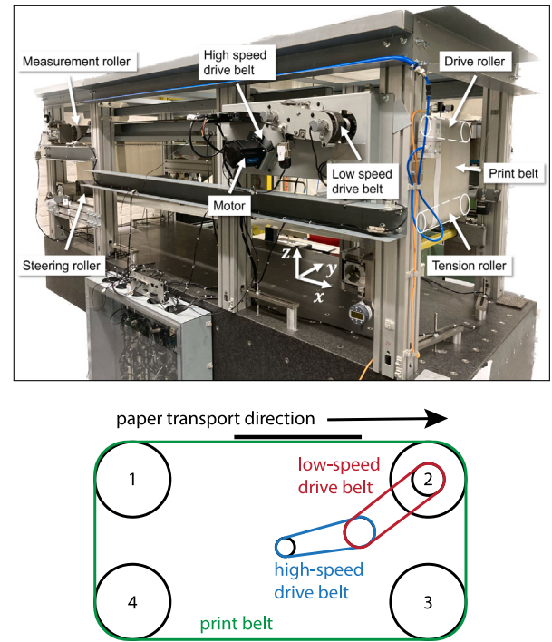
Fig. 1. Industrial print-belt system (top) and schematic representation (bottom). The aim is to transport paper on the print belt (—) with a constant velocity. The rollers (1: measurement roller, 2: drive roller, 3: tension roller, 4: steering roller) and drive belts (high-speed (—) and low-speed (—)) induce various repeating disturbances in the system.
