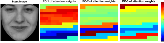
Fig. 5. The visualization of the learned attention weights of the first spatially-indexed attention layer. The Principal Component Analysis (PCA) is performed on the 256-dimension attention weights for each pixel of the attention map. The first 3 principle components (PC) which accounts for 55% variance are visualized.
