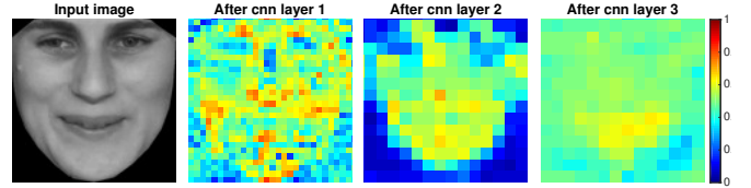
Fig. 4. The visualization of the learned spatial attention weights when placing the spatial attention module after different convolutional layers. Note that we adopt the spatially-indexed mechanism described in Section V-A1.
