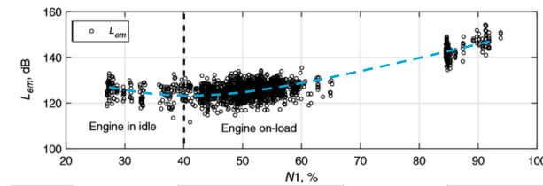
Fig. 7 N1 versus emitted noise for the A320 at 100 Hz. (Adapted from Zellmann et al. [10])
