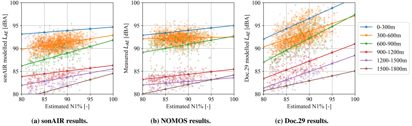
Fig. 5 Relations between the estimated N1 and the modelled and measured L_{AE} for different distance bins.
