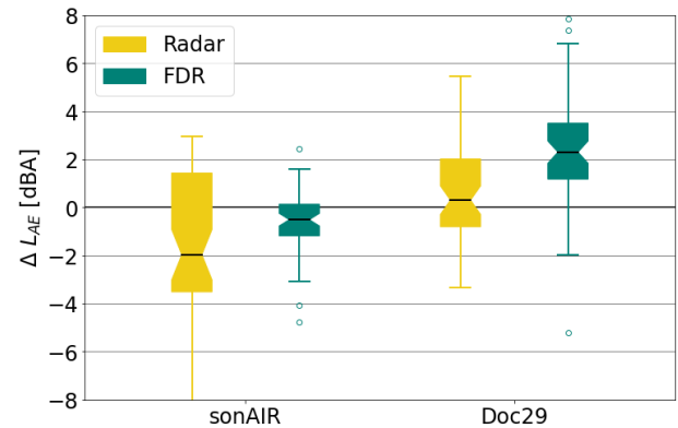
Fig. 6 Boxplots showing \Delta L_{AE} for flights simulated with FDR data and radar data
