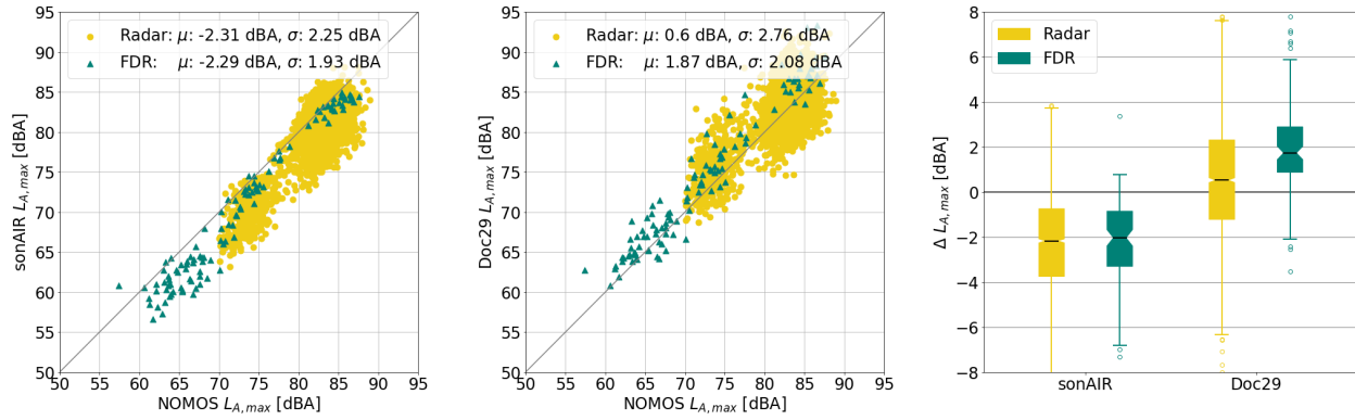
Fig. 8 L_{A,max} comparison for B737 series departures (FDR: 112 events, radar: 2,761 events)
