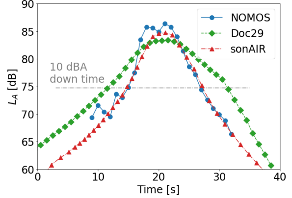
Fig. 4 Example noise level time history for B737NG departure
