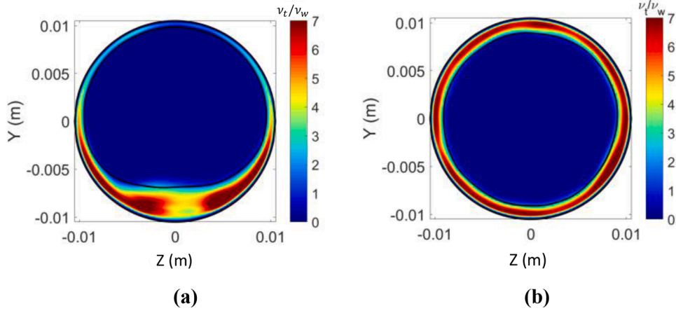
Fig. 9. Comparison of the turbulent viscosity (scaled with the water viscosity) for the 3D simulation; (a) with gravity, (b) without gravity. Values are averaged over time and along the main flow direction. The oil-water interface is indicated with a solid black line.
