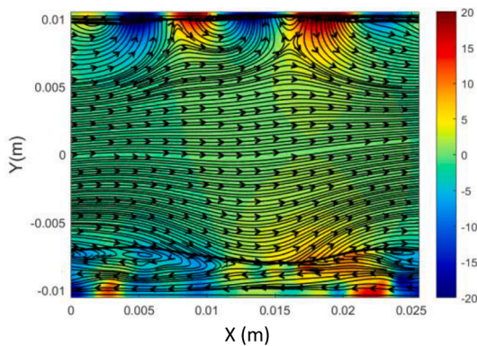
Fig. 16. Snap shot of the pressure fluctuation in the mid plane, as well as streak lines of the secondary flow. The oil-water interface is represented by a thick black line.
