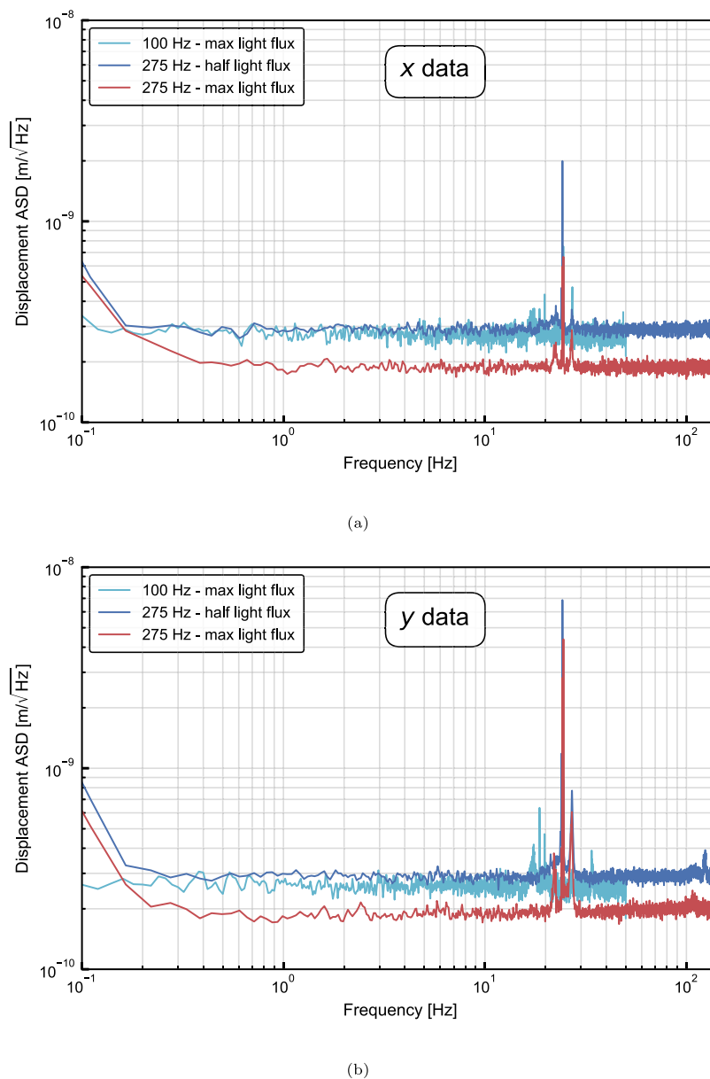
Fig. 12. Welch plot of a SolidRas data set, taken during a period of 30 min. Red: best performance at maximum practical frame rate (275 Hz). Light blue: frame rate reduced to 100 Hz, maintaining exposure time. Dark blue: frame rate 275 Hz, LED current reduced by factor 2. (a) x data, and (b) y data. Colour figures online.
