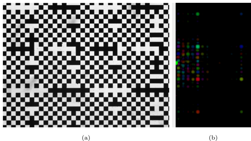
Fig. 7. (a) Typical Rasnik image from SolidRas. Here, a ChessField mask of 120\mu\text{m} was applied. (b) Typical SolidRas FFT-converted Rasnik image of Fig. 7(a). The peaks are associated with the periodicity of the image pattern defined by the ChessField side and by the coarse rows and columns at 9 times the ChessField side. All peaks may contribute to the determination of the phase of the contours.
