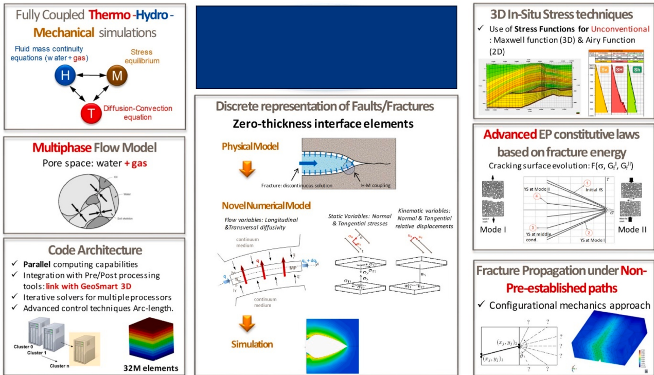
Fig. 8. Components, understanding required and architecture of a multiphysics full fidelity numerical model for fracture propagation on an oil & gas reservoir (image supplied by Repsol).
