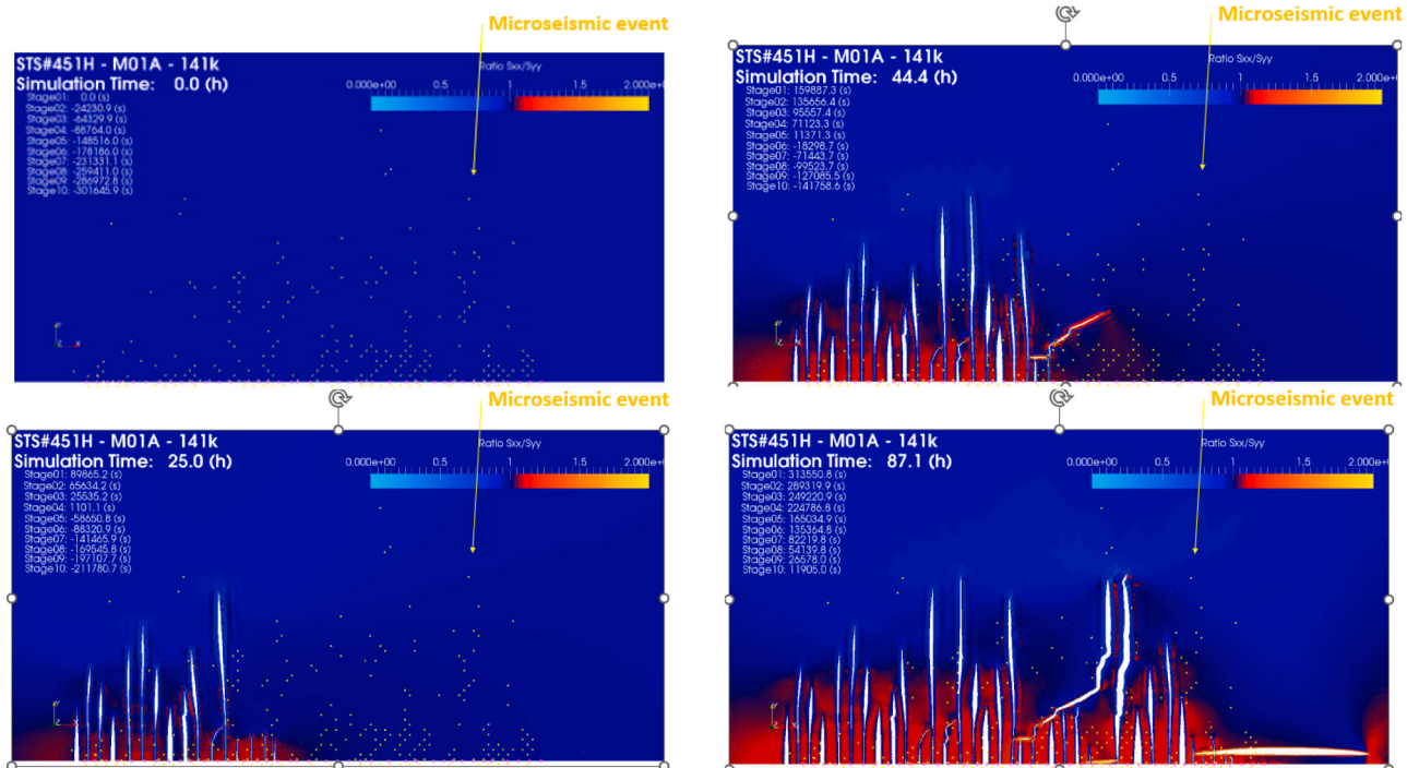
Fig. 10. High fidelity fracture propagation numerical model in a reservoir over 90 h of fluid injection, with multiple natural fractures interacting in the development and propagation of the anthropogenic new fractures. Snapshots at 0, 25, 44 and 87 h are shown.
