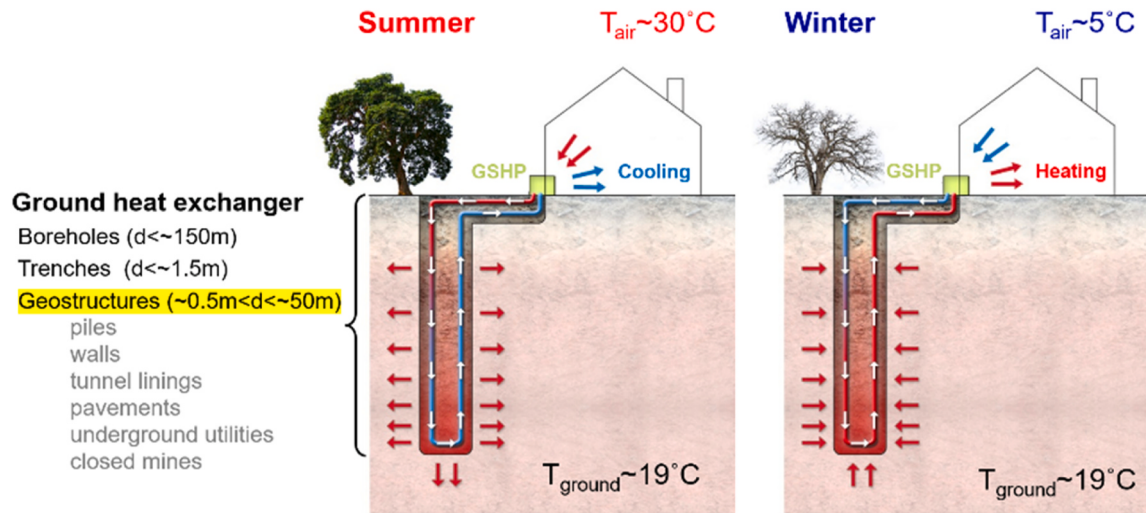
Fig. 6. A ground source heat pump (GSHP) system in a temperature climate site (hinted by the ground temperature T_{\text{ground}} at 19^{\circ}\text{C} ), showing different options for used and trialled ground heat exchangers (GHEs) (modified from 10 ).
