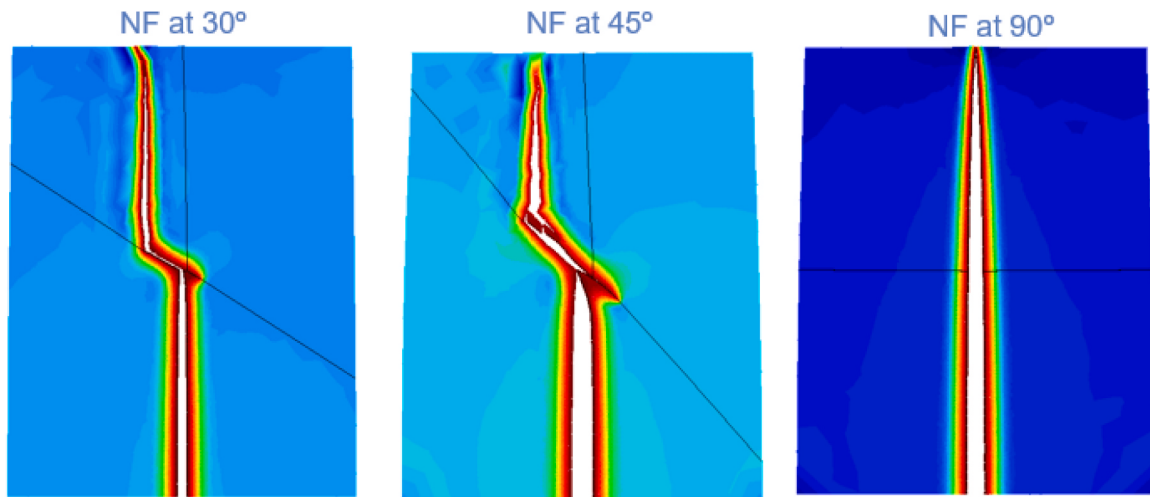
Fig. 9. Fracture propagation and effect of natural fractures (NF) deeping on a relatively simple test case.
