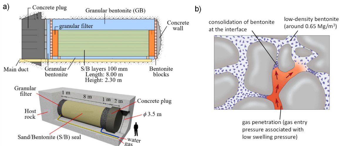
Fig. 5. Engineered gas permeable sand/bentonite S/B seal for a deep geological repository of low and intermediate-level (L/ILW) radioactive waste. a) Schematics of the in situ GAST experiment showing the compaction layers of the S/B seal. b) Schematic of gas transport mechanism in S/B (a) (modified from 4,5 ). (b) (modified from 6 ).
