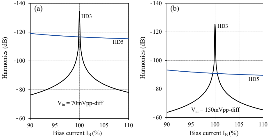
Figure 5.6: Simulated nonlinearities of the amplifier versus its bias current (in percentage) for (a) 70\text{mV}_{p-p,diff} and (b) 150\text{mV}_{p-p,diff} input signals.
