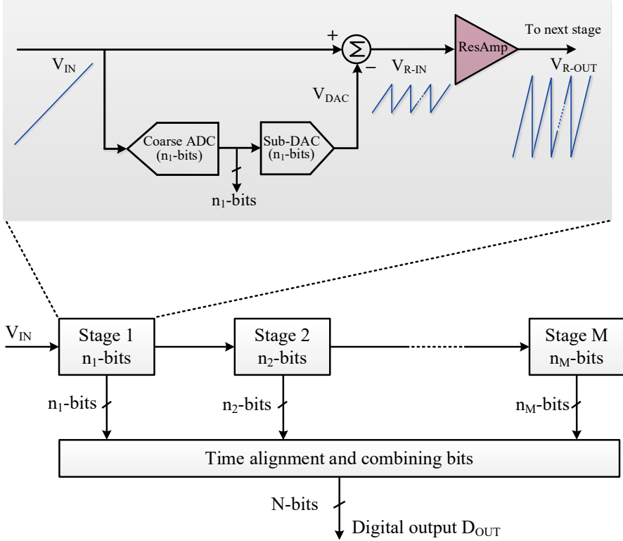
Figure 1.2: Simplified block diagram of a pipelined ADC.
