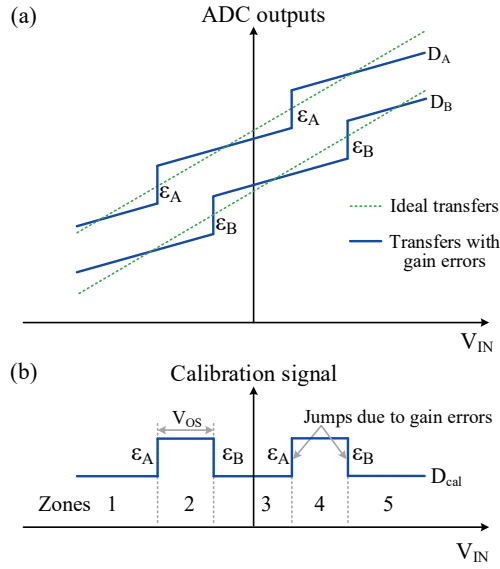
Figure 2.10: (a) ADC transfers and (b) calibration signal when the residue amplifier has gain error.
