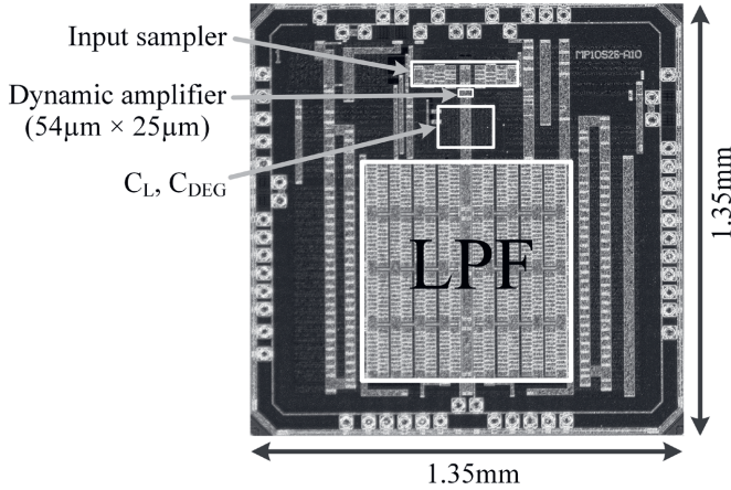
Figure 6.13: Chip photograph.
