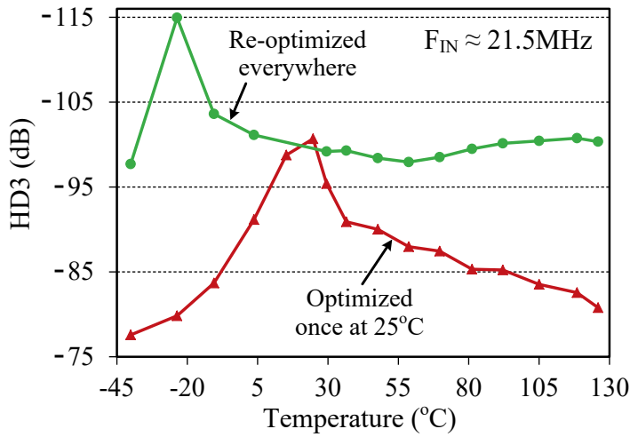
Figure 6.19: Measured amplifier linearity over the temperature range -40°C to 125°C.
