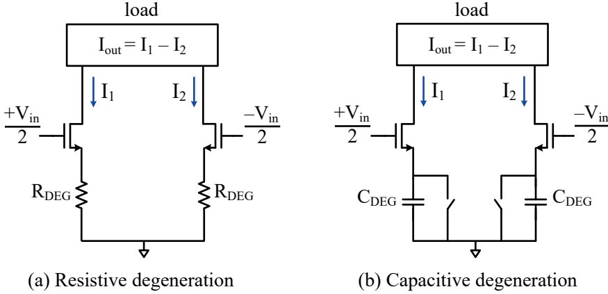
Figure 3.7: Basic amplifier configurations for the presented linearization technique in the weak-inversion region, using (a) resistive and (b) capacitive degeneration.
