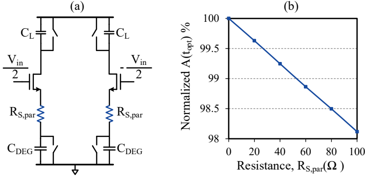
Figure 6.6: Effect of series resistance R_{S,par} on the amplifier's optimum gain A(t_{opt}) .
