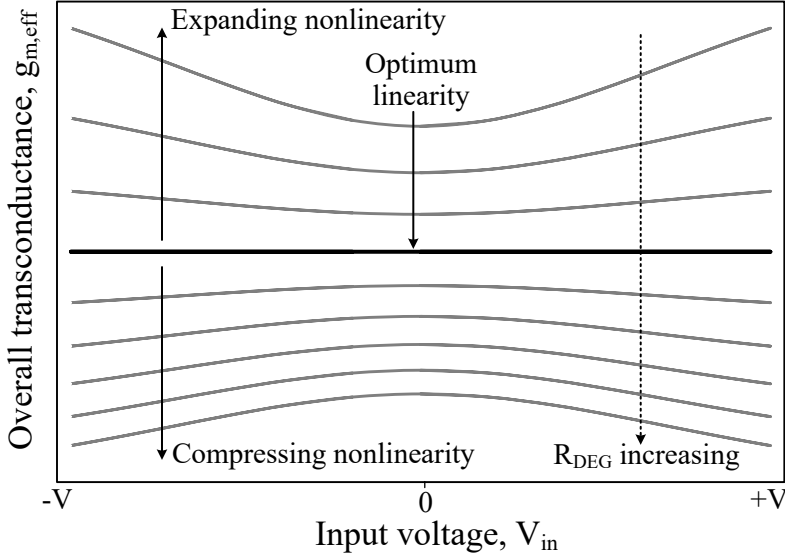
Figure 3.11: Transition from an expanding to a compressing nonlinearity as the degeneration resistance R_{\text{DEG}} increases.
