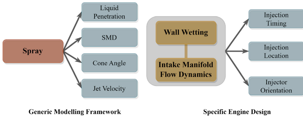
Figure 2. Pillars of PFI conditions modelling.
