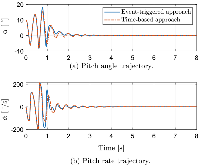
Fig. 10.18 Evolution of the pitch motion states
