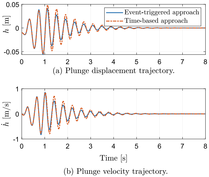
Fig. 10.17 Evolution of the plunge motion states
