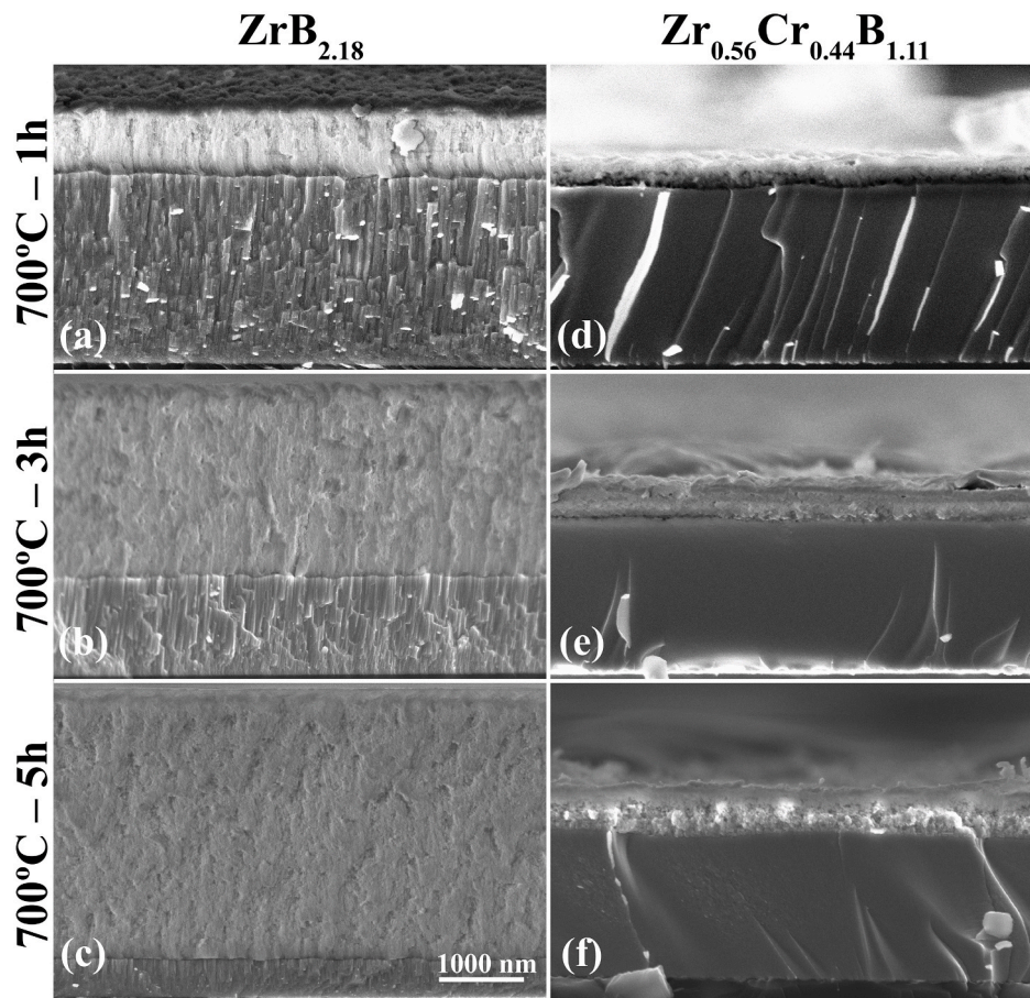
Fig. 8. XSEM images of \text{ZrB}_{2.18} and \text{Zr}_{0.56}\text{Cr}_{0.44}\text{B}_{1.11} thin films annealed at 700 °C for (a and d) 1 h, (b and e) 3 h, and (c and f) 5 h. The films are grown on Si(001) substrates. From the phase diagrams, Si has less affinity to the boride components than Al and O; thus, Si substrates are the better choice to elucidate the role of oxidation. The scale bar is the same for all panels.
