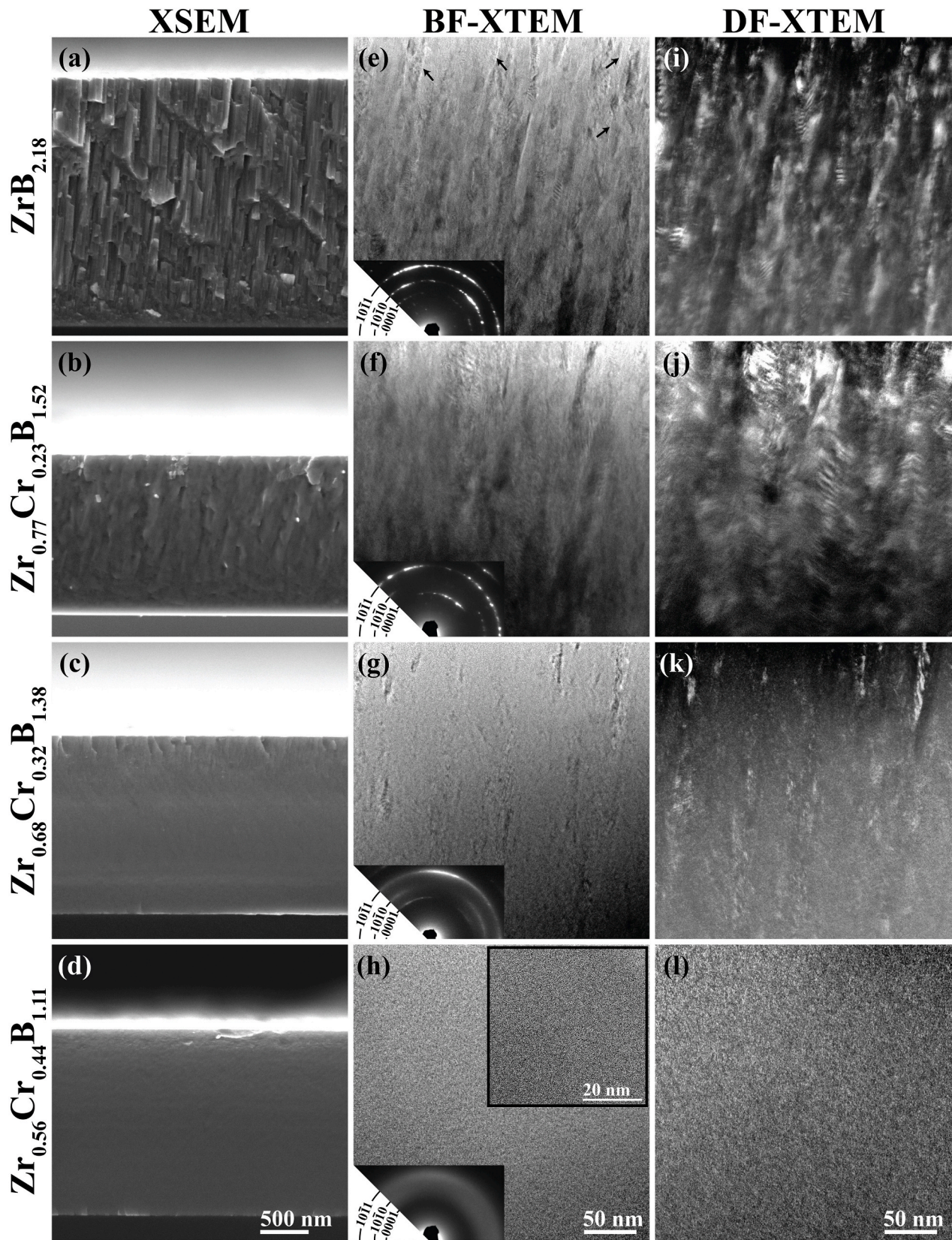
Fig. 3. XSEM, BF-XTEM, and DF-XTEM images of as-deposited (a, e, i) \text{ZrB}_{2.18} , (b, f, j) \text{Zr}_{0.77}\text{Cr}_{0.23}\text{B}_{1.52} , (c, g, k) \text{Zr}_{0.68}\text{Cr}_{0.32}\text{B}_{1.38} , and (d, h, l) \text{Zr}_{0.56}\text{Cr}_{0.44}\text{B}_{1.11} thin films grown on Si(001) substrates. The corresponding SAED patterns are given in insets. The high-resolution BF-XTEM image of \text{Zr}_{0.56}\text{Cr}_{0.44}\text{B}_{1.11} is shown as inset in (h). The brightness appearing at the substrate/film interfaces in XSEM images of \text{Zr}_{0.77}\text{Cr}_{0.23}\text{B}_{1.52} and \text{Zr}_{0.68}\text{Cr}_{0.32}\text{B}_{1.38} films originates from charging.
