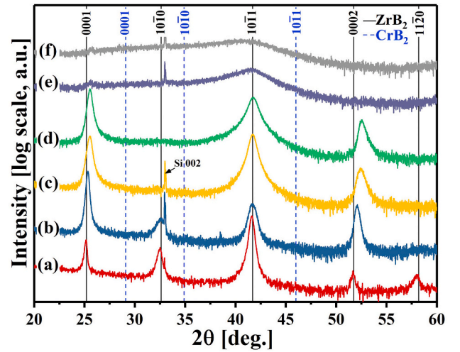
Fig. 1. XRD 0-20 scans of as-deposited (a) ZrB 2.18 , (b) Zr 0.77 Cr 0.23 B 1.52 , (c) Zr 0.71 Cr 0.29 B 1.42 , (d) Zr 0.68 Cr 0.32 B 1.38 , (e) Zr 0.64 Cr 0.36 B 1.30 , and (f) Zr 0.56 Cr 0.44 B 1.11 thin films grown on Si(001) substrates. The peak at 32.8° is the 002 forbidden reflection arising from Si(001) substrate, which appears due to multiple scattering events [42].
