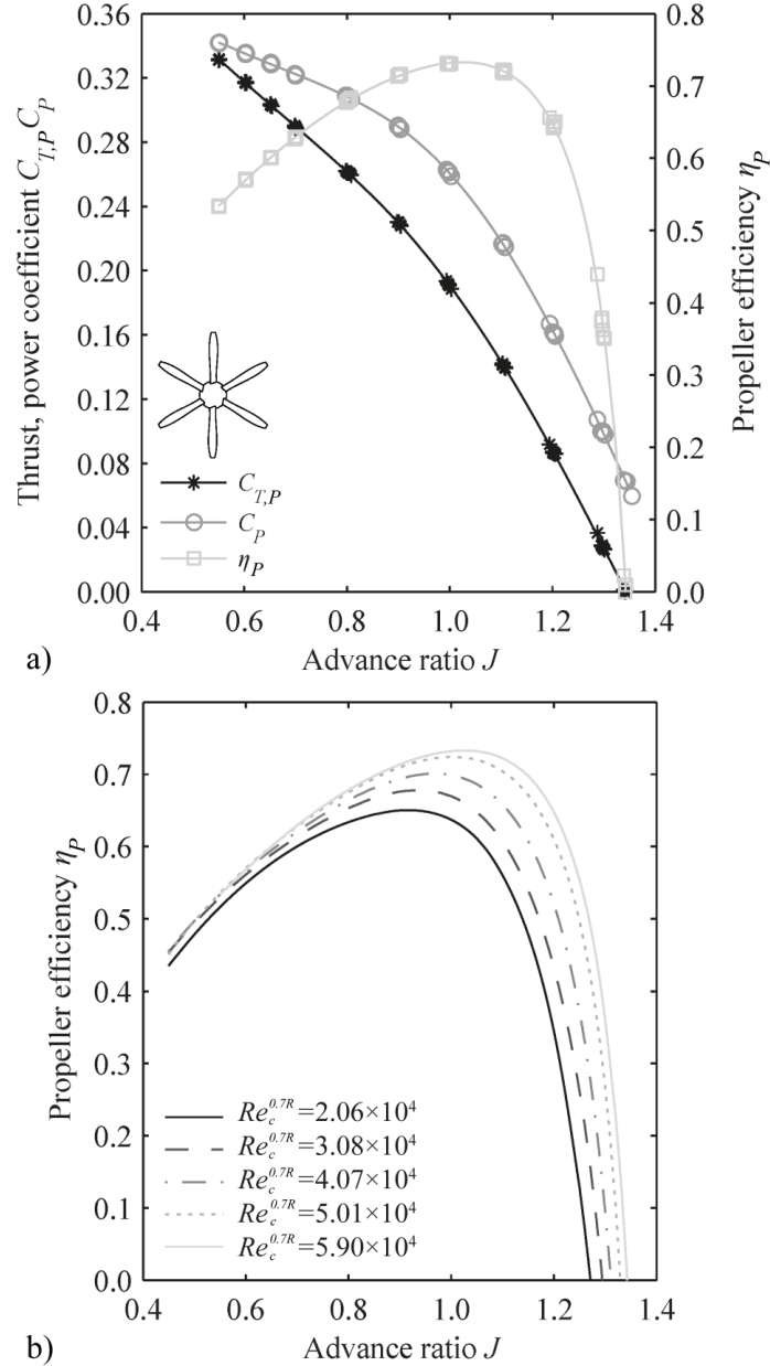
Figure 2.6 Example performance curves measured with the propeller illustrated in Figure 3.5 at \beta_{0.7R} = 30^\circ : a) propeller performance operating at Re_c^{0.7R} = 5.90 \times 10^4 ; b) effect of Reynolds number on propeller efficiency. (Adapted from Sinnige [45])
