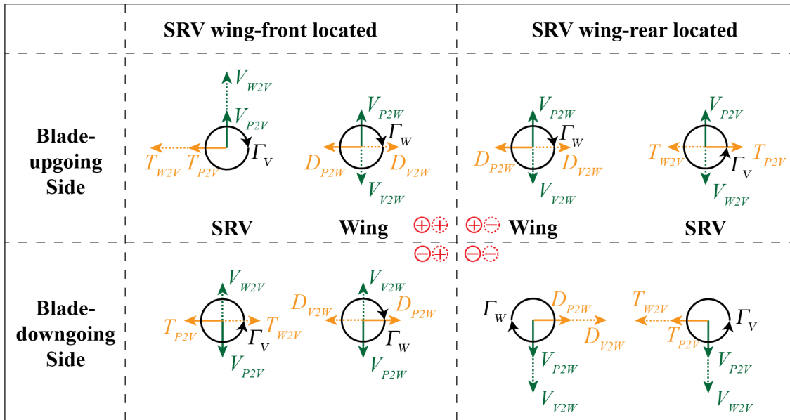
Figure 4.9 SRV-wing mutual induced velocity and force diagrams. In this scheme, the SRV-wing system is viewed from the side with the undisturbed flow coming in from the left.
