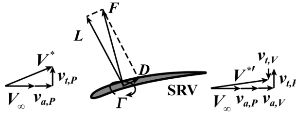
Figure 1.4 Illustration of swirl recovery by SRV.
