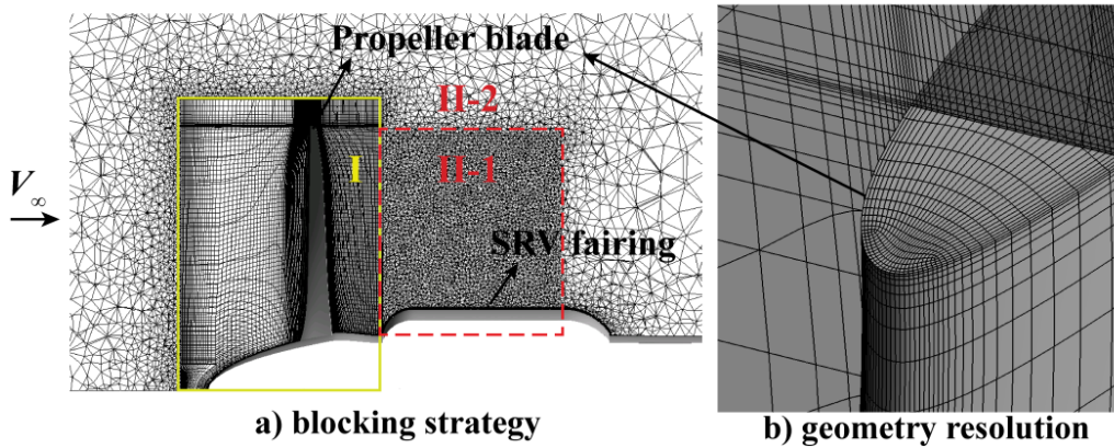
Figure 3.6 Hybrid computation mesh for the isolated propeller.
