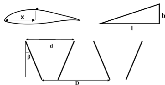
Figure 2. Triangular vane vortex generator parameters. Top left: Airfoil side view, Top right: VG side view, Bottom VG top view.
