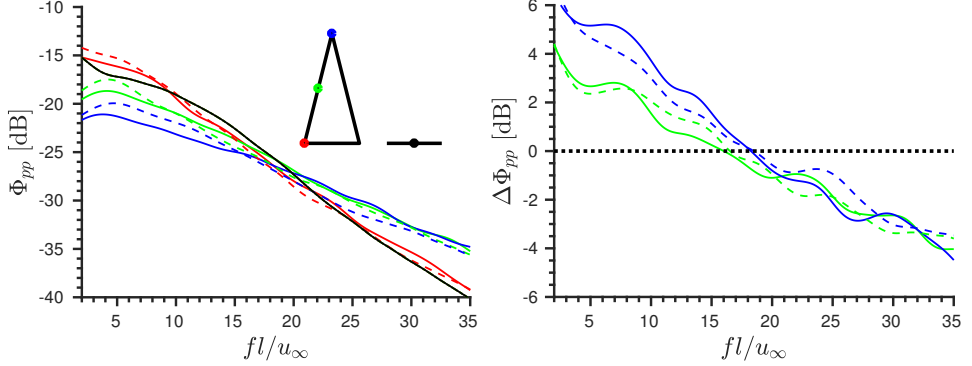
Figure 6.15: (left) Spectra of the surface pressure fluctuations ( \Phi_{pp} ) at three streamwise locations corresponding to x/2h = 0 (red), 0.5 (green) and 1 (blue). The continuous and dashed lines represent the teeth and the combed teeth serrations respectively. (right) \Delta\Phi_{pp} = \Phi_{pp}^{root} - \Phi_{pp}^{stream} with respect to the root location.
