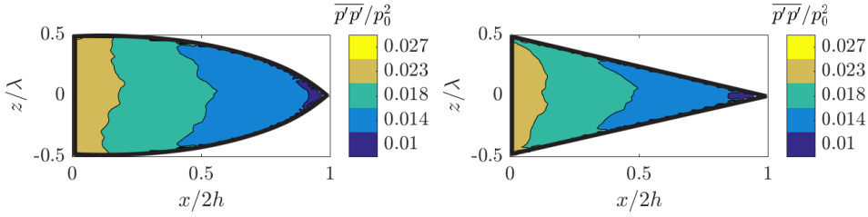
Figure 7.9: Intensity of the mean wall pressure fluctuation ( \overline{p'p'}/p_0^2 ): (left) iron-like serration, (right) sawtooth serration. The serration on the x-z plane are indicated by means of continuous black lines.
