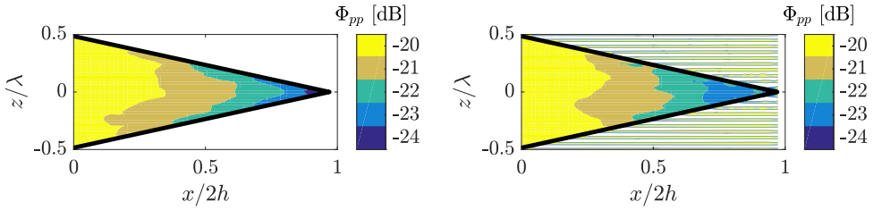
Figure 6.13: Intensity of the surface pressure fluctuation ( \Phi_{pp} ) around St_l = 10 : (left) teeth and (right) combed teeth. The serration edge in the x-z plane is indicated by means of continuous black lines.
