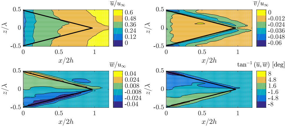
Figure 6.7: Contour of the mean velocity component over the teeth serration at y/\delta = 0.05 : (top left) stream-wise \bar{u} , (top right) wall-normal \bar{v} and (bottom left) spanwise \bar{w} velocity components. Projections of the solid serration on the x - z plane are indicated by means of continuous black lines.
