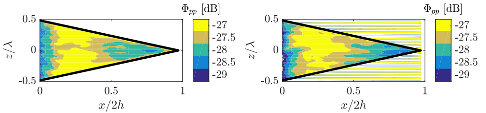
Figure 6.14: Intensity of the surface pressure fluctuation ( \Phi_{pp} ) around St_l = 20 : (left) teeth and (right) combed teeth. The serration edge in the x-z plane is indicated by means of continuous black lines.
