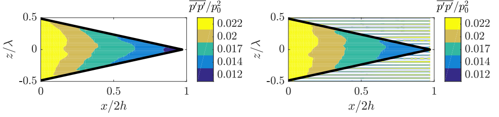
Figure 6.11: Intensity of the mean surface pressure fluctuation ( \overline{p'p'}/p_0^2 ): (left) teeth and (right) combed teeth. The serration edge in the x-z plane is indicated by means of continuous black lines.
