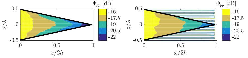
Figure 6.12: Intensity of the surface pressure fluctuation ( \Phi_{pp} ) around St_l = 4 : (left) teeth and (right) combed teeth. The serration edge in the x-z plane is indicated by means of continuous black lines.
