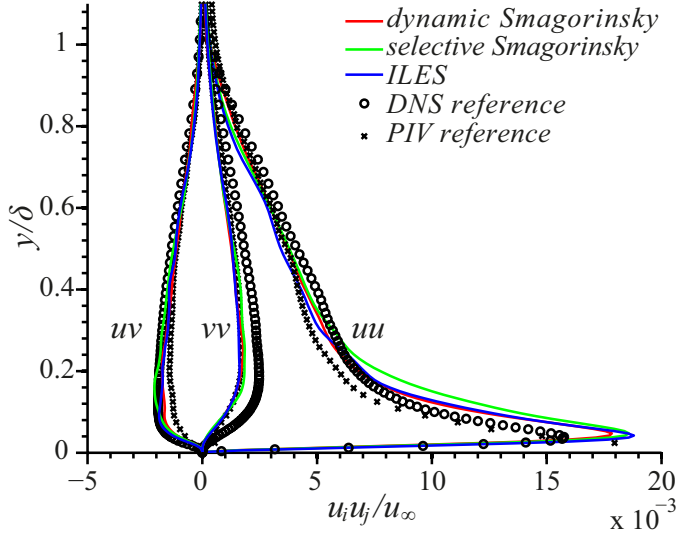
Figure 3.4: Reynolds stress profiles in outer scaling
