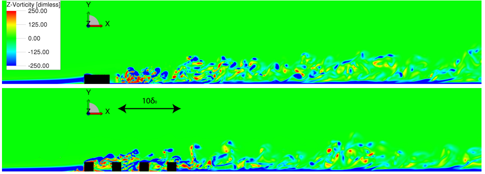
Figure 2.11: Instantaneous spanwise vorticity behind the zig-zag strip (top) and staggered grid of blocks (bottom) in a plane at mid-span
