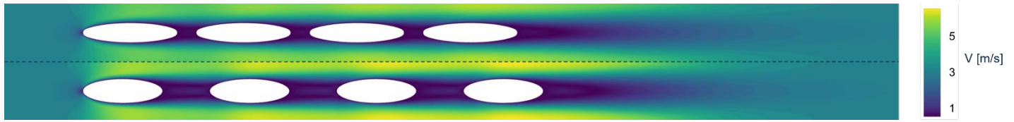
Figure 6: Velocity contours for the optimum design (top) and the baseline design (bottom).
