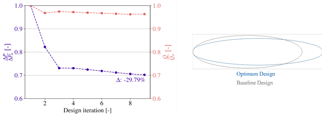
Figure 5: Optimization history depicting the evolution of the normalized objective function and constraint values (Left). Comparison of the optimum tube shape and the baseline design (Right).
