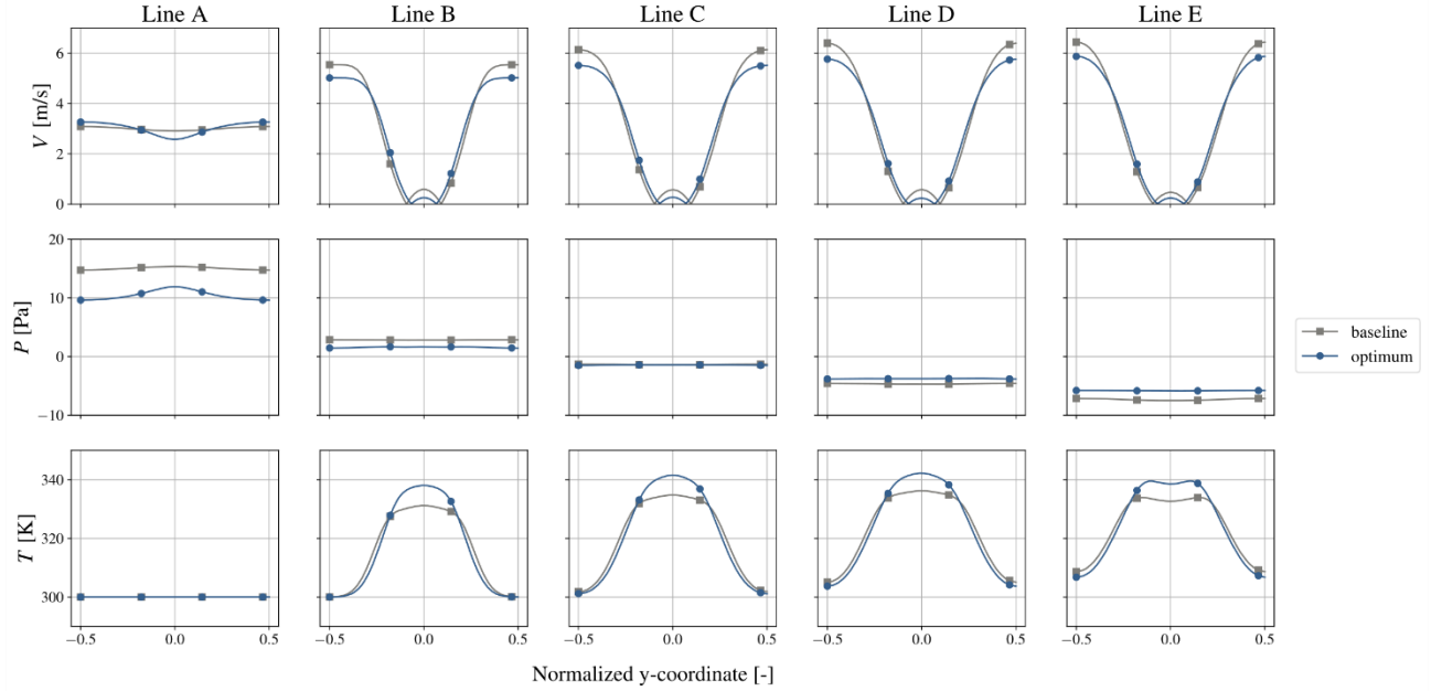
Figure 8: Comparison of the baseline and optimum designs with respect to the variation of flow properties – velocity magnitude, pressure, and temperature – as a function of the normalized y-coordinate at the locations A-E.
