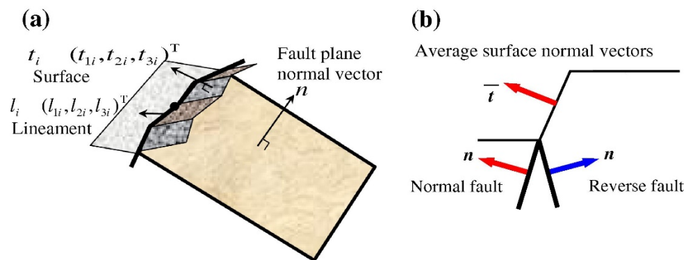
Figure A1. A schematic diagram of azimuth values, normal vectors, and fracture planes. (a) The azimuth of fracture plane; (b) The average surface normal vectors of fracture plane [57].
