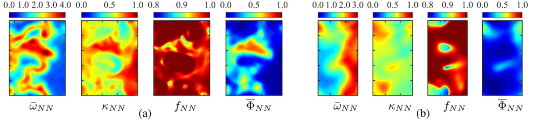
Fig. 8. Typical variations of \bar{\omega}_{NN} , \kappa_{NN} , f_{NN} and \bar{\Phi}_{NN} for B1 (a; \Delta/\delta_{th,nom} = 1.0 ) and BZ1 (b; \Delta/\delta_{th,nom} = 0.75 ).
