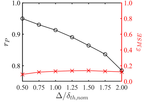
Fig. 10. Corresponding r_P ( \circ ) and \epsilon_{mse} ( \times ) of the \bar{\omega}_{c,NN}^{\delta z} field shown in Fig. 9 at different \Delta .
