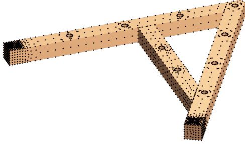
(a) FE-model
