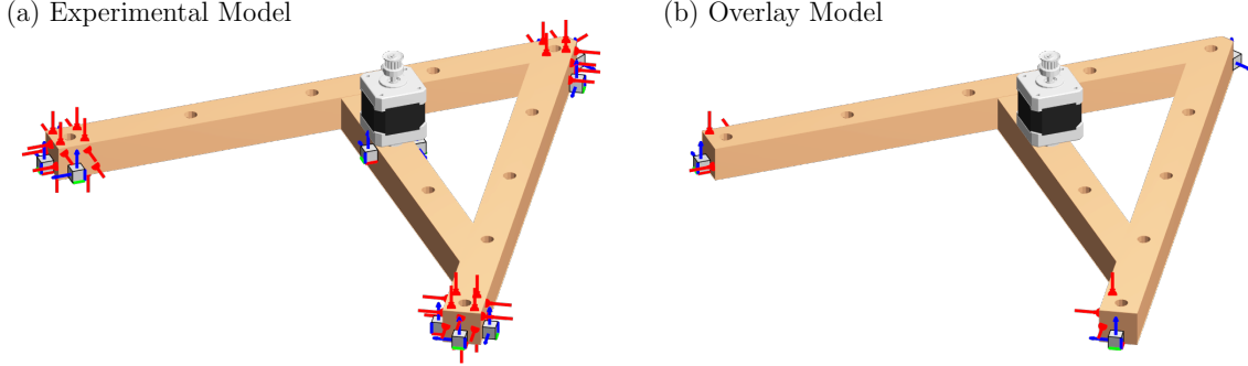
Figure 12: (a): The full experimental measurement sensor (blue) and impact (red) locations. (b): The subset of impact and sensor locations used for the overlay model. Note that the limited number of sensor and impact locations is insufficient for proper virtual point definition.
