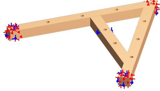
Figure 13: (a): The node locations of the FE model used to construct the numerical FRF model. (b): The DoF locations of the numerical FRF model used as the parent model in the SEMM process. Note that the stepper-motor is not included in the numerical FE-model.
