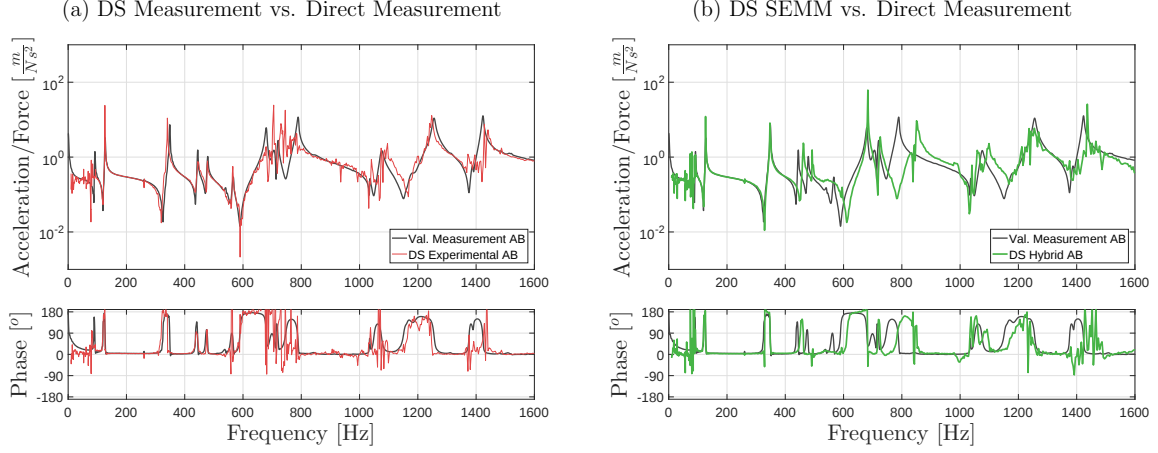
Figure 17: A driving-point FRF in the z -direction of the virtual node 3. Both the pure experimental DS model of AB (a) and the hybrid DS model (b) are compared to a reference measurement of the physical component AB.
