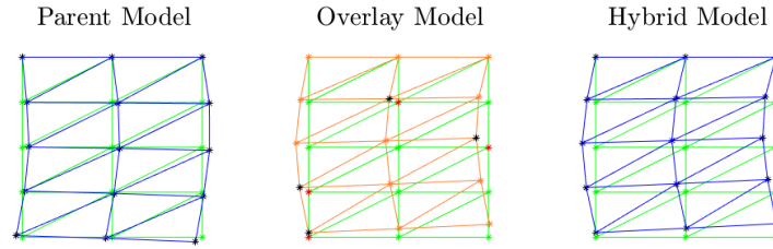
Figure 5: A truss construct actuated by a force at 420 Hz. Both a parent and overlay model exist and both predict different responses to the same load. Furthermore, the parent model (left) describes all nodes whereas the overlay model (centre) describes only a few, marked with a black star. SEMM is applied to create a model with the DoF of the parent model and provides the response of the overlay model.
