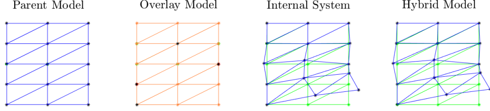
Figure 6: The response of the truss-system under a uniform harmonic load at 866 Hz. Both the parent (left) and overlay model (centre-left) barely respond. In contrast, The internal system of the parent model and therefore the residual \mathbf{Y}^{\text{res}} has its first mode at this frequency (centre-right). Consequently, the hybrid model (right) is sensitive to this actuation.
