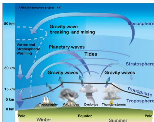
Figure 1: Schematic diagram of the atmospheric dynamic processes in the Earth's atmosphere. Reproduced from [12].
