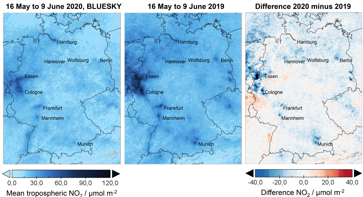
Fig. 8. Mean tropospheric NO 2 vertical column densities over Germany for (left) 2020 and (center) 2019 averaged over the BLUESKY period from 16 May to 9 Jun. The means were derived from Sentinel-5P/TROPOMI level 2 data. (right) The difference of 2020 minus 2019.
