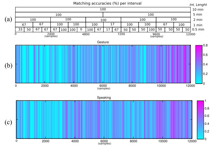
Fig. 11. Analysis of impact the impact of social actions in the association (better seen in color). (a) Matching accuracies for selected 6 participants under different length intervals at different times. (b) Normalized density of hand gestures for all participants (1 equals all participants gesturing). (c) Normalized density of speaking for all participants (1 equals all participants speaking).
