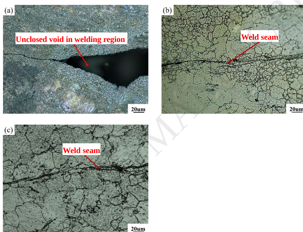
Fig. 20. Microstructures in welding zone D (R=12.5 mm) of the welded samples extruded at a speed of 0.8 mm/s and initial temperatures of (a) 300, (b) 350 and (c) 400 °C.
