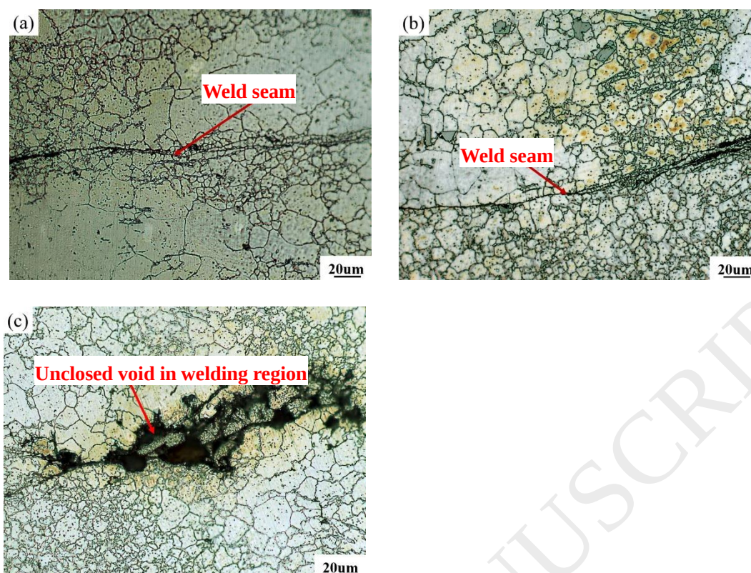
Fig. 19. Microstructures in welding zone D (R=12.5 mm) of welded samples extruded at an initial temperature of 350 °C and speeds of (a) 0.8, (b) 1.4 and (c) 2 mm/s.
