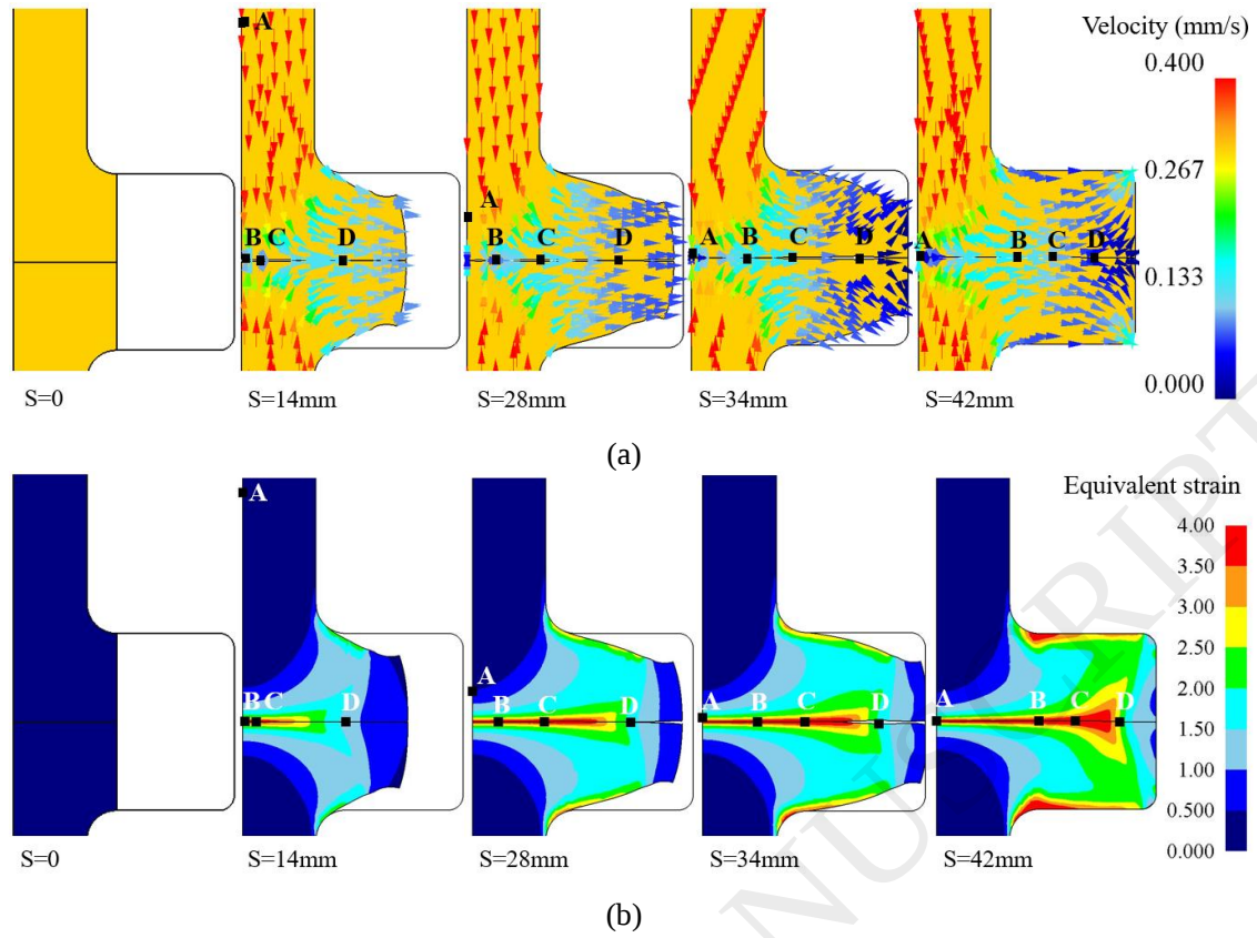
Fig. 7 FE simulated results of metal flow in the welding chamber when the extrusion temperature and speed were 350\text{ }^{\circ}\text{C} and 0.8\text{ mm/s} , respectively: (a) velocity fields and (b) equivalent strain fields.
