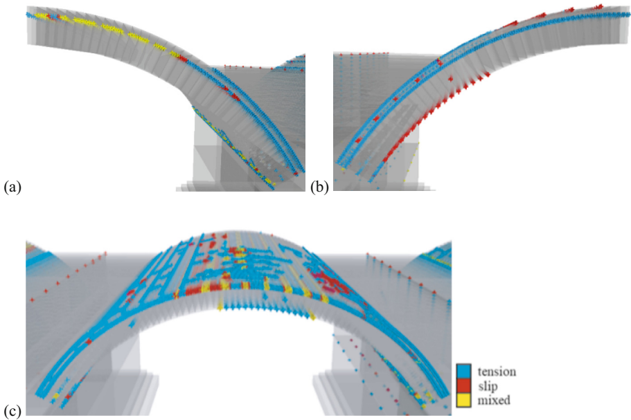
Fig. 10. Damage state of the wharf cellular under failure load condition at (a) left arch, (b) right arch, and (c) middle arch
