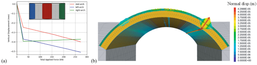
Fig. 9. (a) vertical displacement vs total applied force and (b) normal displacement vector at middle arch of the wharf cellular model
