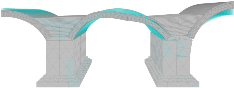
Fig. 12. Deformed shape of the wharf cellular model at failure load (magnified 10x)
