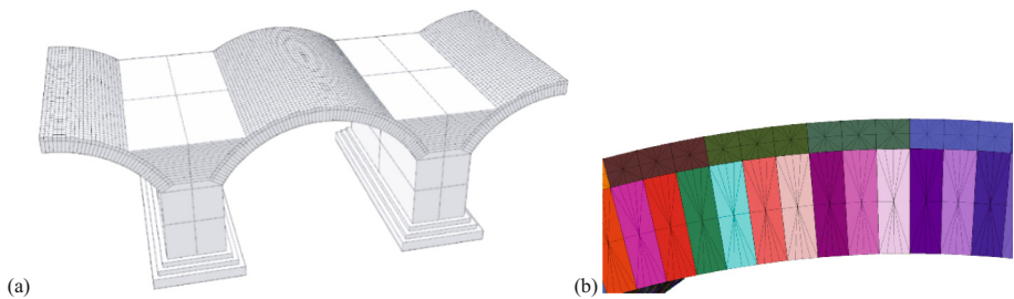
Fig. 5. (a) Isometric view of the Rhino 3D model of Utrecht Wharf Cellular and (b) stacking pattern at the arch section
