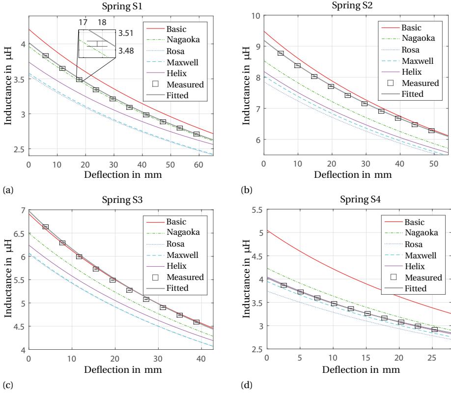
Figure 2.3: Experimentally determined deflection-inductance characteristics of the four springs, compared to predictions of the different theoretical models as well as a simplified model that is fitted to the data. The standard deviations of the measured inductances along the measurement profile of S1 lie between 0.0038 \mu\text{H} and 0.0060 \mu\text{H} , of S2 between 0.0023 \mu\text{H} and 0.0051 \mu\text{H} , of S3 between 0.0037 \mu\text{H} and 0.0055 \mu\text{H} and of S4 between 0.0034 \mu\text{H} and 0.0065 \mu\text{H} .
