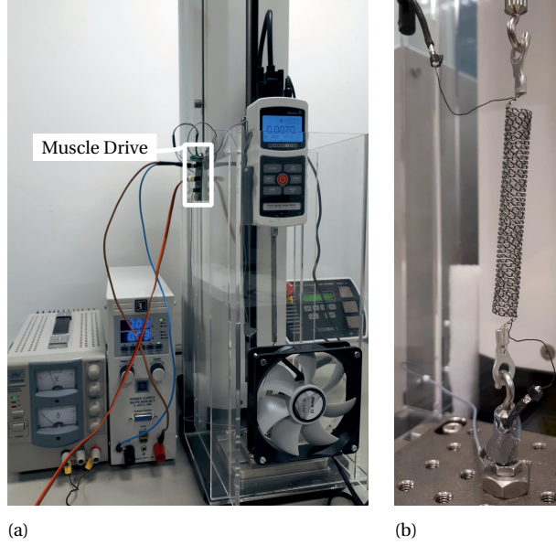
Figure 7.4: Overall setup, with the Universal Testing Machine and the Muscle Drive in (a) and the Twisted and Coiled Polymer Muscle in (b).
