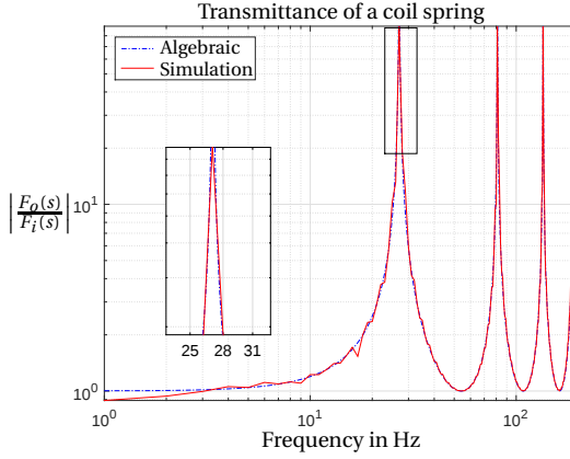
Figure 4.2: Comparison of the algebraically calculated transmittance (blue dash-dotted line) with the transmittance of the model (red solid line). Both represent the transmittance of coil spring S_T in Table 4.1.
