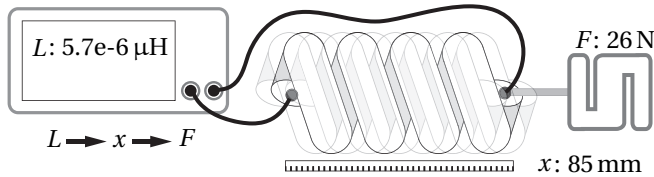
Figure 1.2: Chapter 4 investigates the influence of coil spring oscillations on three sensors, respectively measuring inductance L , deflection x and force F . This figure illustrates the sensors used. The gray box represents the inductance sensor, the ruler represents the deflection sensor and the S-shaped structure represents the force sensor. The numerical values represent a typical data point measured by the respective sensors.
