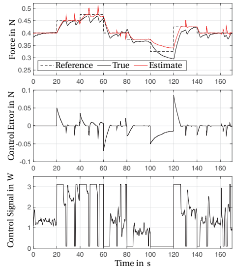
(b) Step response during force control.
