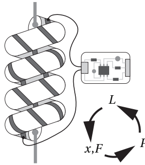
Figure 1.4: Chapter 7 contains an implementation of self-sensing and closed-loop control of a Twisted and Coiled Polymer Muscle using self-sensing. The self-sensing implementation is based on the applied power P and the measured inductance L . It enables closed-loop control of both deflection x and force F . The illustration shows closed-loop control of the muscle's deflection under a constant force, represented by the weight and its position, performed by the custom hardware, represented by the printed circuit board.
