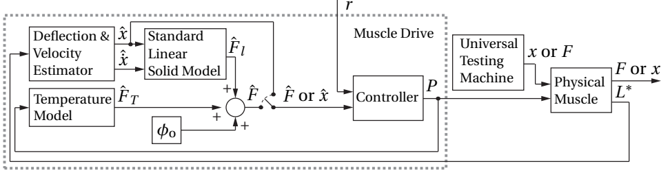
Figure 7.2: Block diagram for estimation and control. The gray dashed rectangle contains the functionality of the Muscle Drive (MD). Within the MD, the switch indicates that either the deflection estimate \hat{x} or the force estimate \hat{F} is used as input for the controller, alongside reference r , resulting in either control of deflection x or force F . The Universal Testing Machine (UTM) acts as a load on the muscle. When the MD controls force, the UTM imposes deflection, and vice versa. The temperature model uses power input P to compute the contribution of temperature to force \hat{F}_T , as in (7.1). The deflection and velocity estimator represents the measurement of deflection based on decay time L^* in (7.4), the subsequent low-pass filtering of the deflection measurement, and taking the backward difference to find velocity \dot{\hat{x}} . The Standard Linear Solid model calculates the contribution \hat{F}_l to force by deflection and velocity using (7.6). The total force estimate \hat{F} is found by adding \hat{F}_l , \hat{F}_T and force offset \phi_o . Finally, the PID controller with anti-windup determines the control signal by using (7.7).
