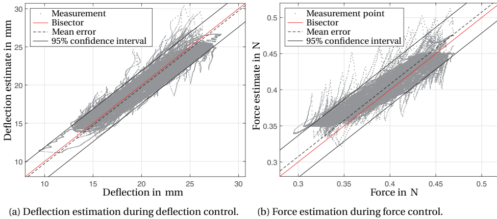
Figure 7.6: Estimation data during respectively deflection control (a) and force control (b). The gray dots and effectively gray areas represent the estimates given at the true value. The red line represents bisector of the graph, indicating what the correct values would be. The area between the black lines indicates the 95% confidence interval, which is \pm 2.14 mm around a mean error of -0.27 mm for deflection, and \pm 29.0 mN around a mean error of 7.5 mN for force.
