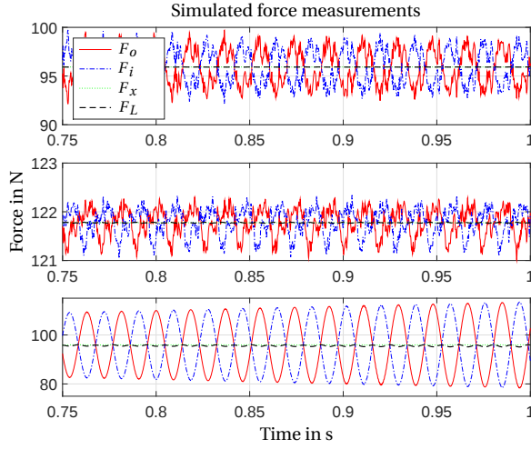
Figure 4.4: Simulated force measurements for three excitation cases. The three subplots respectively contain the heel strike, the end-stop collision when extending and the excitation at the first Eigenfrequency. The red solid lines are the output forces F_o as in (4.7), the blue dash-dotted lines are the input forces F_i as in (4.7), the green dotted lines are the measured forces via direct position data F_x , and the black dashed lines are the measured forces via inductance data F_L .
