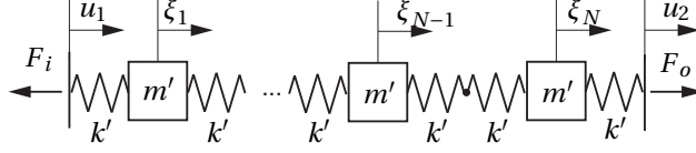
Figure 4.1: N^{th} -dimensional mass-spring model of a coil spring, with inputs u_1 and u_2 , positions \xi_1 to \xi_N . The individual masses m' are found by m/N and the individual stiffnesses k' are found by 2Nk .
