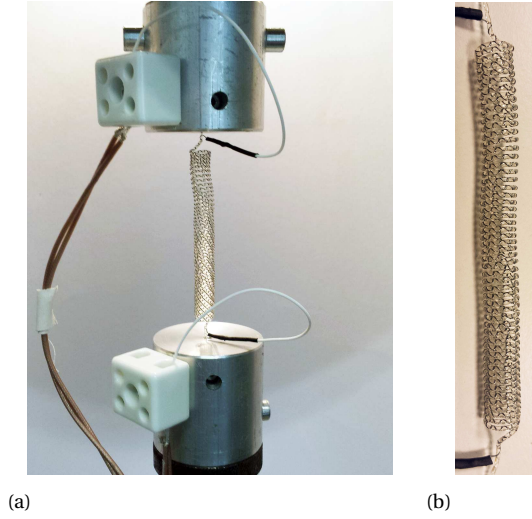
Figure 6.2: Illustration of the measurement setup. Figure 6.2a shows the TCPM in the UTM with four-point measuring cables attached, leading to the LCR43100. Figure 6.2b shows a close-up of the TCPM.
