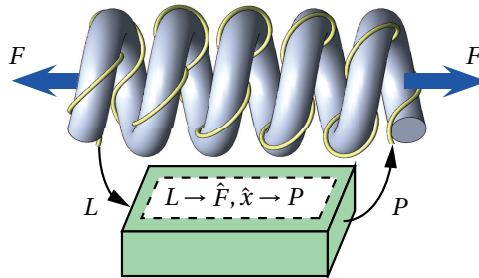
Figure 7.1: Impression of a self-sensing muscle. A control signal P is used to both drive the muscle to generate the force F and measure the inductance L of the Joule-heating wire. Based on the measurement and the previous control input, the self-sensing and control module estimates the force \hat{F} and deflection \hat{x} , and subsequently determines the new control signal.
