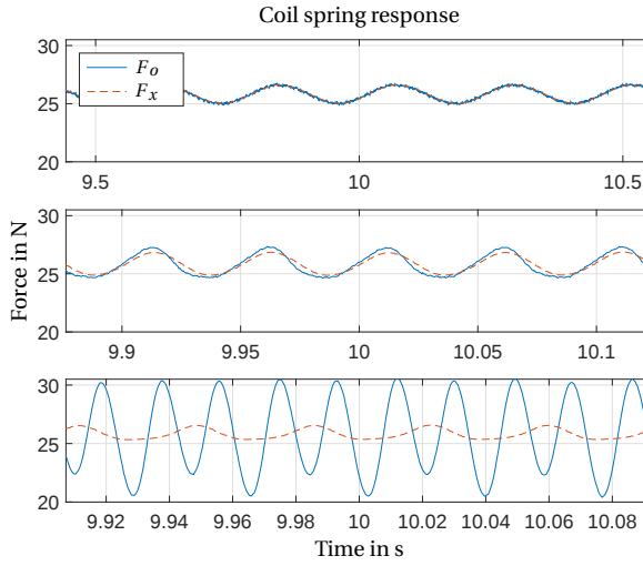
Figure 4.5: Raw force measurements from a load cell and a laser distance meter, for three excitations: 4.5, 20.2 and 27.0 Hz.
