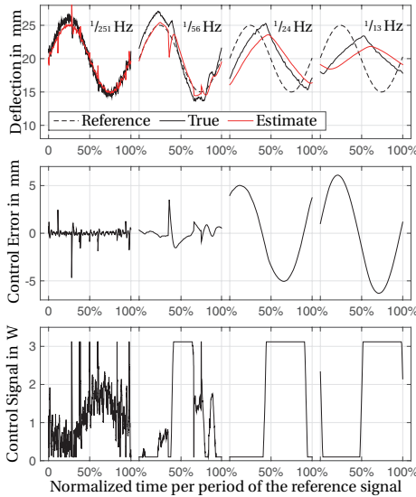
(c) Sine sweep during deflection control.
