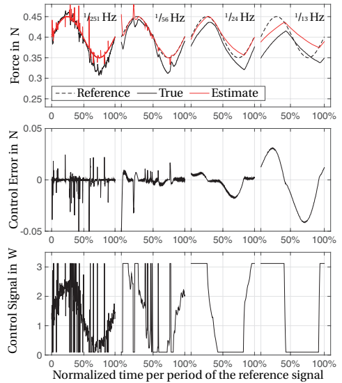
(d) Sine sweep during force control.
