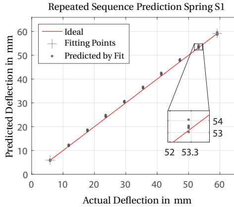
Figure 2.4: The measured versus predicted deflection of spring S1 for five sequences, according to the fit of sequence S1-a. The standard deviations across the sequences lie between 0.16 mm and 0.38 mm.
