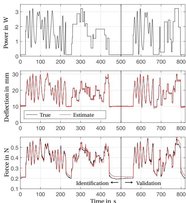
Figure 7.5: Time series of the identification and validation. The top figure shows the applied power. The middle figure shows the applied deflection in black, and the fit deflection estimate in red. The bottom figure shows the measured force in black and the fit force in red. In all figures, the black vertical line shows the separation of identification and validation data.
