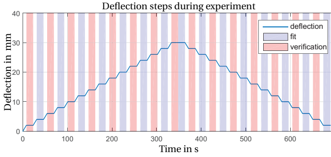
Figure 6.3: The deflection steps taken during the experiment for one reference temperature, once the heating chamber had reached that temperature. The blue and red ribbons indicate which data was used for respectively fitting and verification.
