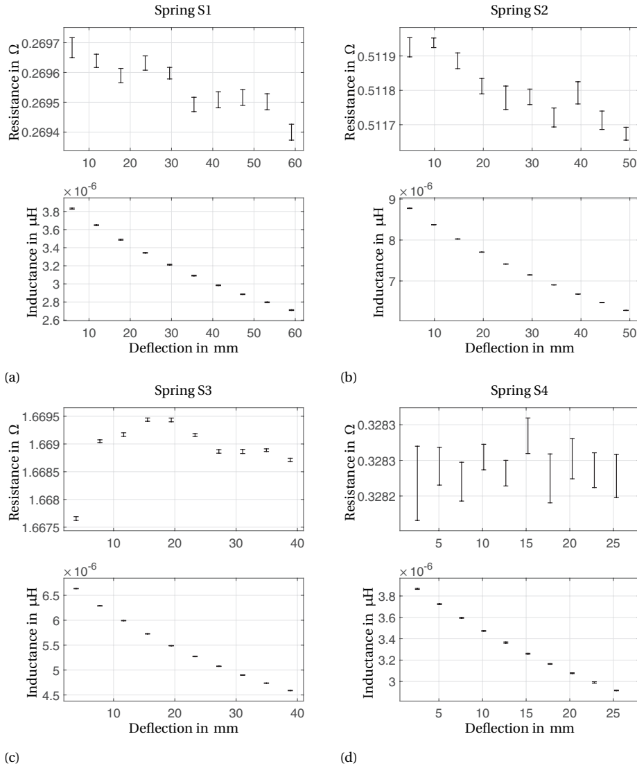
Figure 3.1: Data demonstrating the sensitivity of respectively resistance and inductance to deflection of four coil springs. The errorbars indicate the mean and standard deviation of ten measurements taken at each deflection.
