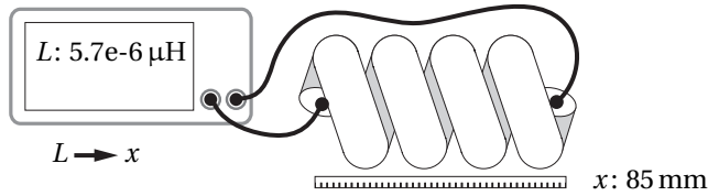
Figure 1.1: Chapter 2 characterizes the relation between inductance L and deflection x of coil springs. This figure conceptually illustrates the performed experiment. The gray box represents the inductance sensor, and the ruler represents the deflection sensor. The numerical values represent a typical data point measured by the respective sensors.
