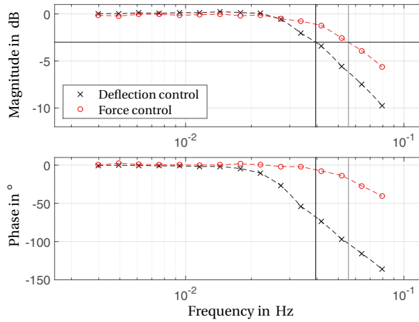
Figure 7.8: Frequency response data of the sine sweeps, with deflection control in black, and force control in red. The cross markers indicate the measured response. The dashed lines indicate the linear interpolation between these points. This shows that the -3 dB point for deflection control lies at approximately 0.039 Hz, and for force control approximately at 0.056 Hz.
