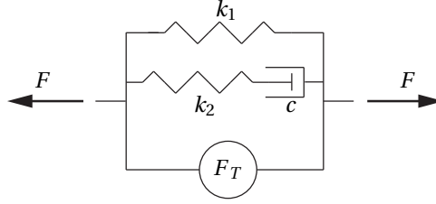
Figure 7.3: Representation of the force model used for the muscles: the Standard Linear Solid model [120], with a contribution by temperature in parallel.
