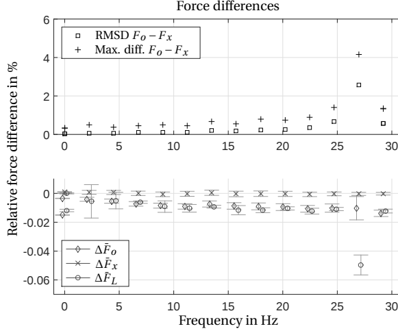
Figure 4.6: Relative force measurement performance from a LC F_o , LDM F_x and an inductance meter F_L . The first subplot indicates the difference over time between the LC and the LDM, in the form of the RMSD and the maximum difference. The second subplot gives the relative averaged force measurements \Delta\bar{F}_o , \Delta\bar{F}_x and \Delta\bar{F}_L .
