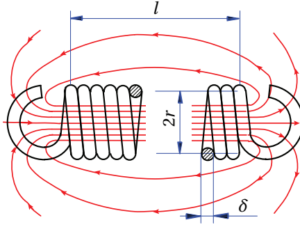
Figure 2.1: Spring of length l , coil radius r , and wire diameter \delta , and magnetic field when a current is applied.
