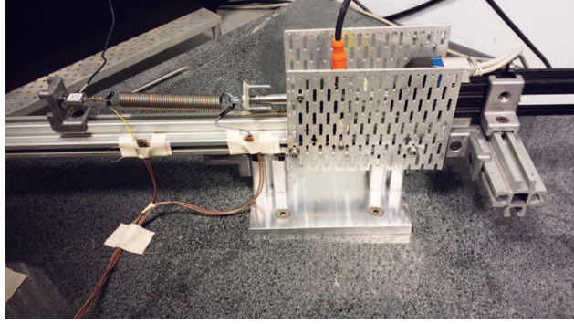
Figure 4.3: The experimental setup: The spring is mounted between a linear actuator and a force sensor. It is also connected to an inductance meter, and a laser distance sensor measures deflection. The motor imposes harmonic oscillations at a range of frequencies, including the spring's first resonance.
