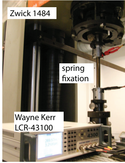
Figure 2.2: Measurement setup, with the Zwick 1484 applying and measuring displacement between the spring fixations, and the Wayne Kerr LCR-43100 measuring inductance of the spring.
