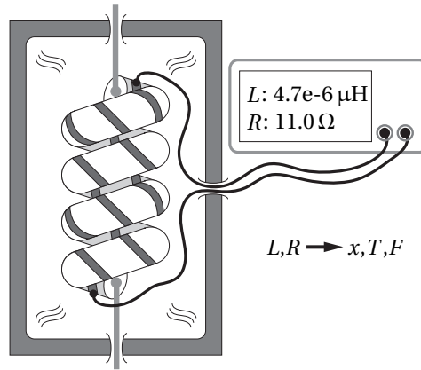
Figure 1.3: Chapter 6 contains a characterization of the relation between inductance L and resistance R , and the thermo-mechanical state of a Joule-heated Twisted and Coiled Polymer Muscle consisting of deflection x , temperature T and force F . This figure illustrates the muscle suspended inside a testing machine with climate chamber, represented by the dark gray box, to apply and measure temperature, deflection and force. The light gray box measures the electrical impedance of the muscle's Joule heating. The numerical values represent a typical data point measured by the respective sensors.
