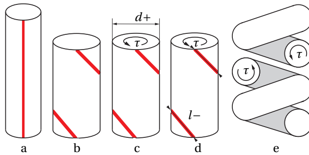
Figure 5.1: The working principle of twisted and coiled actuators. Subfigure (a) shows the precursor fiber, with the red line indicating the alignment of the polymer chains. Subfigure (b) shows the twisted fiber after annealing, so the fiber retains its shape. In this figure the polymer chains have obtained a helical orientation. Subfigures (c) and (d) respectively show the torque that results from increasing fiber diameter and from entropic contraction of the polymer chains. Subfigure (e) illustrates that a (homochiral) coil of twisted fiber contracts when heated.
