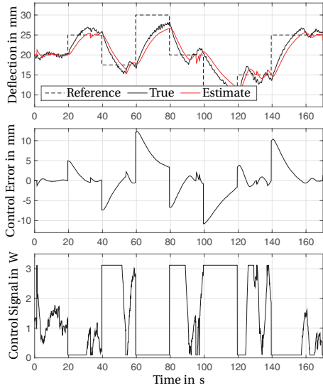
(a) Step response during deflection control.
