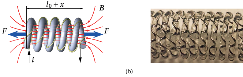
Figure 6.1: Electromechanical model of a Joule-heated TCPM (Figure 6.1a), and a close-up of an actual TCPM (Figure 6.1b). A metal wire wrapped around a polymer helix is the conductor for Joule heating. The muscle contracts when heated and has a substantial mechanical stiffness, so a force F results from a temperature change or a deflection x . The metal wire has an inductance, so a magnetic flux B results from a change in current i through the wire. The wire's resistance changes with temperature. Therefore, the electrical impedance of the muscle provides information on the mechanical state.
