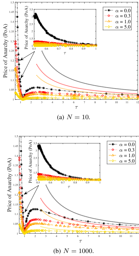
Fig. 2: The Price of Anarchy (PoA). The dotted lines represent the bound from Corollary 2.
