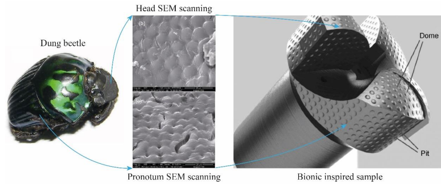
Figure 1.6 Bionic drill bit inspired by dung beetle, based on [14]
