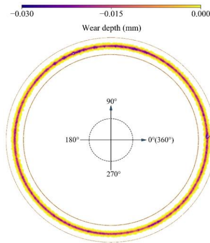
Figure 5.17 Wear profile
