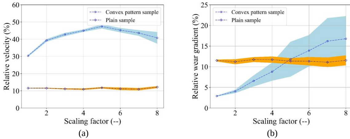
Figure 4.13 Comparison of the relative velocity and wear rate (a) relative velocity, (b) relative wear rate
