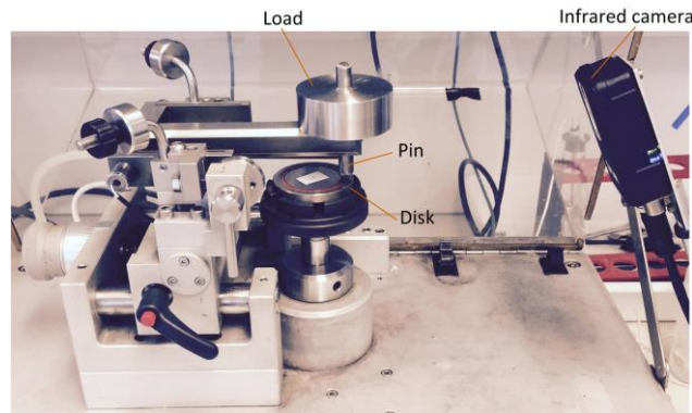
Figure 5.3 Pin-on-disc apparatus [194]
