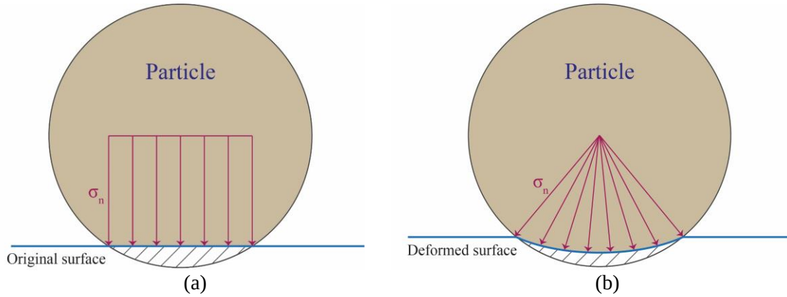
Figure 5.16 Illustration of stress over disc (a) original surface, (b) deformed surface
