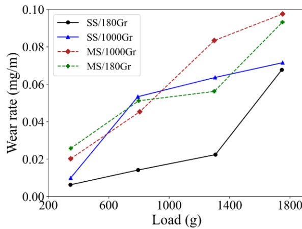
Figure 2.19 Wear rate against applied load for three-body abrasion wear, based on [57]
