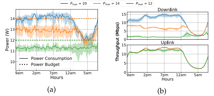
Fig. 13. Performance evaluation of SBP-vRAN throughout one day.
