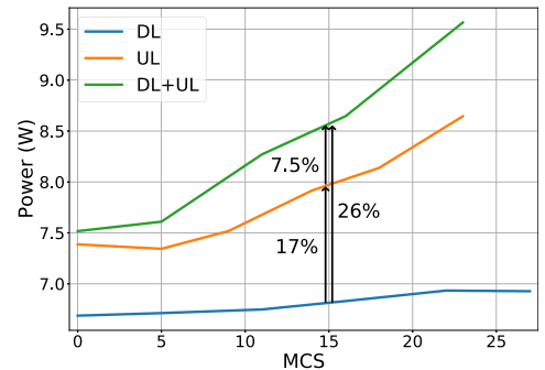
Fig. 4. MCS impact on BBU power consumption with high SNR. Results presented for three cases: only DL traffic being processed; only UL traffic; concurrent DL and UL traffic.
