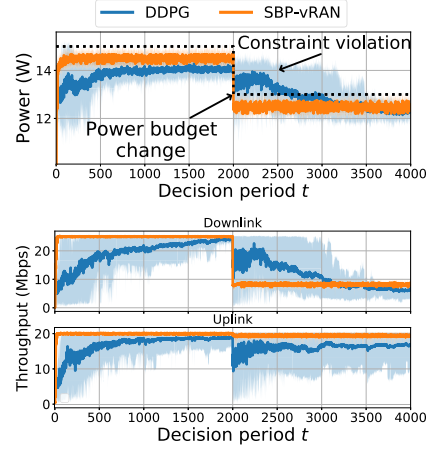
Fig. 15. Comparison of SBP-vRAN with the customized DDPG.
