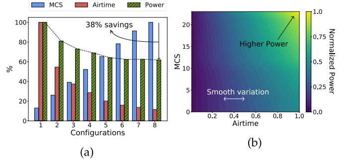
Fig. 3. (a): Eight configurations of MCS and airtime that offer 2.6Mbps in UL, and the respective power (idle mode's power subtracted). (b): Normalized BBU power consumption over baseline, for full buffer UL transmissions and high SNR values, as a function of MCS and airtime.
