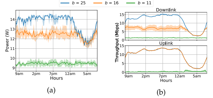
Fig. 12. Performance evaluation of BP-vRAN throughout one day.
