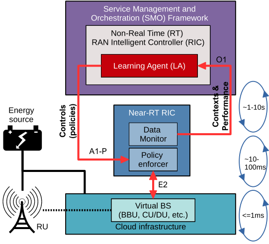
Fig. 5. O-RAN compliant system architecture and workflow.
