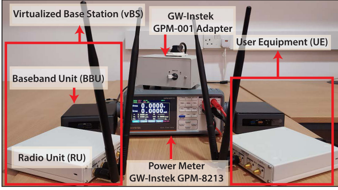
Fig. 7. Customized Wireless Testbed with a vBS (srsRAN) and a node aggregating the UE traffic. Measurements are collected in real time, using a GW-Instek Power Meter and a Power Adapter.
