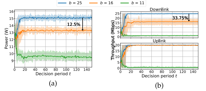
Fig. 8. Convergence rate evaluation of BP-vRAN for different objective function parameters.
