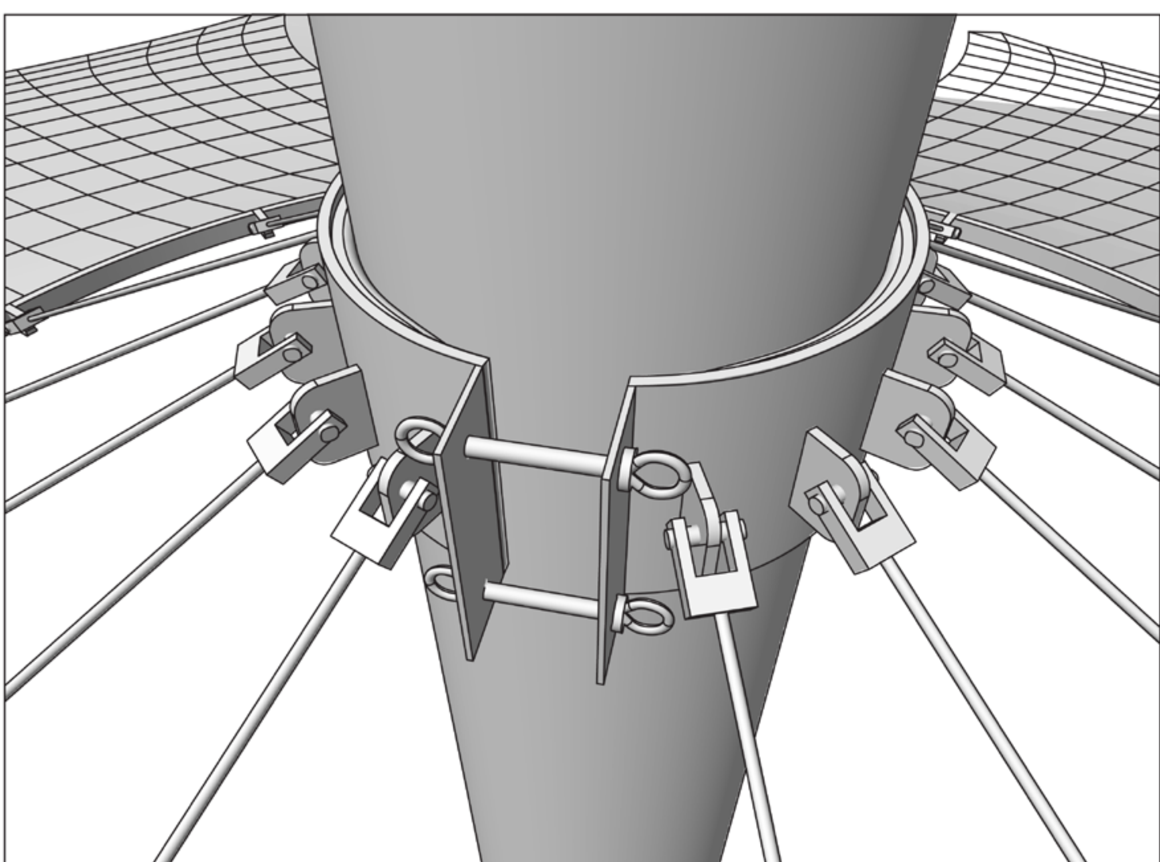
De Theatertent | Detail F | 1:200
