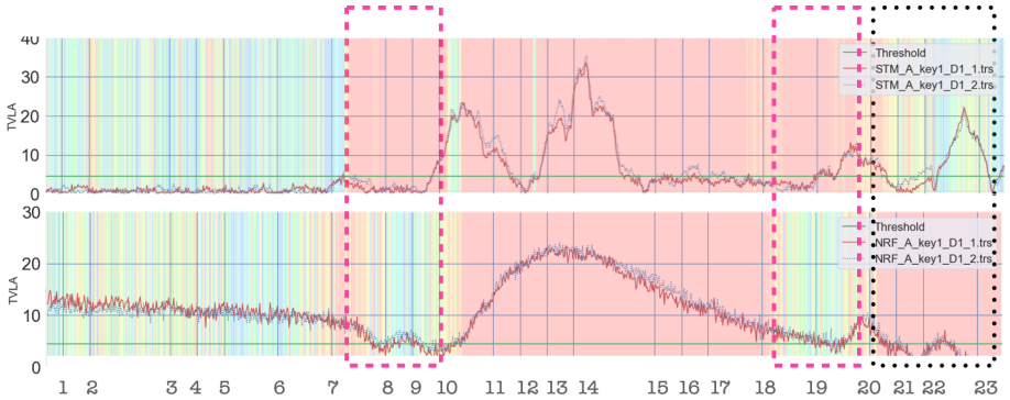
Fig. 12. (To be viewed in colors.) Overlay of the key rank estimate on the TVLA results for STM_A device (top) and NRF_A device (bottom). Red regions represent the index locations where the correct key is ranked first. The rectangles highlight differences in leakage between the two boards. The numbers on the x-axis are the instruction being executed, see Listing 1.1.
