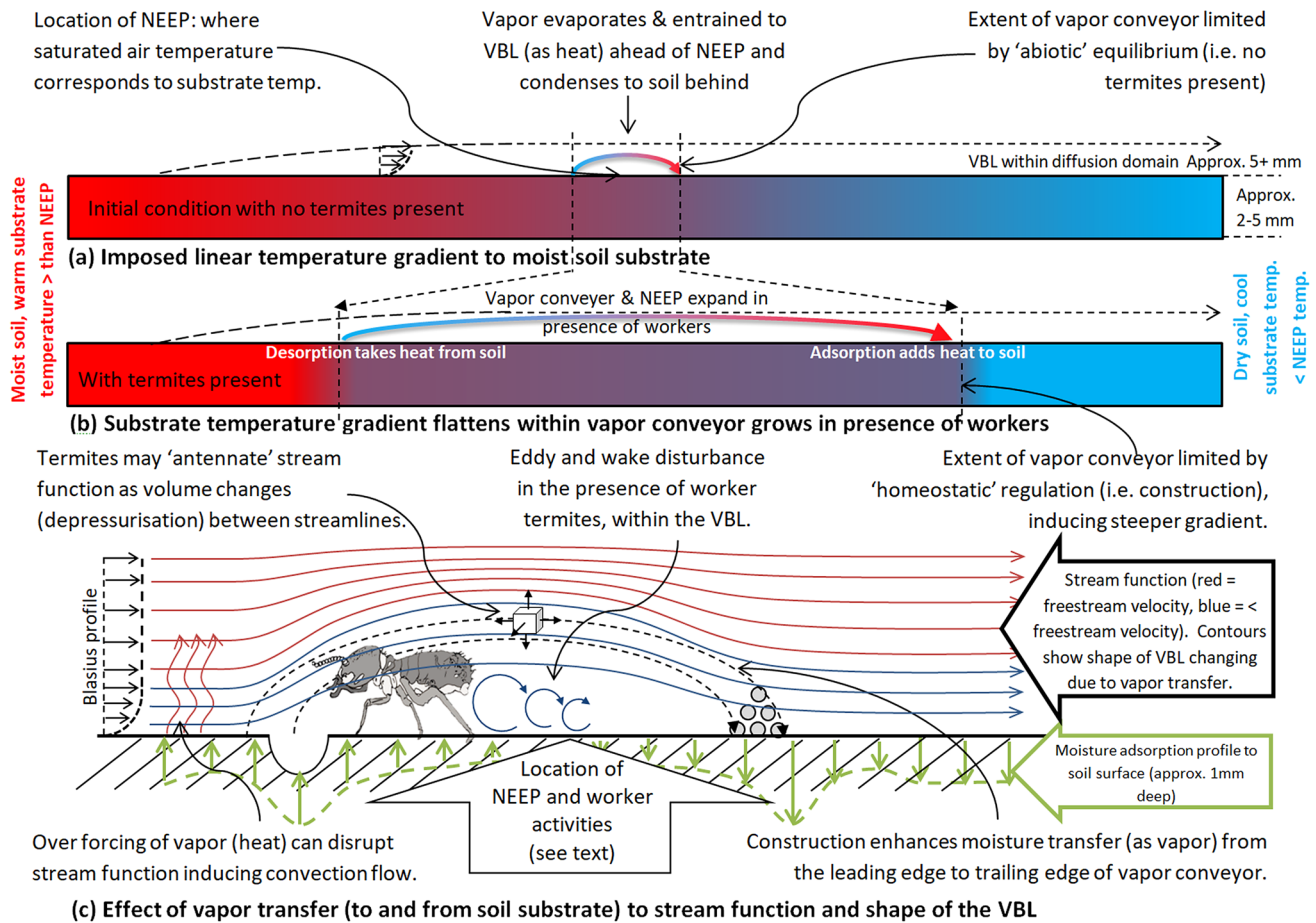
Fig. 1 a 'Vapor conveyor' emerges at the soil/air interface, either side of a neutral evaporative equilibrium point (NEEP) due to the presence of (i) temperature gradient, (ii) moist soil substrate and (iii) diffusion limited viscous boundary layer. It expands around the NEEP and its extents are limited by 'abiotic equilibrium' (vertical dashed line). b Workers sense the vapor conveyor as it is coupled to soil moisture and
