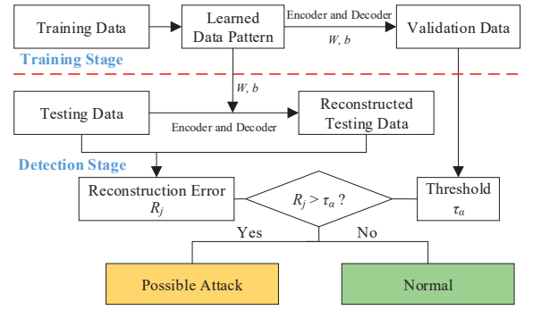
Fig. 2. The proposed training and FDIA detection mechanism.
