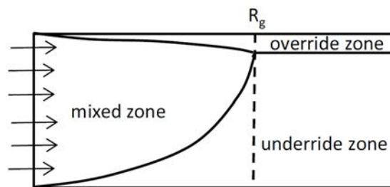
Figure 1—Schematic of gravity-segregation model of Stone (1982)
