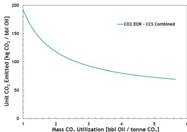
Figure 2—CO 2 intensity of oil production (including its burning in later application e.g. in a power plant) for a CO 2 EOR process combined with CCS, as a function of mass CO 2 utilization factor (reproduced from Farajzadeh et al. 2020).
