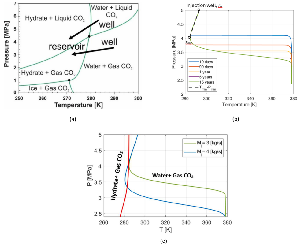
Fig. 2. (a) Pressure-Temperature phase diagram of water-CO 2 binary system, reproduced from Voronov et al. (2016) , (b) (P,T) diagram based on our model. (c) Mass injection rate effect on a (P,T) diagram, at time t_D = 1 .
