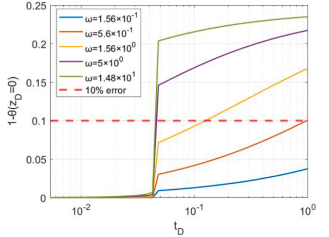
Fig. 9. Newton's law criterion vs. time, for different \omega values. Plotted for x_D=4\text{E-}5 .
