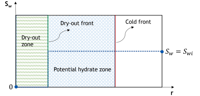
Fig. 6. Formation of a region with a non-zero water saturation between dry-out and cold fronts.
