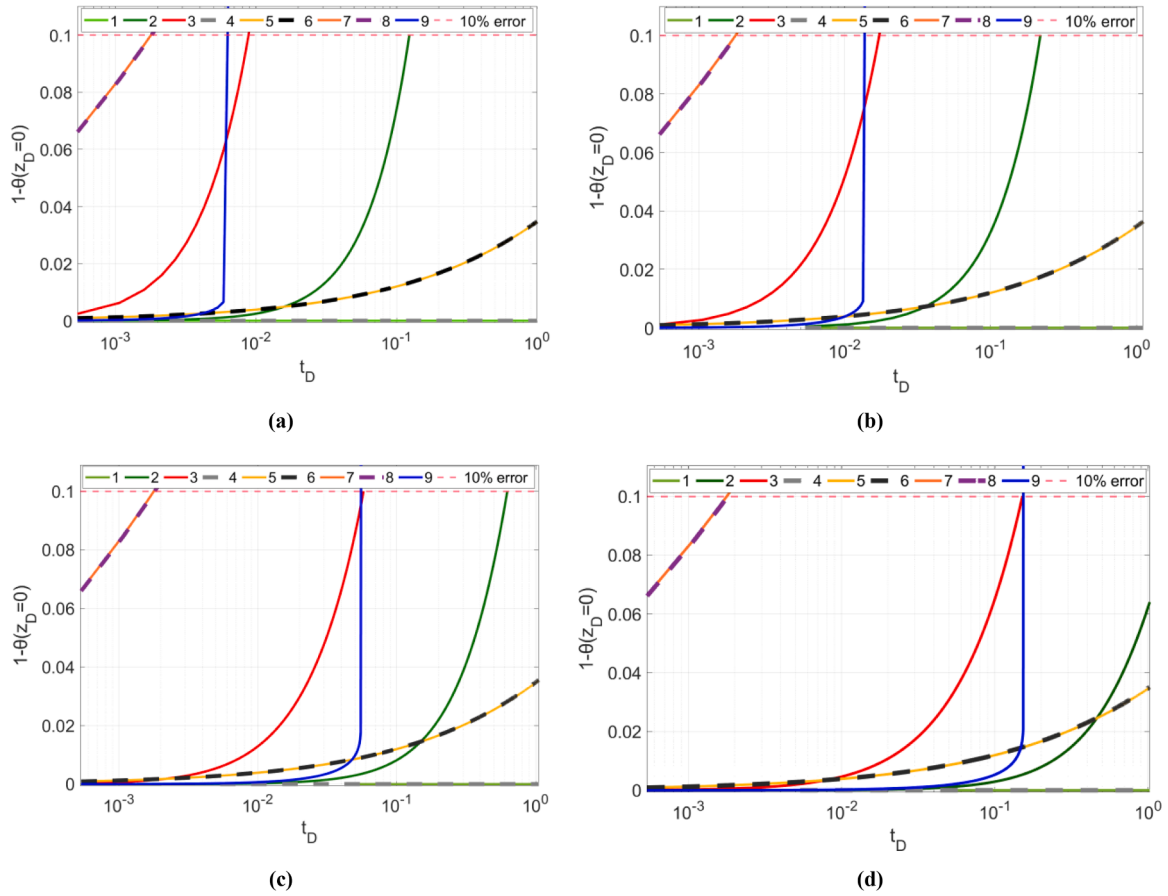
Fig. 10. Difference between temperature at the outer bounds of shale and initial reservoir temperature, to validate Newton's law, temperature history at the distance from injectors at (a) x_D = 2.5E-6 , (b) x_D = 5.6E-6 , (c) x_D = 2.25E-5 , (d) x_D = 6.3E-5 .
