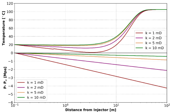
Fig. 14. The impact of permeability on the temperature profiles.
